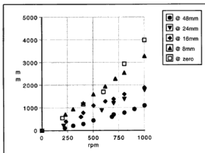
Figure 5 Variation of Distance from Disc to Magnet
