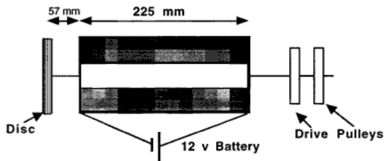
Figure 2 Solenoid Apparatus
