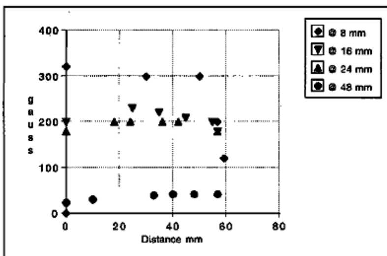
Figure 6 Magnet Field Readings
