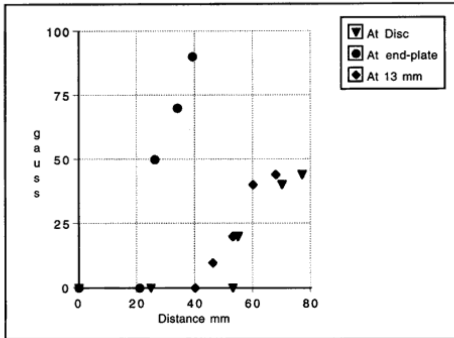
Figure 7 Solenoid Field Readings
