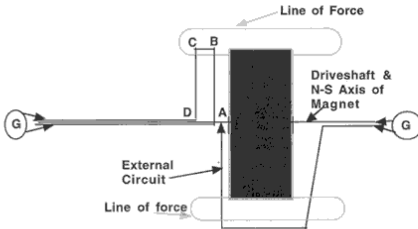
Figure 9 Circuit Cut Twice by Lines
