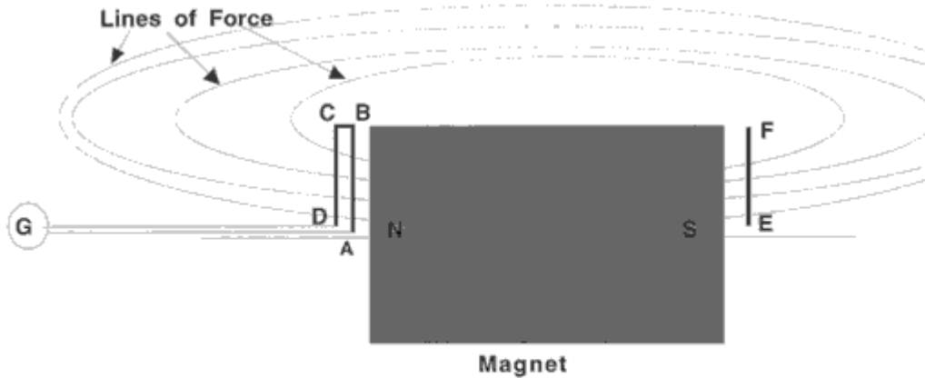
Figure 8 Effect Produced on a Conductor near a Magnet
