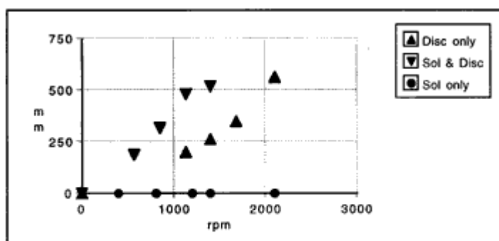
Figure 4 Solenoid Tests
