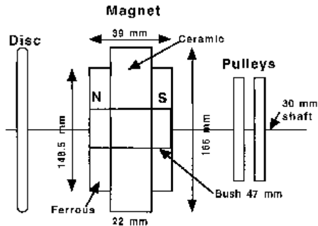
Figure 1 Magnet Apparatus
