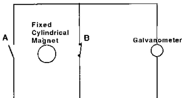
Figure 13 Tilley Test
