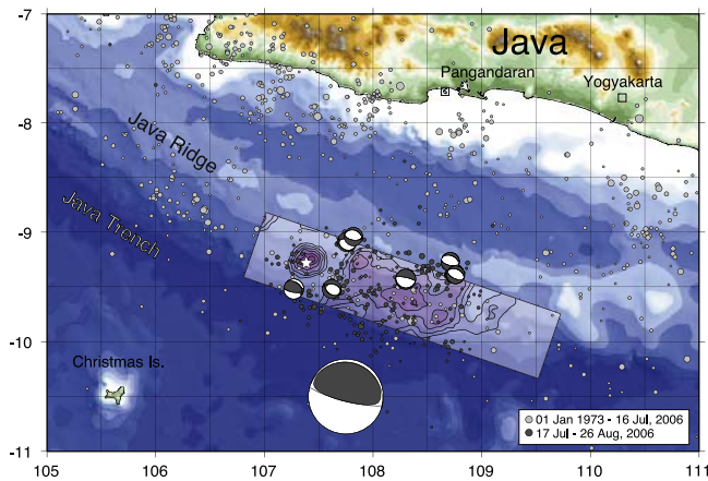
Figure 1. Map showing the Global CMT solutions for the 17 July 2006 Java tsunami earthquake and aftershocks and the NEIC epicenters of mainshock (star), aftershocks (dark circles), and prior activity (gray circles). The mainshock CMT solution is centered near the centroid location, which has a bias toward the southwest; other CMTs are at the NEIC locations. The preferred slip model found in this paper is contoured (scale is shown in Figure 4).
