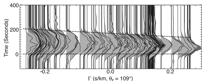
Figure 2. Rayleigh wave STFs for the 17 July 2006 Java earthquake plotted as a function of directivity parameter, \Gamma , assuming a rupture propagating at an azimuth of \text{N}109^\circ\text{E} . STFs corresponding to rupture towards the station are located on the right, those in a direction away from rupture are on the left. The time functions systematically decrease in width from 200 s to 100 s as \Gamma increases from left to right, as indicated by the dotted lines.
