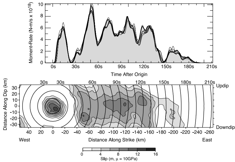
Figure 4. (top) Moment rate functions estimated from 6 finite fault inversions with rupture speeds of 1.00, 1.25, and 1.50 km/s and with and without SH waveforms. The moment-rate function is the perhaps best-constrained quantity from this type of inversion. The thicker line and shading highlight the moment-rate function from the model above. (bottom) Finite-fault inversion results for an assumed rupture speed of 1.25 km/s. The peak moment in the 5 km x 5 km cells is 0.34 \times 10^{20} N-m and the total moment is 7.0 \times 10^{20} N-m, ( M_w = 7.8 ). The hypocenter location is (0, 0), the top of the fault is one km beneath the trench. Rupture front isochrons are shown at 10 s intervals (top axis); the left and bottom axes show distance from the focus in km. Slip is scaled from moment using \mu = 10 GPa.
