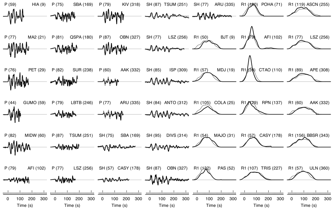
Figure 5. Observations and predictions from 16 P waveforms, 9 SH waveforms, and 17 R1 STF's used in the finite fault inversion with a rupture velocity of 1.25 km/s shown in Figure 4. Wave type and distance ( ^\circ ) are shown above and to the left of each waveform, the station name and azimuth ( ^\circ ) are shown to the right. Body waves are cut to exclude PP or SS arrivals, but no effort is made to account for core reflections. The observations are shown with a thicker black line, the predictions with the thinner gray. Observed peak STF amplitudes in the AFI and CTAO are high (as indicated by their seismic moments) because their azimuths are near a radiation node and they are sensitive to the assumed faulting geometry.
