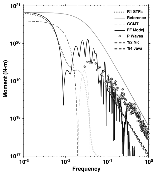
Figure 3. Spectrum of the moment rate function from the finite fault inversion (FF), the average R1 STF amplitude spectrum, the Global CMT assumed time function spectrum, and average values for the P wave spectrum computed using the method of Polet and Kanamori [2000]. The R1 and GCMT spectra are light gray where they are extrapolated to short periods. An average \omega -squared source spectrum with typical corner frequency is shown for reference. The average P wave spectra for the 1992 Nicaragua and 1994 Java tsunami earthquakes are also shown.
