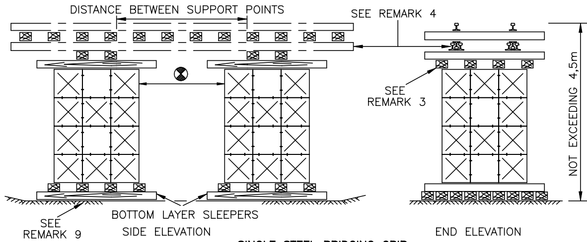
SINGLE STEEL BRIDGING CRIB (SEE NOTE 5)
