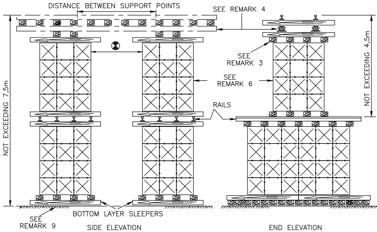
DOUBLE STEEL BRIDGING CRIB
