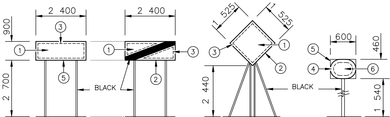
WARNING BOARD
