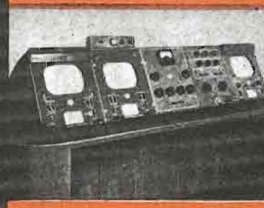
Similar setup with two camera control units (one live and one film, or two film), such as used in the RCA "Busta Boy" Fox TV.
