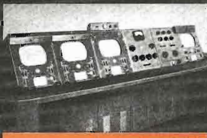
TC-4A with master monitor unit, preview monitor unit and two camera control units (one live and one film, or two film). If desired sections can be arranged U-shape or L-shape to fit available space.
