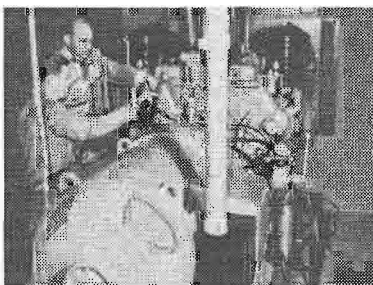
WJR—Detroit, Michigan, uses 200 kw. GM Diesel generator set as stand-by power for 50,000-watt transmitter. Compactness of unit permitted installation in garage adjoining transmitter building—eliminating cost of a specially designed building.
