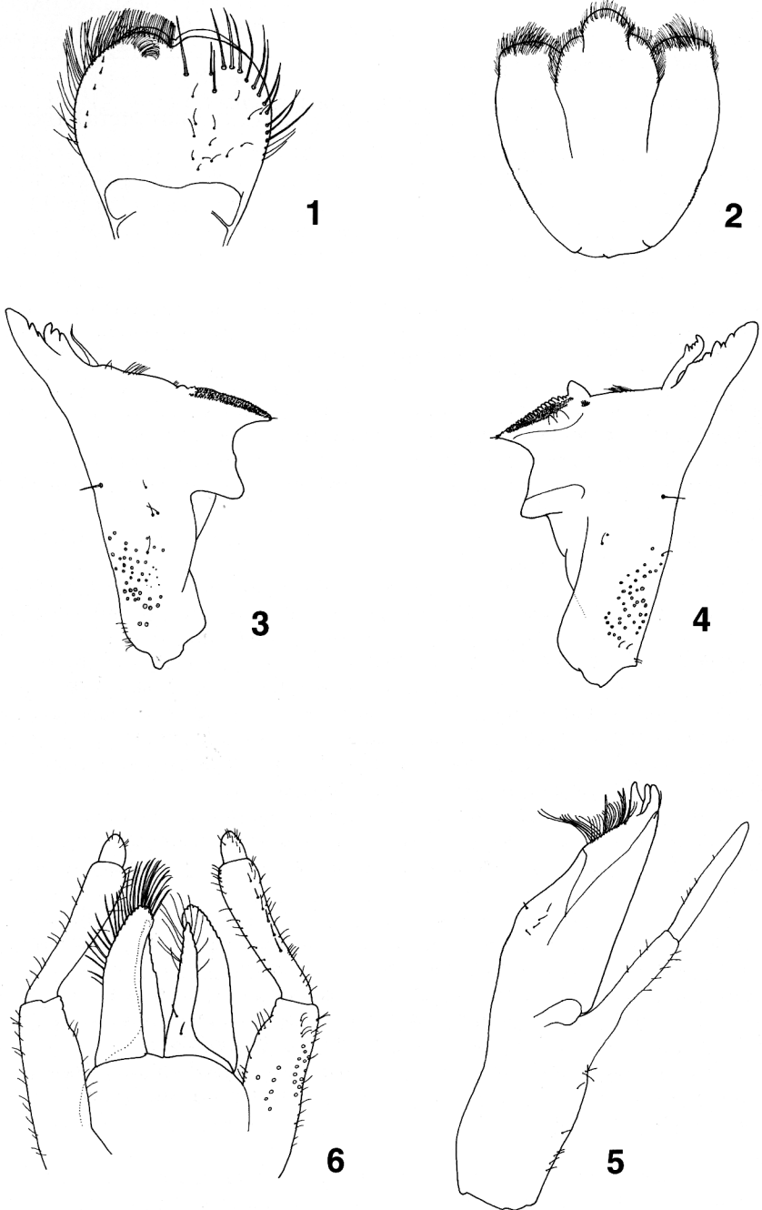
Figs 1–6: Larval structures of A. spinosum . 1: labrum (left: ventral; right: dorsal); 2: hypopharynx; 3: right mandible; 4: left mandible; 5: left maxilla; 6: labium.
