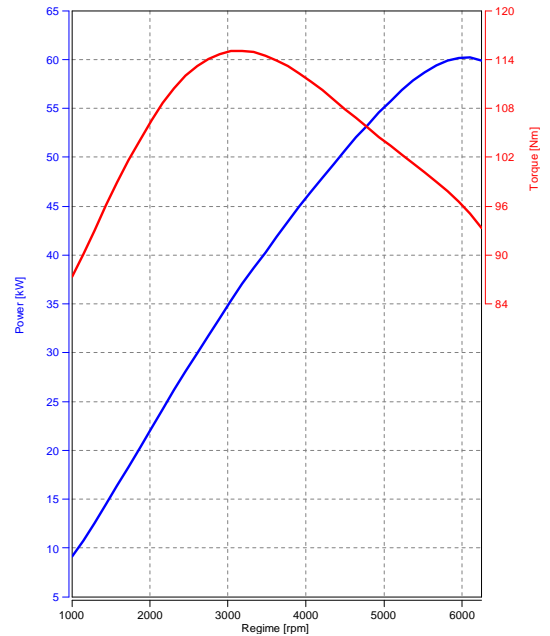
Performances curves
