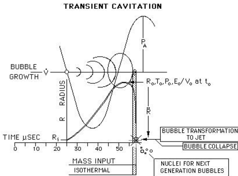
Figure 21 Transient Cavitation Bubble Diagram
