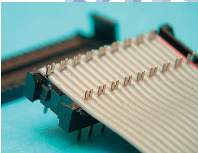
A closeup of an 18-pin IDC header plug which has had the main clamping strip removed again, to show the jaws passing through the cable. Note the two rows, for alternate wires.
