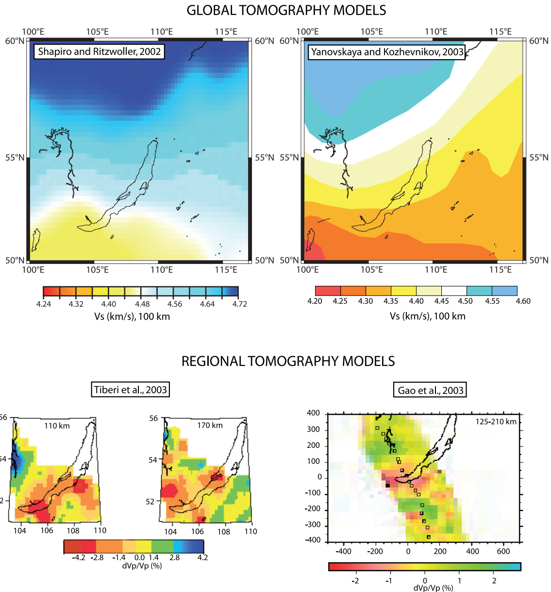
Figure 9. Comparison of tomographic models over the BRS. (top) S-wave velocity at 100 km from Rayleigh wave tomography, redrawn after Shapiro and Ritzwoller [2002] (left) and Yanovskaya and Kozhevnikov [2003] (right). (bottom) P wave velocity around 150 km from local tomography models, redrawn after Tiberi et al. [2003] (left) and Gao et al. [2003] (right).
