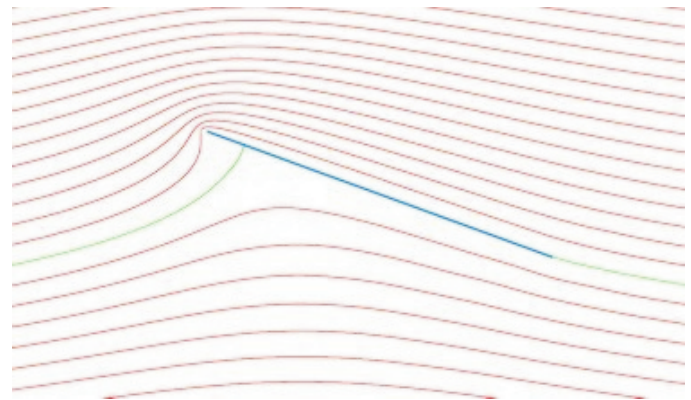
Figure 5. Lifting flow about flat plate.
