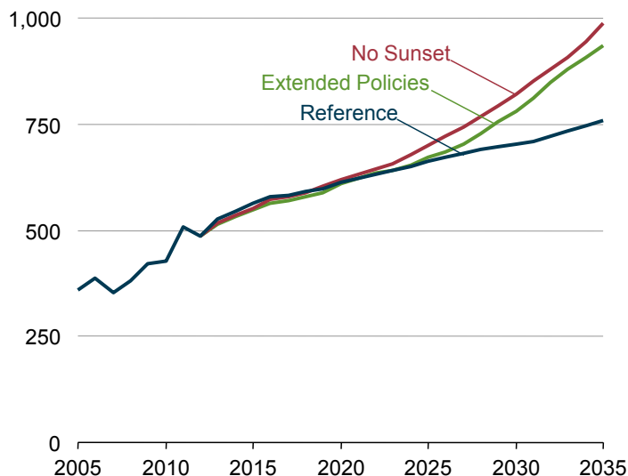
Figure 13. Renewable electricity generation in three cases, 2005-2035 (billion kilowatthours)
