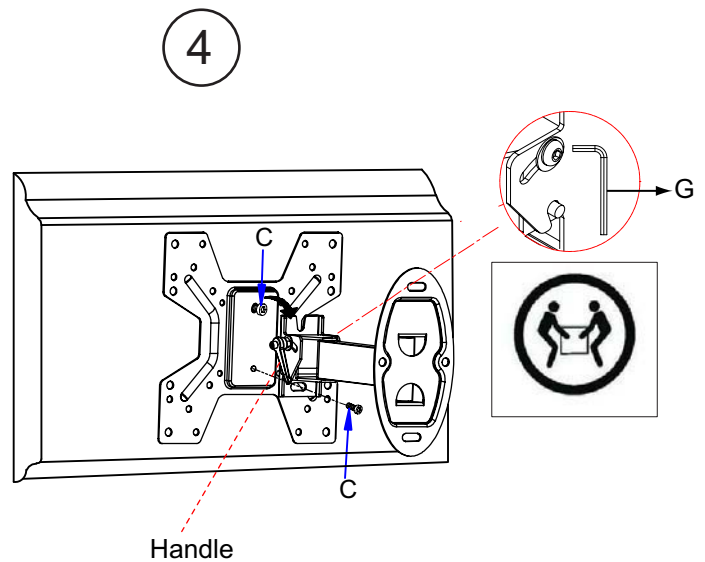
4. Attach the TV to wall bracket(A) with screws(C). You may need rotate the handle to adjust TV to your desired angle, please remember to fasten the screw tightly after adjustment
