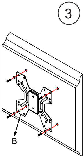
3. Attach TV plate(B) to the back panel of TV.
