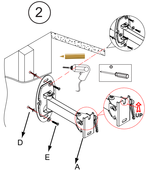
2. Hold wall bracket(A) against wall at desired position, then using a pencil mark 4 hole locations. Then drill holes according pencil marks using 5/16" or 8mm size drill bit to a depth of 2.5"/64mm. Insert wall anchor(D) to the holes, then fix wall bracket(A) to the wall with screws(E).
