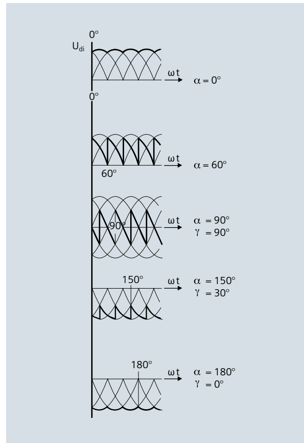
Fig. 3-2: DC voltage of bridge converter as a function of \alpha
