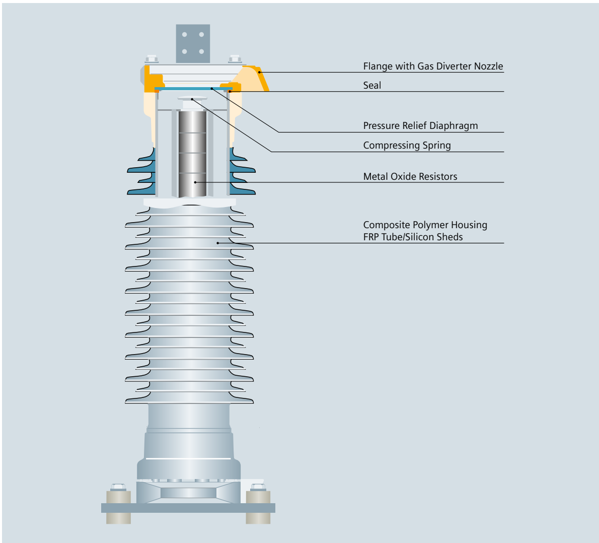
Fig. 5.5-3: Cross-section of a polymer-housed arrester
