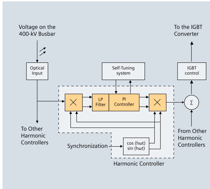
Fig. 5.4.3-3: Principle block diagram of the harmonic control
