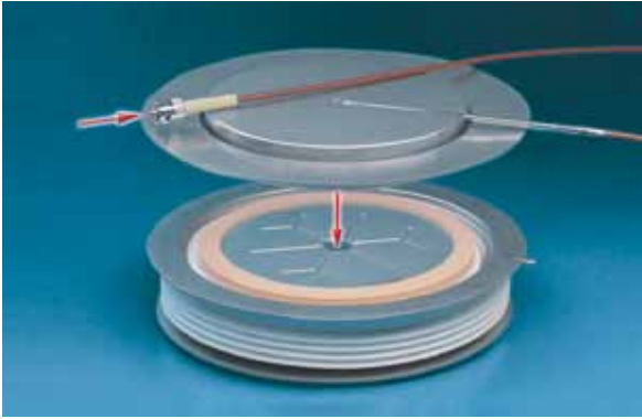
Fig. 5.1-6: Silicon wafer and housing of a direct-light-triggered thyristor
