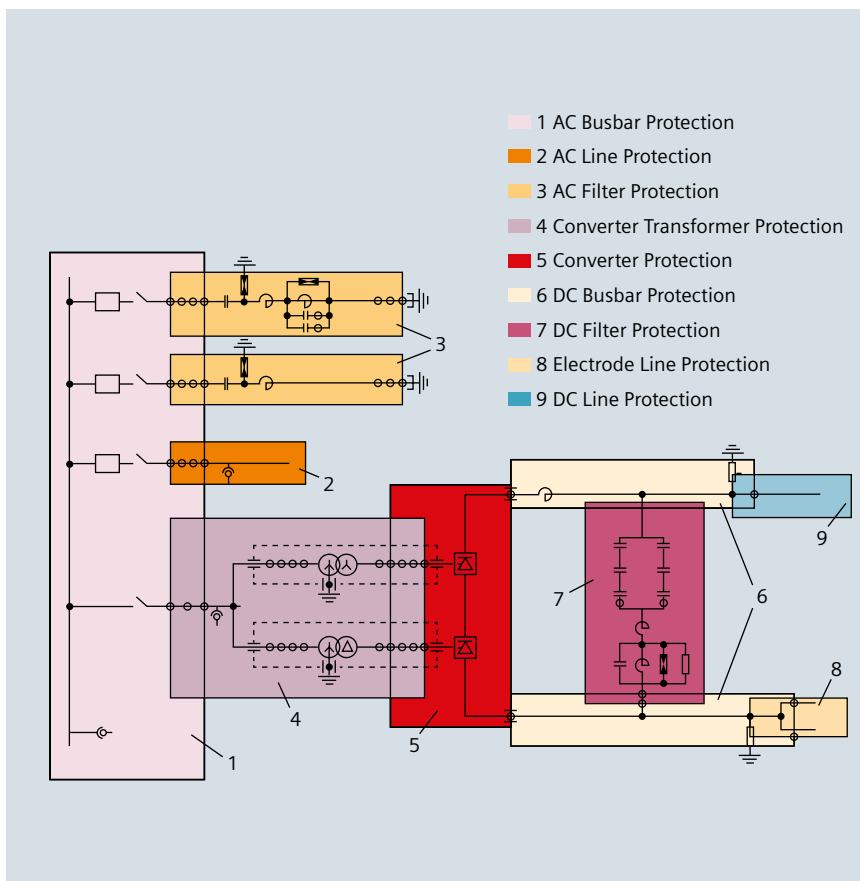
Fig. 5.7.1-8: Protection zones, one pole/one station
