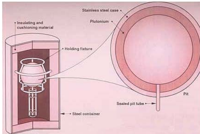
Fig. 8: Plutonium Pit in a stainless steel case and sealed pit tube used for boosting.
