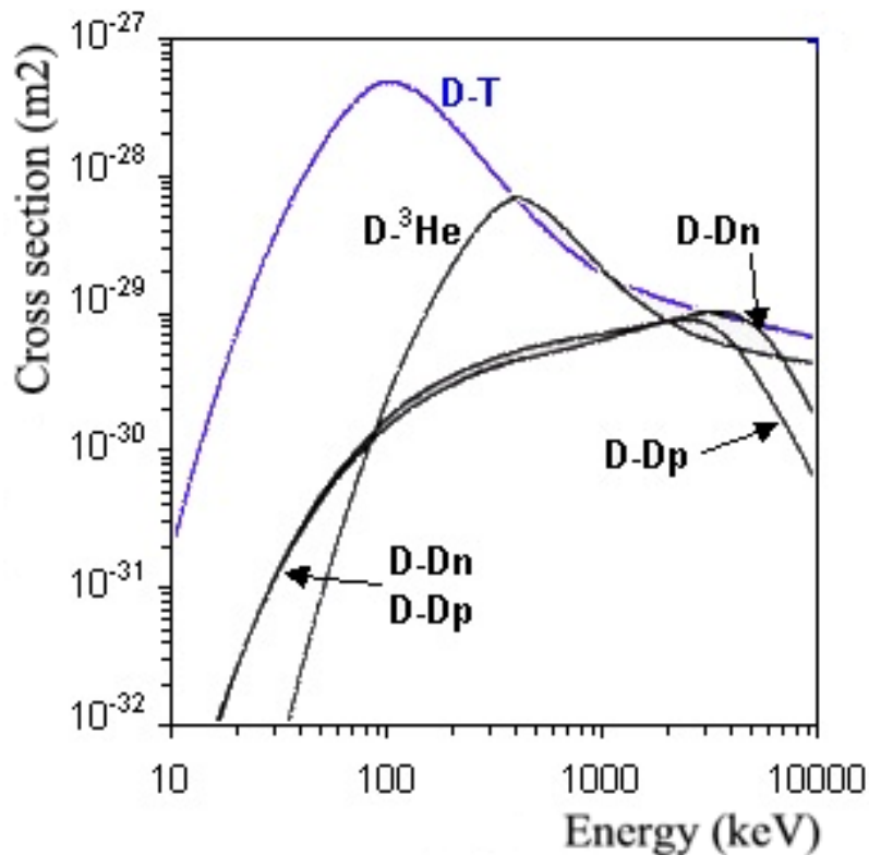
Fig. 3: The cross section for the DT reaction reaches a maximum at about 100 keV at a lower temperature than the maximum of the DD reaction branches.
