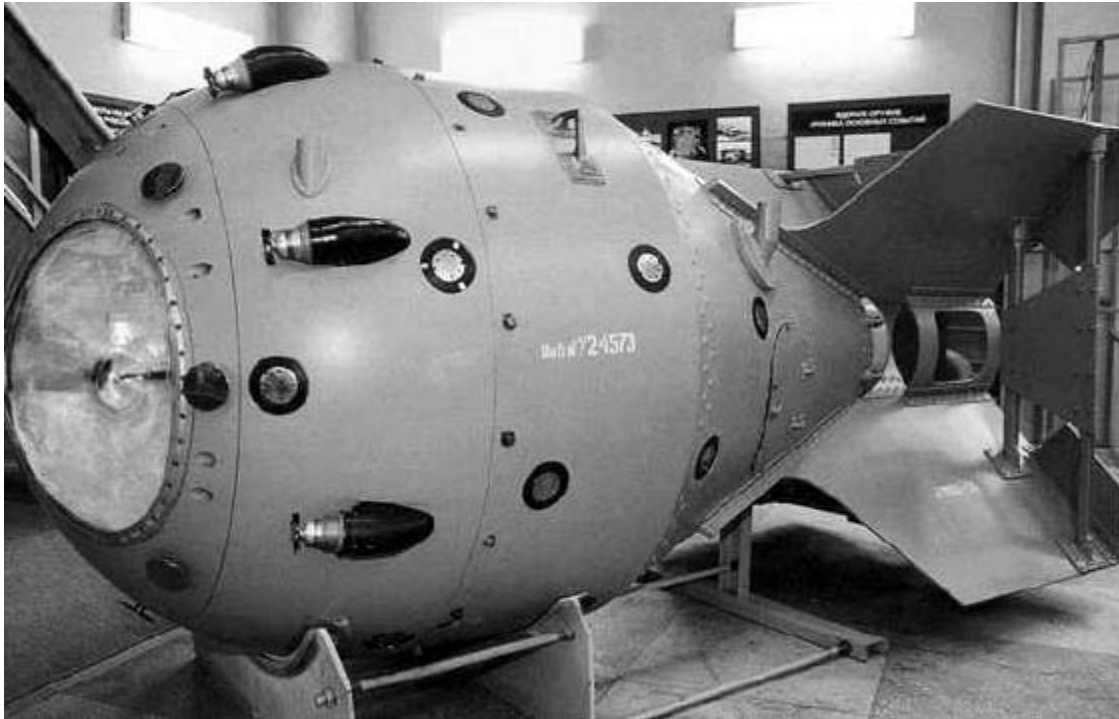
Fig. 6: Replica of RDS-1 the fission Russian analog to the USA Fat Man \text{Pu}^{239} implosion design.
