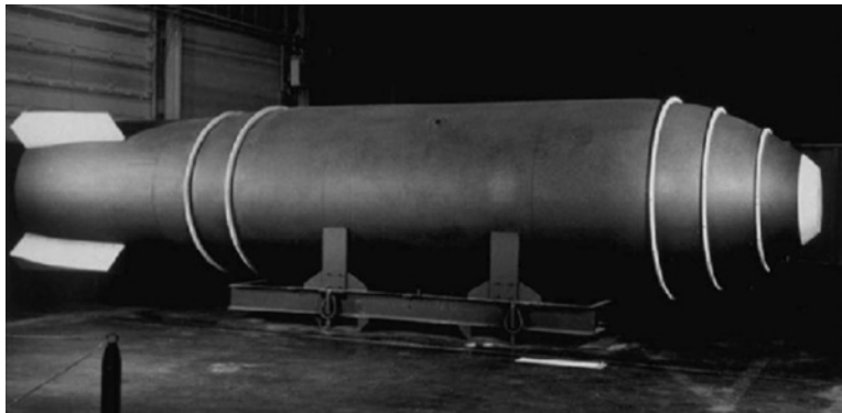
Fig. 15: Mk 17, the \text{Li}^6\text{D} deliverable USA thermonuclear device had a casing 25 ft in length, 3.5 inches in thickness and weighted 21 tons.
