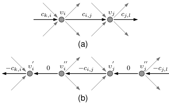
Fig. 13. The two-phase graph transformation. (a) Two nodes v_i and v_j in the original graph. Bold lines (with edge costs c_{\dots} ) represent the arc of a shortest path incident to these two nodes. (b) The same part of the graph after the transformation.
