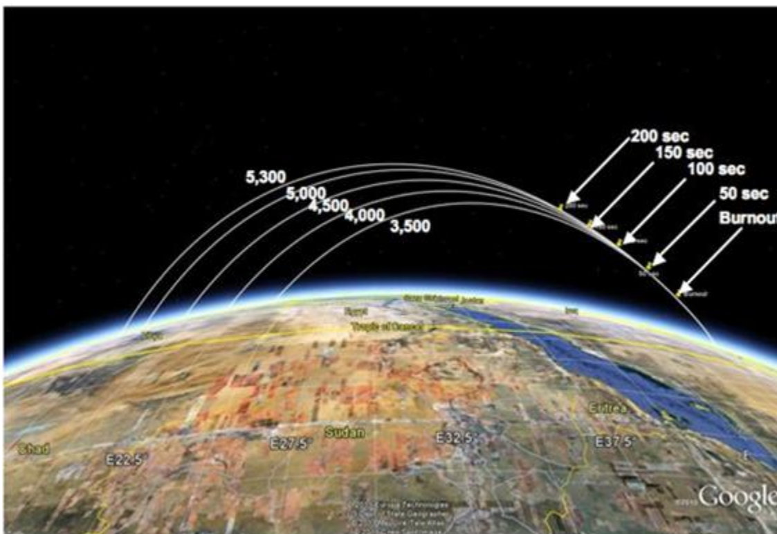
FIGURE 4-4 PTSS view of notional 5,600 km IRBM as the satellite passes over 30 degrees East.
