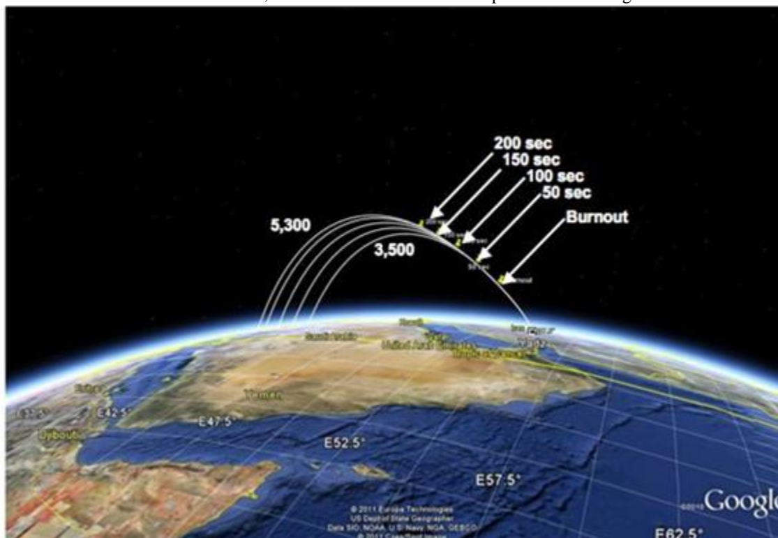
FIGURE 4-5 PTSS view of notional 5,600 km IRBM as the satellite passes over 60 degrees East.
