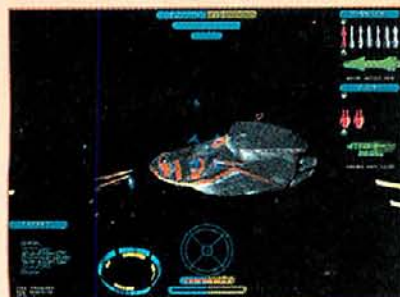
Privateer 2
