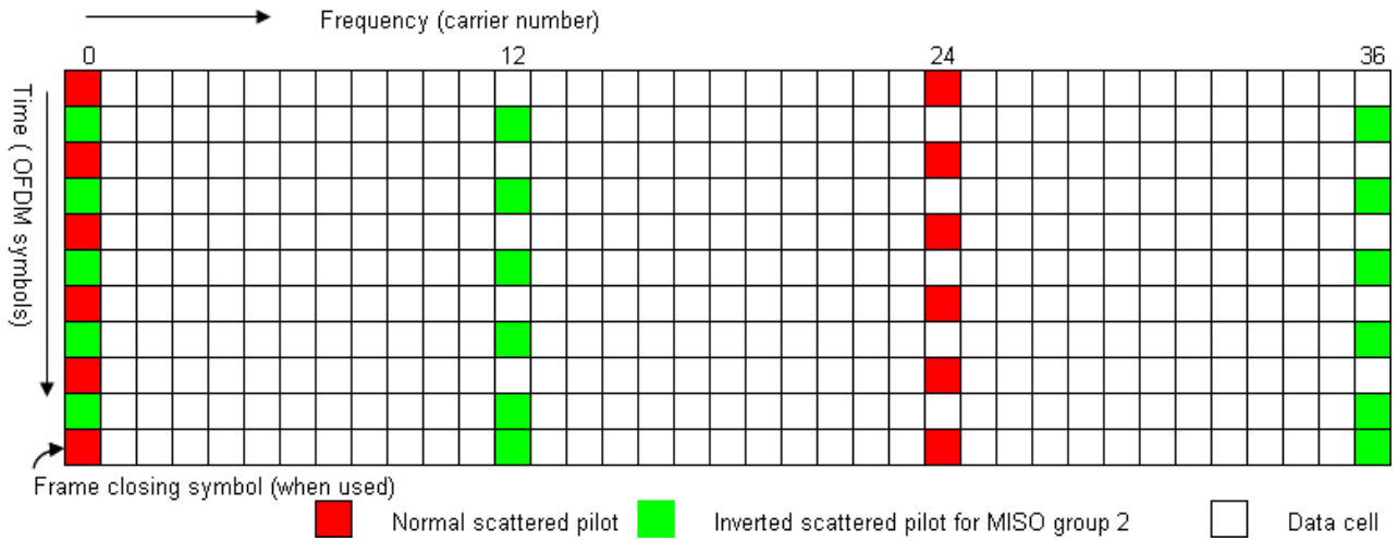
Figure K.12: Scattered pilot pattern PP4 (MISO)
