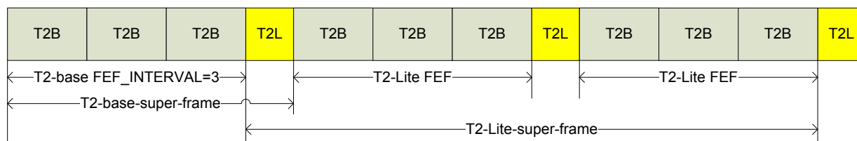
Figure 55(a) Example of a composite T2-base and T2-Lite signal
