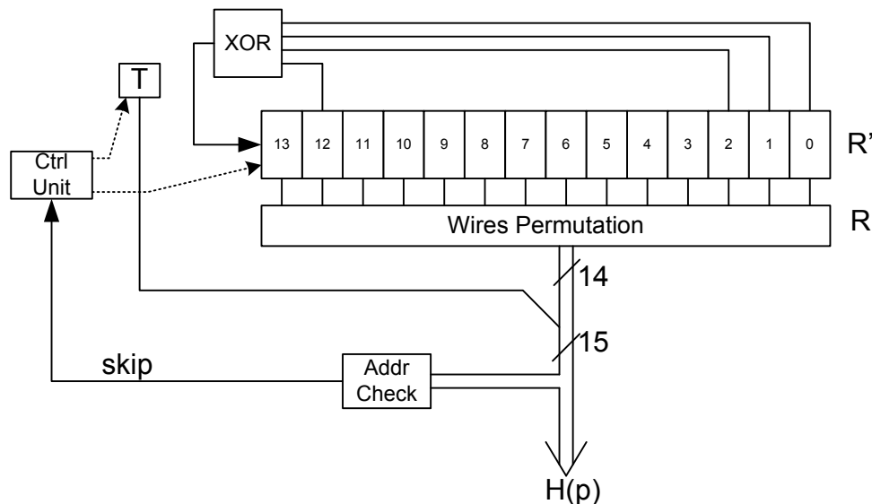
Figure 46(f): Frequency interleaver address generation scheme for the 3k mode
