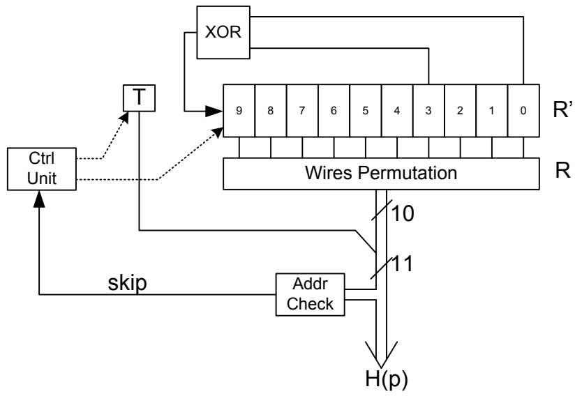
Figure 46(b): Frequency interleaver address generation scheme for the 2k mode
