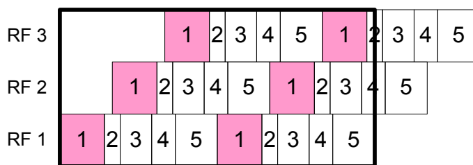
Figure E.3(a): The structure of the type 2 part of a T2-frame with N_{RF} = 3 and N_{subsllices\_total} = 6 before folding, showing the sub-slices exceeding the frame
