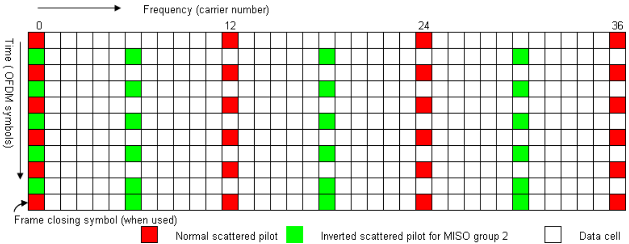
Figure K.10: Scattered pilot pattern PP2 (MISO)
