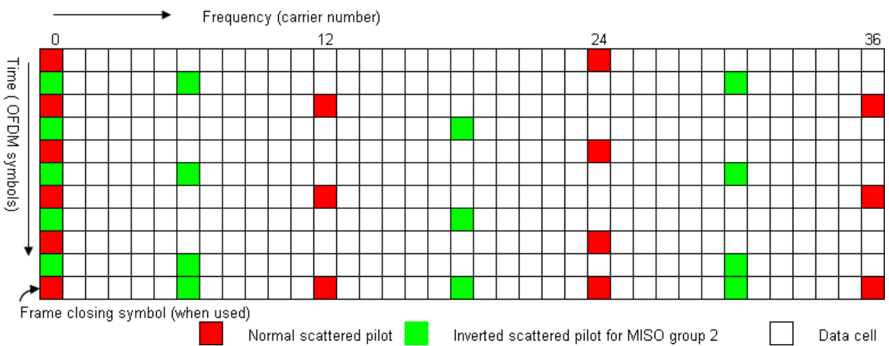
Figure K.11: Scattered pilot pattern PP3 (MISO)
