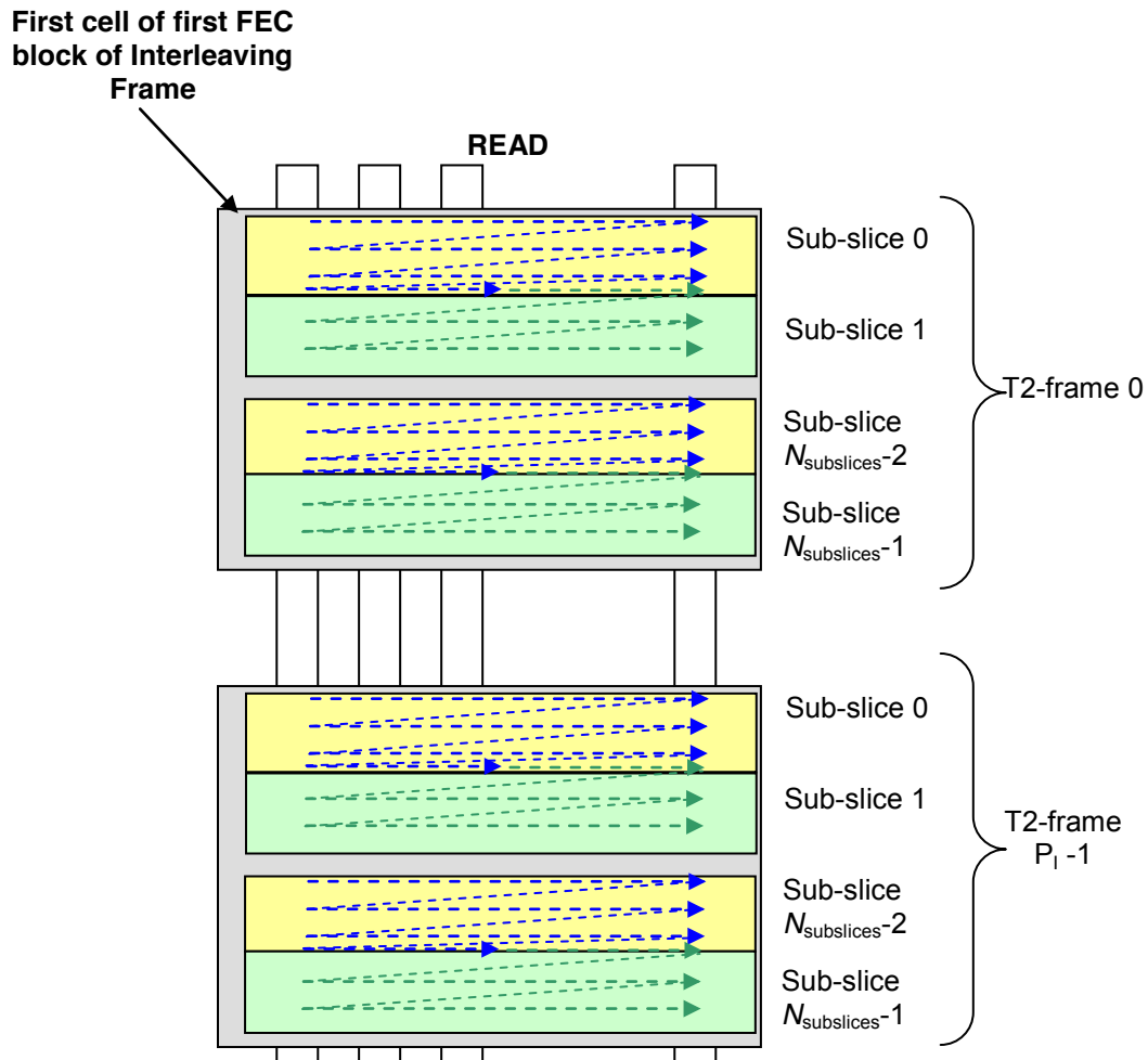
Figure 22: The output from a single TI-block, split into N_{\text{subslices}} sub-slices in each of P_1 T2-frames
