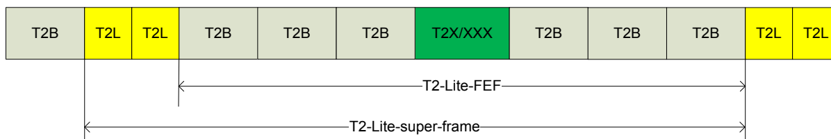
Figure 55(b) Example of a composite T2-base and T2-Lite signal
