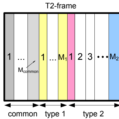
Figure 42: Allocation of M_{\text{common}} common PLPs, M_1 data PLPs of type1 and M_2 data PLPs of type 2 transmitted in one T2-frame
