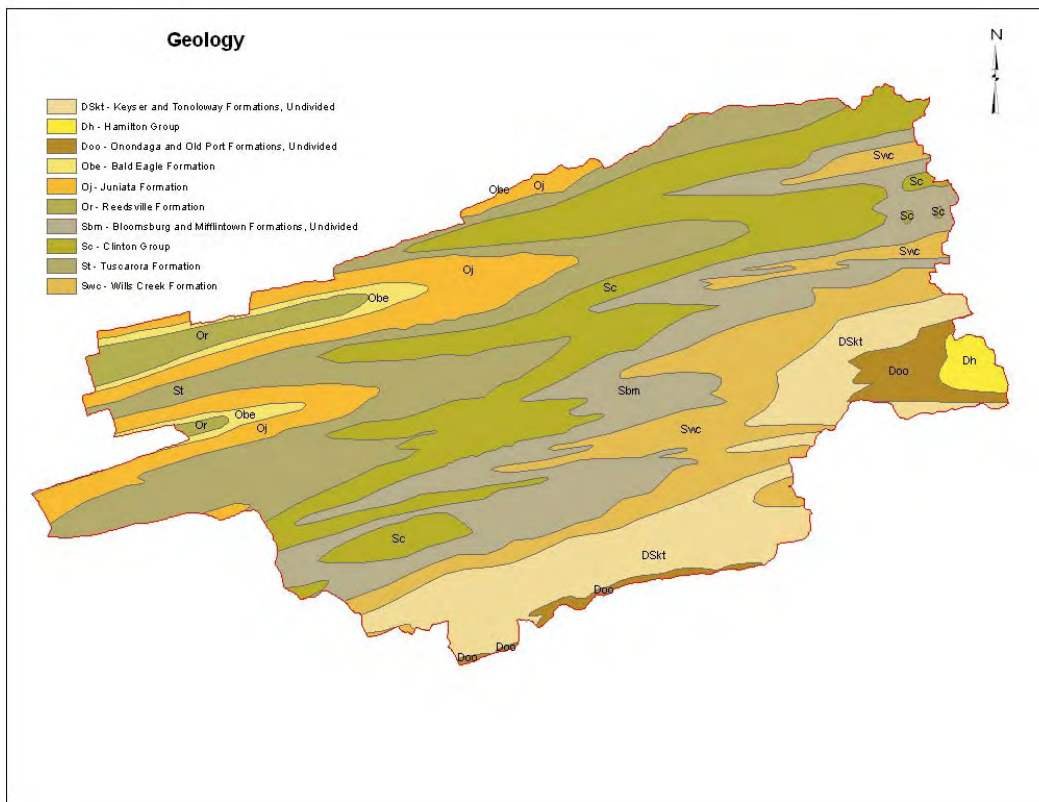
Figure 2.1 Surface geology of the Buffalo Creek watershed.
