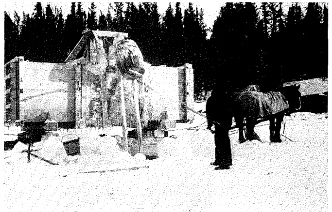
Seven of these wooden water tanks were used to ice the land stretches between the frozen lakes on the way to Island Falls. The ice covered land made travel much easier for the linn tractors and sleighs. (F. Willis 1928)
