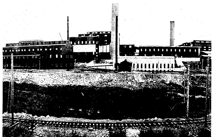
Almost ready for operation. Copper smelter and zinc plant. August 1930 (HBM&S)
