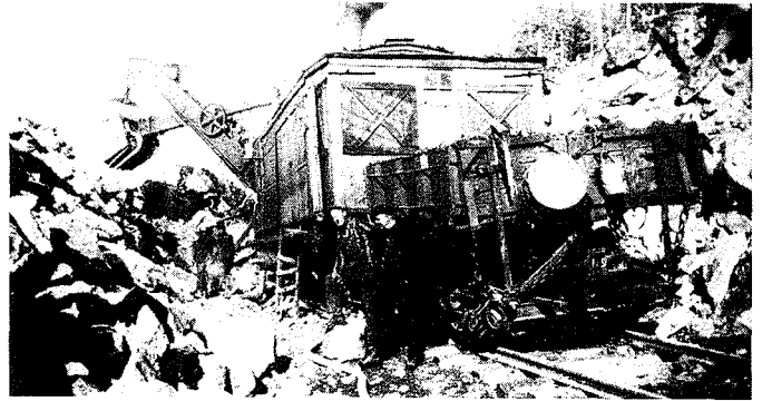
Clearing blasted rock. The side car was used for dumping gravel. (F. Wells 1928)
