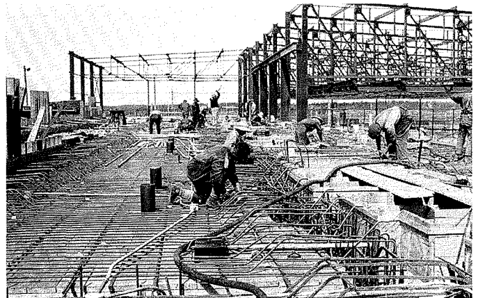
Erection of steel for zinc plant buildings by the Dominion Bridge Co., Limited. (H. Ennis 1929)
