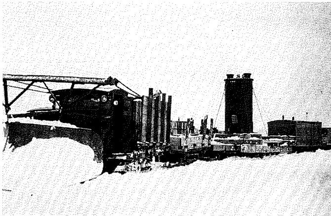
Linn tractors were equipped with snow plows and were capable of hauling up to 38 tons, the weight of this load. The huge transformer had to be transported on a specially built rack. (F. Willis 1928)
