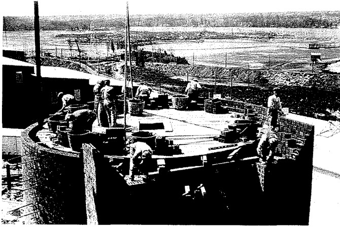
Custodis Chimney Company was contracted to build the two stacks. (W. S. B. Lockhart 1930)
