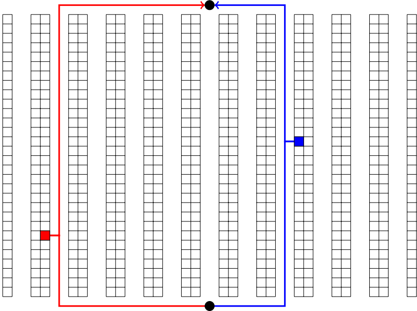
Figure 6.8: The blue location (right) is more convenient than the red location (left) because the total distance from receiving to the location, and from there to shipping is smaller.
