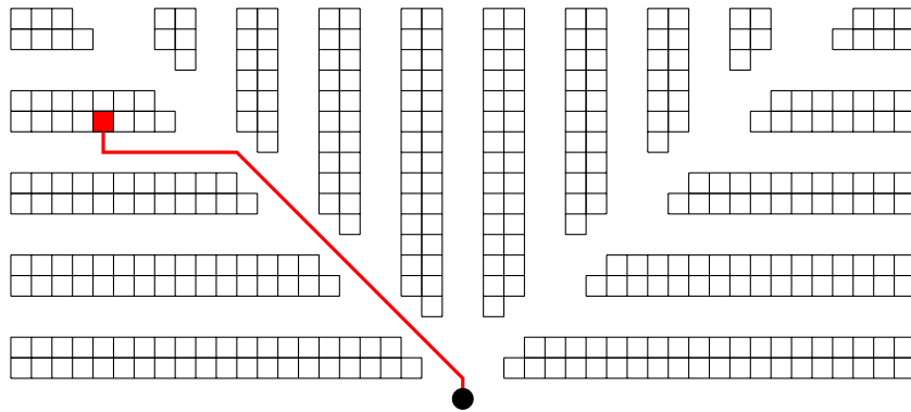
Figure 6.12: Angled aisles, suggested by Gue and Meller, allow more direct travel between storage and a central location of receiving/shipping (at the bottom).
