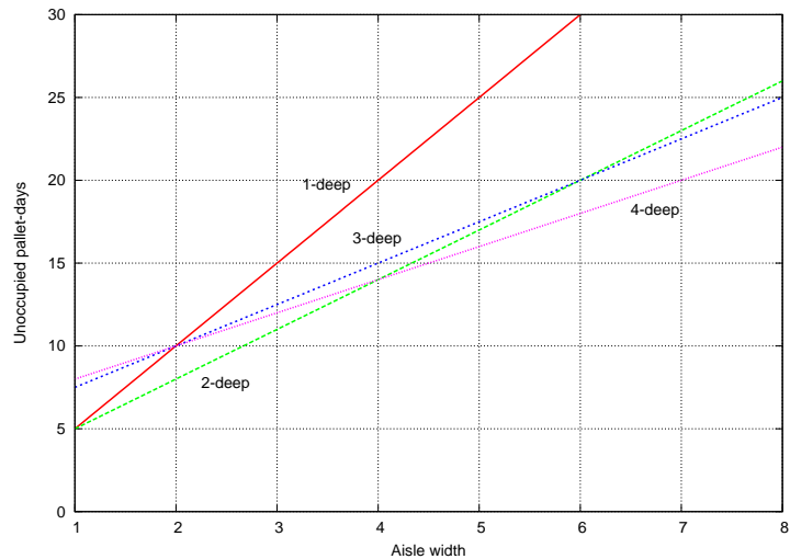
Figure 6.4: Waste, measured as pallet position-days that are unoccupied but unavailable, depends on both the lane depth and the aisle width. The four pallets of this sku should be stored either 2-deep or else 4-deep, depending on the width of the aisle.
