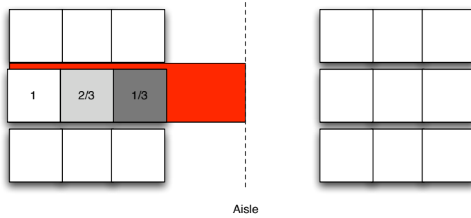
Figure 6.3: The floor space charged to a lane includes storage space, any gap between lanes, and one-half the aisle width in front of the lane.
