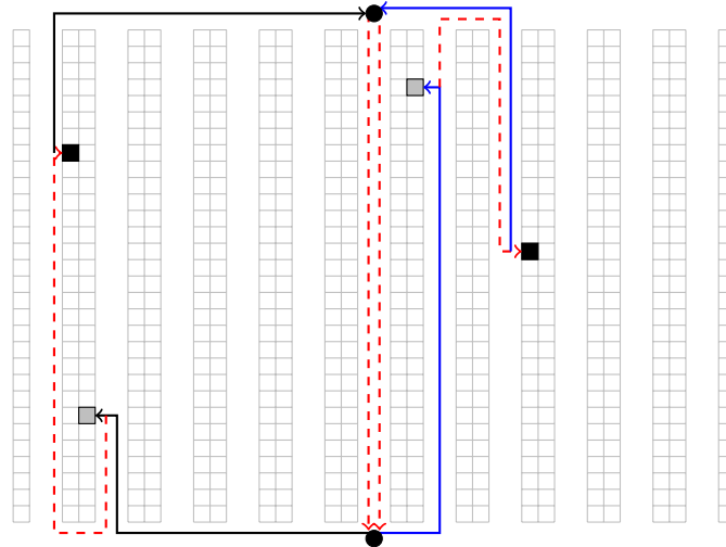
Figure 6.7: When receiving and shipping are separated, a dual-cycle trip must dead-head between them (dashed red line in the center).
