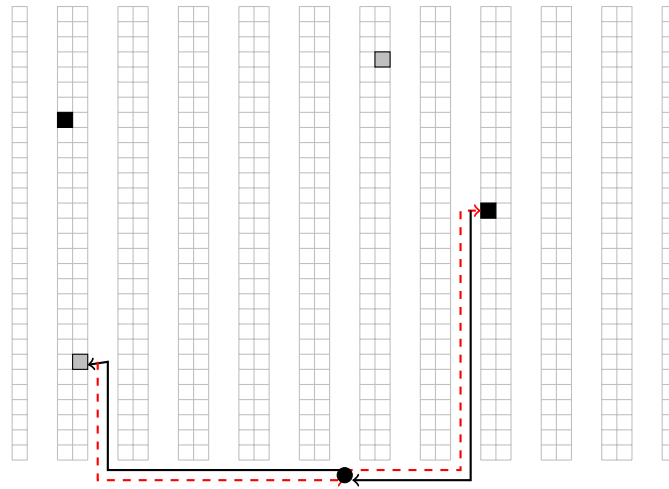
Figure 6.5: Under single-cycle protocol, only half of forklift travel is productive. In this example, both receiving and shipping are at the bottom, and the trip to the left, to stow a pallet in an available location, requires that the forklift return with empty forks (red dashed line). The trip to the right, to retrieve a pallet, requires that the journey begin with empty forks.
