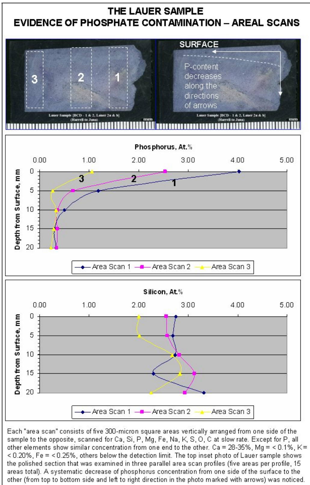
Figure 13: Further evidence of phosphorus contamination in the Lauer sample. Notice the decrease in P concentrations along three area profiles 1, 2, and 3 on the top photo whereas more or less consistent concentration of silicon (and other elements) in these areas. Based on this analysis, the maximum depth of phosphorus contamination is judged to be ~5 mm from the sectioned edge.
