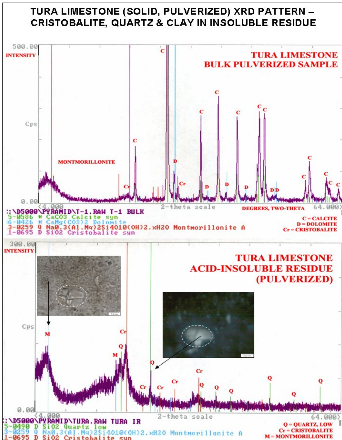
Figure 9: X-ray diffraction patterns of the Tura limestone (top), and its acid-insoluble residue (bottom) showing: (a) the dominance of calcite with a minor amount of dolomite in the limestone; and (b) the presence of quartz, cristobalite (opal-CT), and sodium montmorillonite clay in the insoluble residue. The inset optical micrographs of oil immersion mounts of the acid-insoluble residue in the bottom pattern shows clay and a quartz grain (circled).
