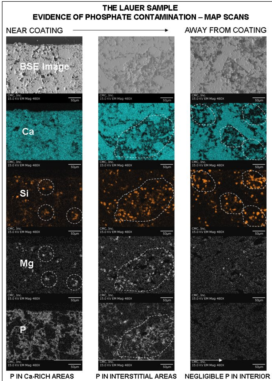
Figure 14: Further evidence of P-contamination - Elemental mapping of polished section of the Lauer sample in three 300\mu\text{m}^2 areas located diagonally across the section from the most contaminated zone at the top corner (shown by the left column of analyses with the maximum P) to the uncontaminated interior at the opposite corner (shown by the right column of analyses with negligible P). Notice in the contaminated zone P occurs mostly in the areas of Ca, indicating a possible calcium-phosphate based chemistry, whereas away from this zone, in the middle column, P occurs in the interstitial and in Ca-rich areas. The Si-rich interstitial phases are also enriched in Ca and Mg.
