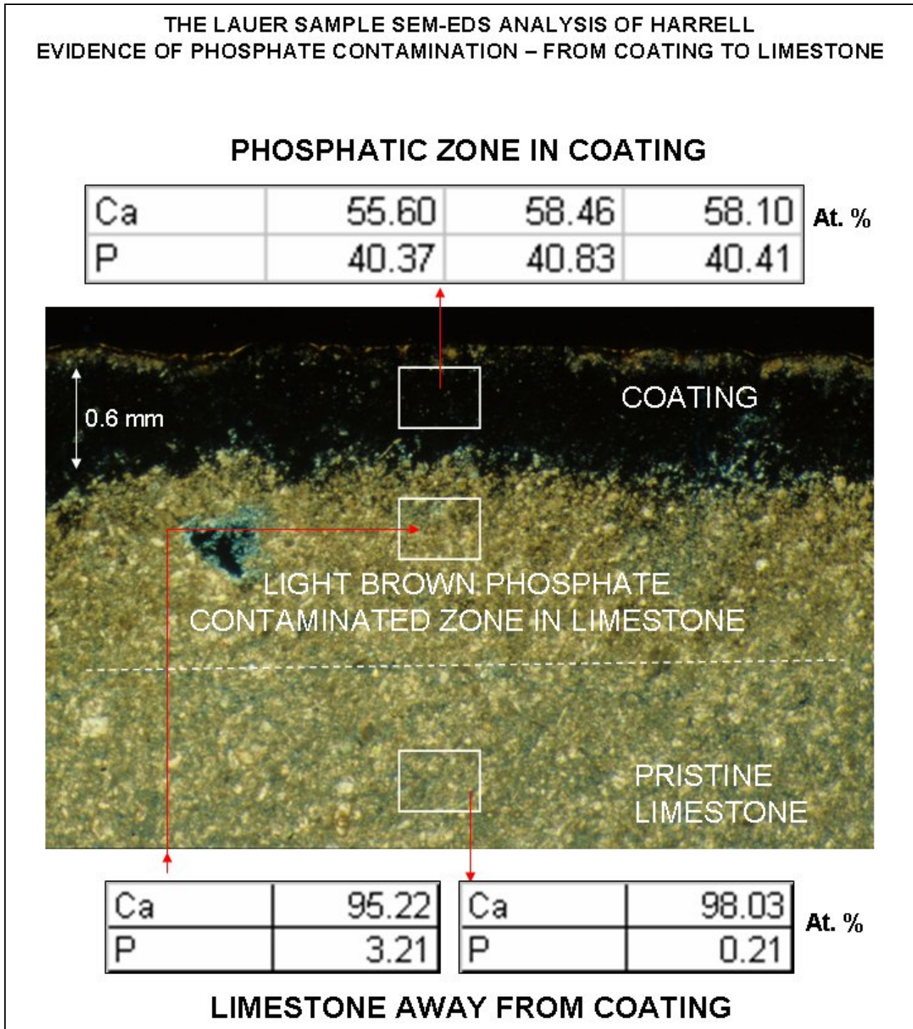
Figure 15: Photomicrograph of thin section of the Lauer sample studied by Harrell (Harrell and Penrod 1993), which contained a dark isotropic coating layer (approximately 1 mm in maximum thickness) on top of limestone, which is followed by a light brown contaminated zone in the limestone, and then the uncontaminated interior. Inset EDS analyses of the coating and the interior limestone show the calcium phosphate composition of coating (consistent with Davidovits’ XRD results) and the absence of a phosphate-phase in the interior limestone. Despite the absence of this “coating”, Figures 12 through 14 in this present study clearly detected evidence of phosphorus invasion in limestone presumably from this coating, extension of contamination to a distance of approximately 5 mm, and the existence of bulk interior “uncontaminated” limestone devoid of any phosphate phase. The coating layer is described in detail in Harrell and Penrod (1993). Photo courtesy of James A. Harrell.
