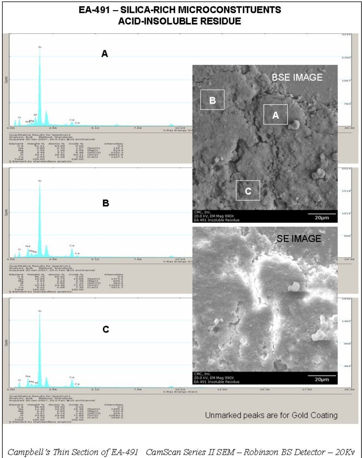
Figure 18: Backscatter electron image (inset top right), secondary electron image (inset bottom right) and x-ray elemental analyses (left photos) of hydrochloric acid-insoluble residue in EA-491. The residue is silica-rich with minor amounts of Ca, Na, Mg, and Al. Analyses of the boxed areas marked as A, B, and C in the BSE image are given in the left. Optical microscopy determined the presence of quartz, opal-CT, clay, and iron oxide in the residue (this study, Campbell and Folk 1991, Freestone et al. 1984).
