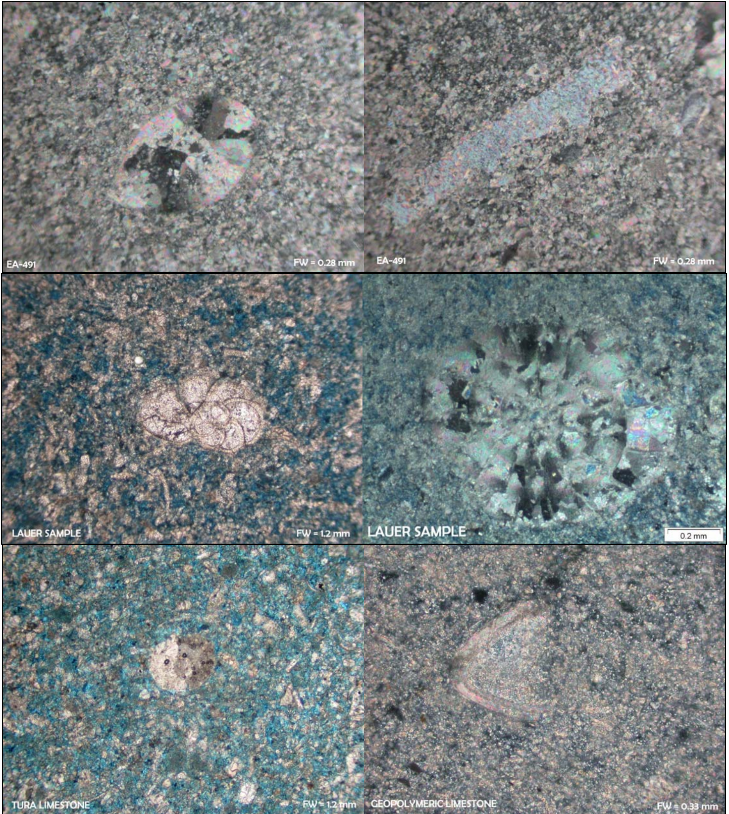
Figure 2: Photomicrographs of thin sections of casing stones (EA-491 and the Lauer sample), Tura limestone, and geopolymeric limestone showing some bioclast fragments (e.g., foraminifera, molluscs) and overall texture of the microcrystalline calcite grains in the surrounding areas. FW (Field Width) is the distance from left to right of a photo.
