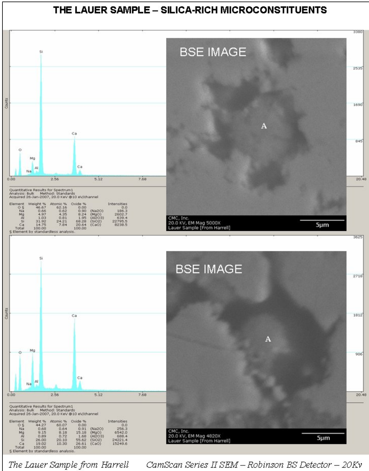
Figure 19: Backscatter electron images (inset top and bottom right) and x-ray elemental analyses (left photos) of spherical silica-rich microconstituents in the Lauer sample. The silica-rich spherical phases, presumably described as lepispheres or opal-CT also contain subordinate amounts of Ca and Mg and minor amounts of Al, and Na. Two different areas are analyzed. The sample contains many such areas with similar compositions. These silica-rich spheres correspond to Si-rich spots on dot maps shown in Figure 16.
