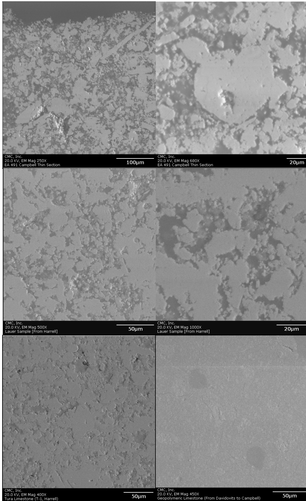
Figure 5: Backscatter electron images showing the overall particulate texture with intergranular pore spaces in the casing stones and Tura limestone, whereas relatively smooth texture with two spherical air voids in the geopolymeric limestone.
