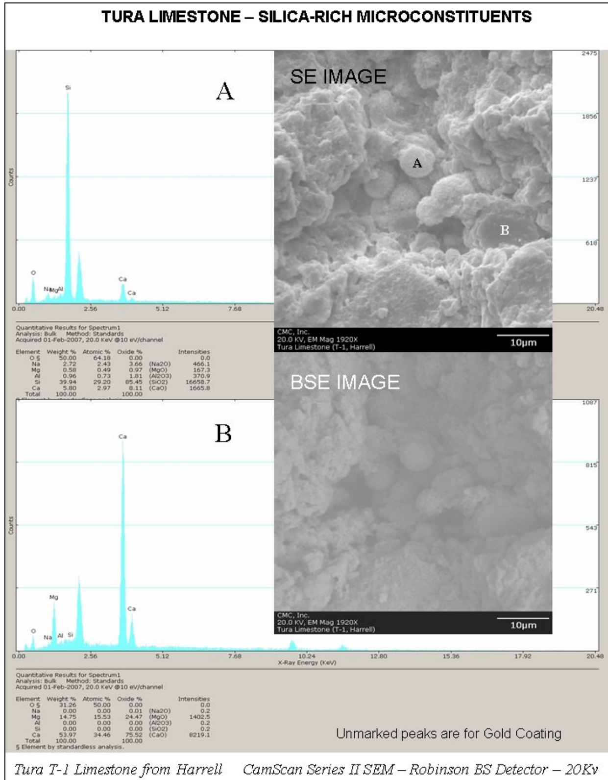
Figure 21: SE and BSE images of Tura limestone showing a bunch of silica-rich lepispheres with an analysis of one such sphere marked as “A”. All spheres are similar in compositions, with Si>>>Ca>Na>Al>Mg, identical to those detected in the Lauer sample and EA-491, and represent impure lepispheres. Area “B” is probably a dolomite phase (also detected in XRD study).
