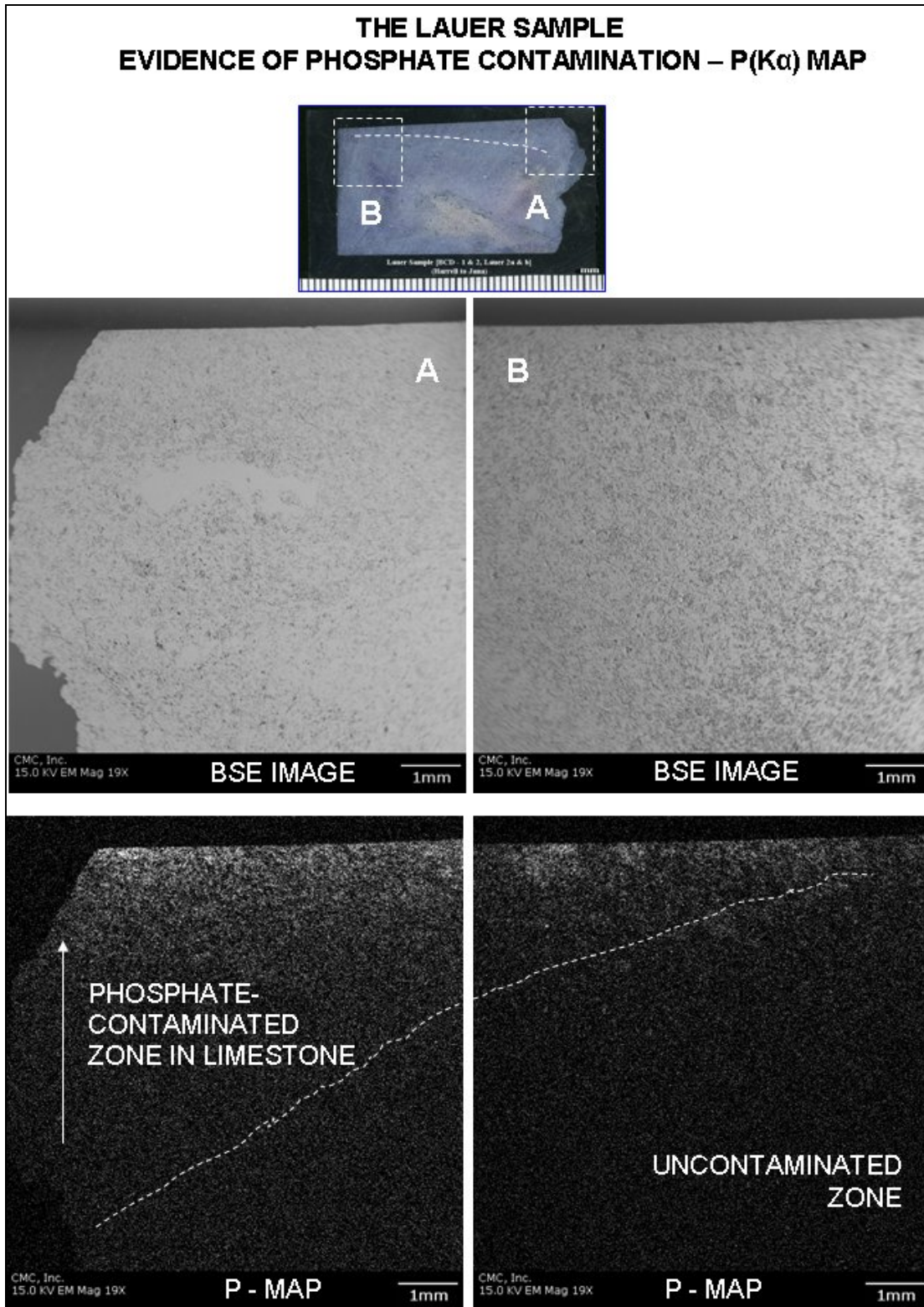
Figure 12: X-ray elemental (phosphorus) map of the Lauer sample over a broad area from one side of the sample (shown in the top photo) showing distinct P-enrichment at one corner on the top and its progressive decrease in concentration towards opposite ends (bottom photos). The middle photos are backscatter electron images of the boxed areas A and B on the sample (top photo); the lower photos are the P-scans over these areas. The P-contaminated zone is separated by a dashed line (bottom photo) from the interior uncontaminated limestone. The calcium phosphate phases that Davidovits detected in his XRD pattern of the Lauer casing stone sample most probably came from the contaminated zone.
