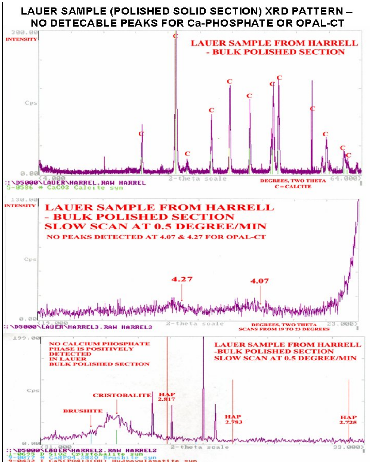
Figure 8: X-ray diffraction pattern of polished section of the Lauer-Harrell sample, which was used for the SEM work. The pattern shows the dominance of calcite, as expected; and an apparent absence of an opal-CT or a calcium phosphate phase on a polished section (during slow scans in 2θ ranges where characteristic diffraction peaks were detected in Davidovits’ 1986 study). Optical and scanning electron microscopy, however, clearly detected silica-rich spherical microconstituents in this sample, which, therefore, indicates an integrated approach of optical-SEM-XRD work for definitive detection of microconstituents in these samples.
