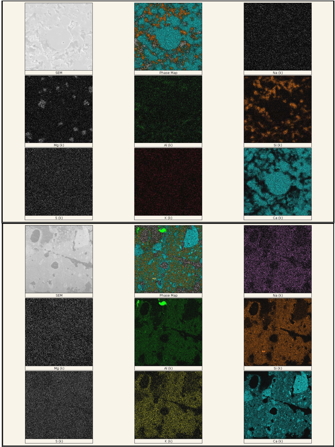
Figure 11: X-ray elemental analysis (SEM-EDS) of Tura Limestone (top) and Davidovits' Geopolymeric Limestone (bottom). Similar to the patterns seen in the casing stones, Tura limestone shows: (a) the dominance of Ca-rich areas (in blue) corresponding to the calcite grains, (b) Si-rich areas (in brown) as isolated, mostly near-spherical to irregularly shaped interstitial areas, some of which correspond to the Mg-rich ones (in white); and (c) complete absence of any indication of alkali (Na, K) or alumina (Al) enrichment in the binder phases (interstitial areas) or in grains, which Davidovits' lime-natron-clay based geopolymeric chemistry produces in the bottom photo. Notice the uniform and distinct enrichment of Na (in purple), K (in yellow), Al (in green), and Si (in brown) in the geopolymer matrix, and occurrences of Si as uniform mass in a geopolymer matrix rather than interstitial, isolated "spots/grains" as in the pyramid samples and Tura limestone.
