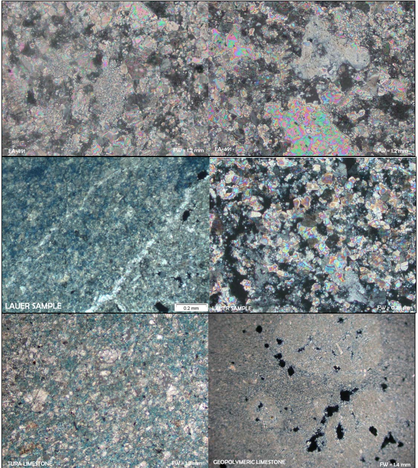
Figure 3: Photomicrographs of thin sections of casing stones (EA-491 and the Lauer sample), Tura limestone, and geopolymeric limestone showing the overall texture of micritic calcite grains, fine-grained micritic lumps in casing stones, spherical and elliptical lumps of calcite dust in geopolymeric limestone, and a calcite-filled fracture in the Lauer sample. FW (Field Width) is the distance from left to right of a photo.
