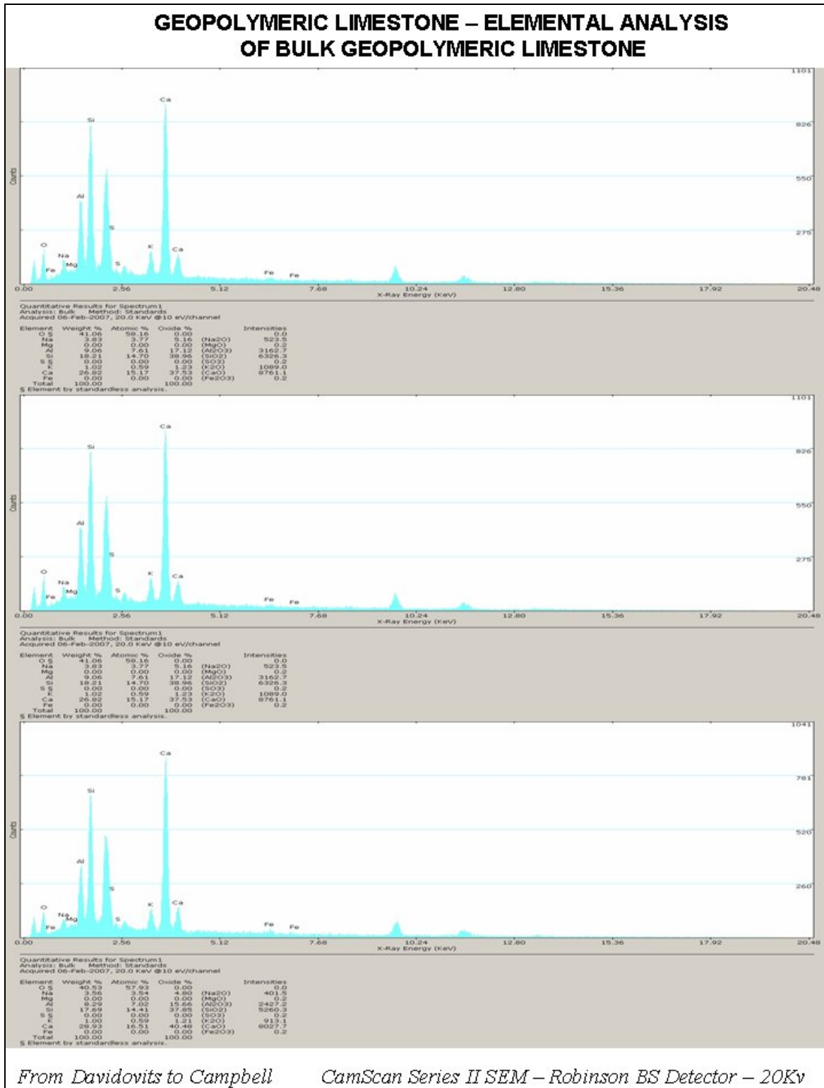
Figure 24: X-ray elemental analysis of different areas of geopolymeric limestone sample of Davidovits showing its distinct characteristic composition of calcium (from limestone) and enriched alkali (Na+K)-aluminosilicate composition, as expected for a geopolymeric binder. Notice the total alkali (Na 2 O+K 2 O) and alumina (Al 2 O 3 ) content in this limestone is significantly higher than those detected in all silica-rich microconstituents. These results are consistent with uniform enrichment of Si-Na-K-Al found in the elemental maps of this limestone. Neither the casing stone nor the natural limestone showed this characteristic composition.
