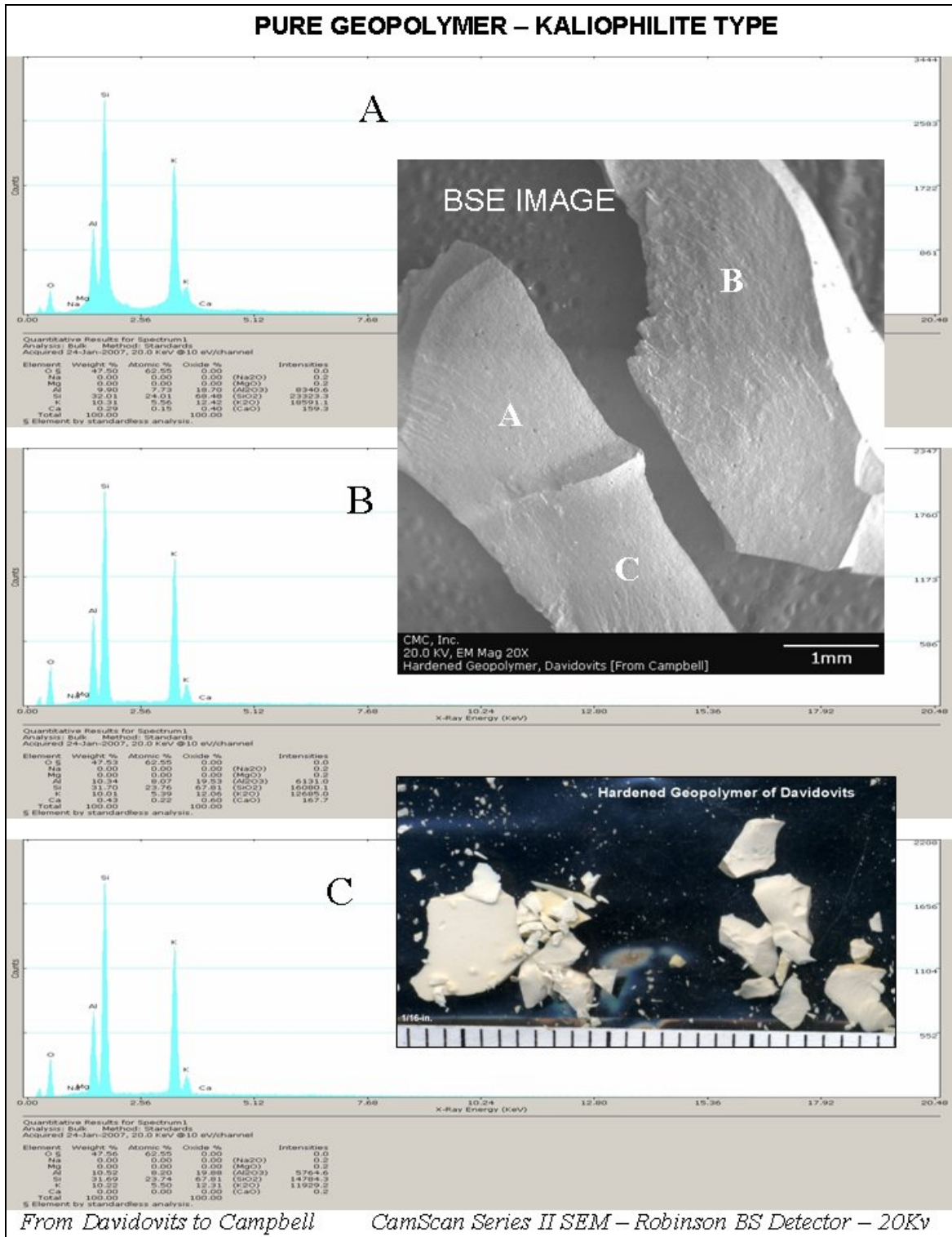
Figure 25: Backscatter electron image (the top right photo), actual fragments as received (the bottom right photo), and x-ray elemental analyses of three areas (marked as A, B, and C) of Davidovits’ pure geopolymer sample (Kaliophilite base - type K-PSS) showing its characteristic potassium aluminosilicate composition. A geopolymeric limestone, made using a similar sodium or potassium activated aluminosilicate binder should detect similar composition (i.e., analcime or kaliophilite-type zeolitic composition) in the “binder” phases of limestone, which is well detected in the geopolymeric limestone of this study but not found in any of the casing stone samples. The lime-natron-clay-based recipe in the geopolymer hypothesis of construction of pyramid stones is apparently yet to be detected in a pyramid sample.
