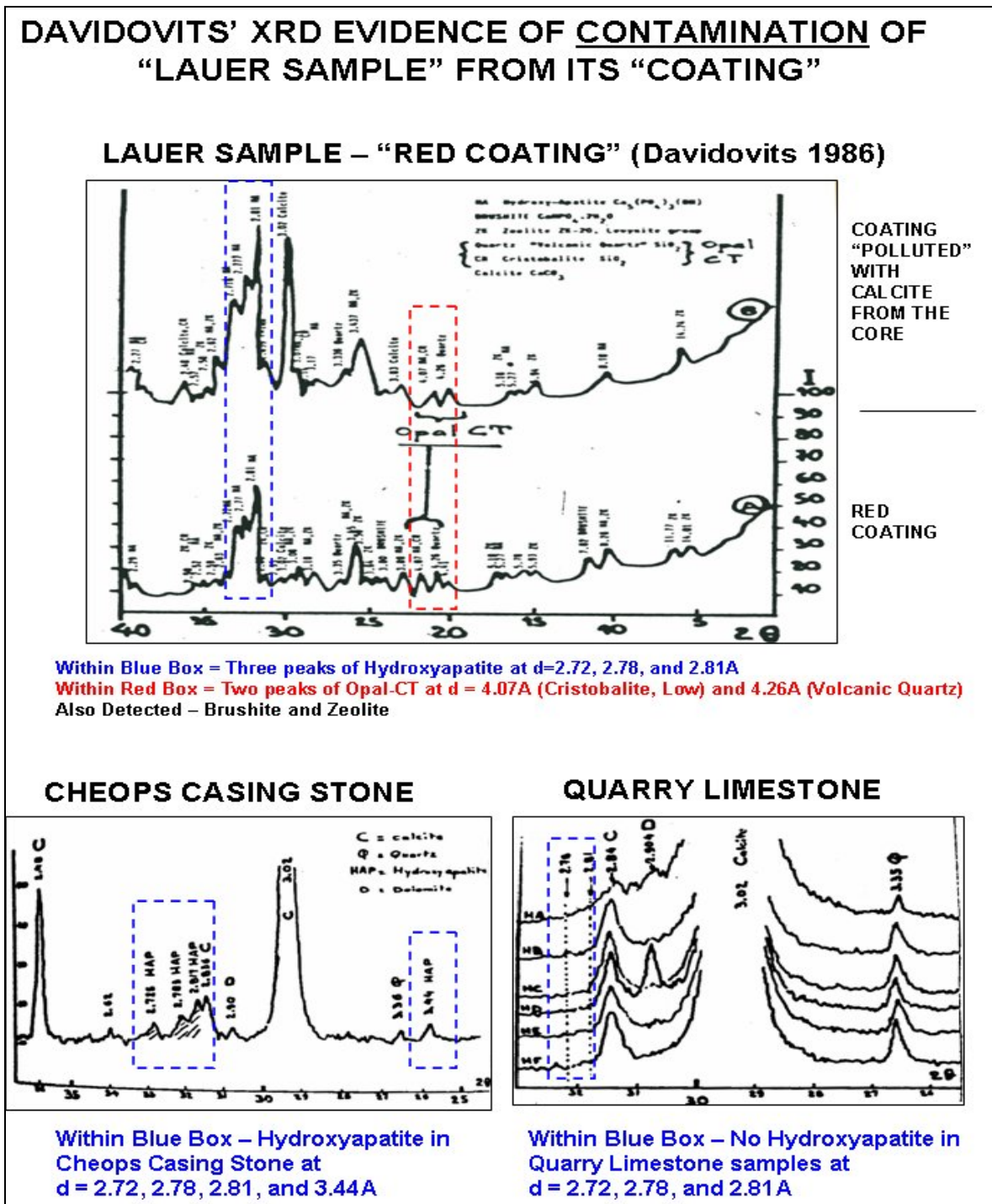
Figure 6: A reproduction of Davidovits' XRD patterns of: (a) the red coating on the casing stone of the Khufu pyramid, (b) the casing stone beneath the coating; and (c) natural (quarry) limestones. The patterns show the presence of a calcium phosphate phase (HAP, hydroxyapatite) in the coating (diagnosed within the blue boxed areas), its detection in significantly less amount in the casing stone beneath the coating, and its absence in the quarry limestone samples. The data itself indicates a possible contamination of the casing stone by the overlying coating materials, which is not present in the quarry limestones. Detection of HAP (and associated traces of coating materials) in the limestone, therefore, does not indicate a "man-made" origin of the casing stone. This statement is supported by the present study, where a clear zone of phosphate contamination is detected in the limestone beneath the coating to a distance of ~5 mm.
