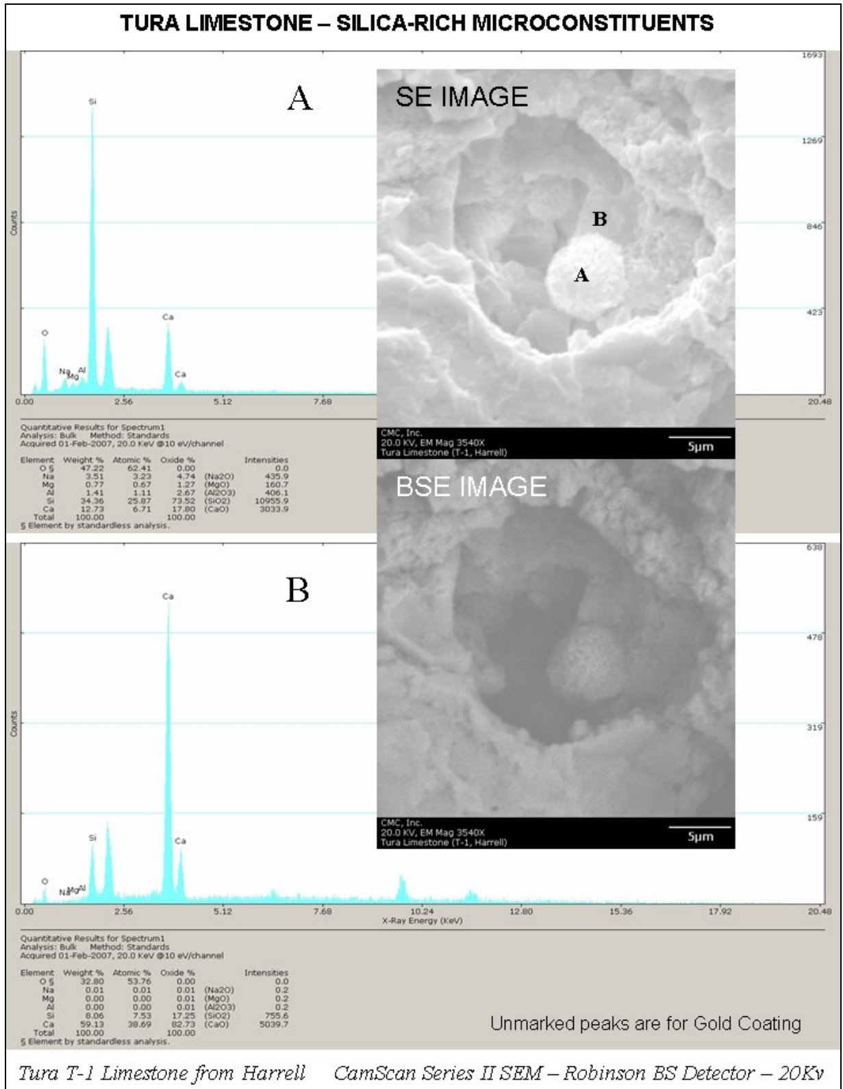
Figure 22: Another excellent example of a silica-rich microsphere in Tura limestone (marked as “A”) having significant amount of SiO 2 , followed by CaO>>Na 2 O>Al 2 O 3 >MgO. All these lepispheres in Figures 21 and 22 are silica-rich, detected in the casing stone samples as well as in natural limestone, and contain variable amounts of Ca, Mg, Al, and Na as impurities.
