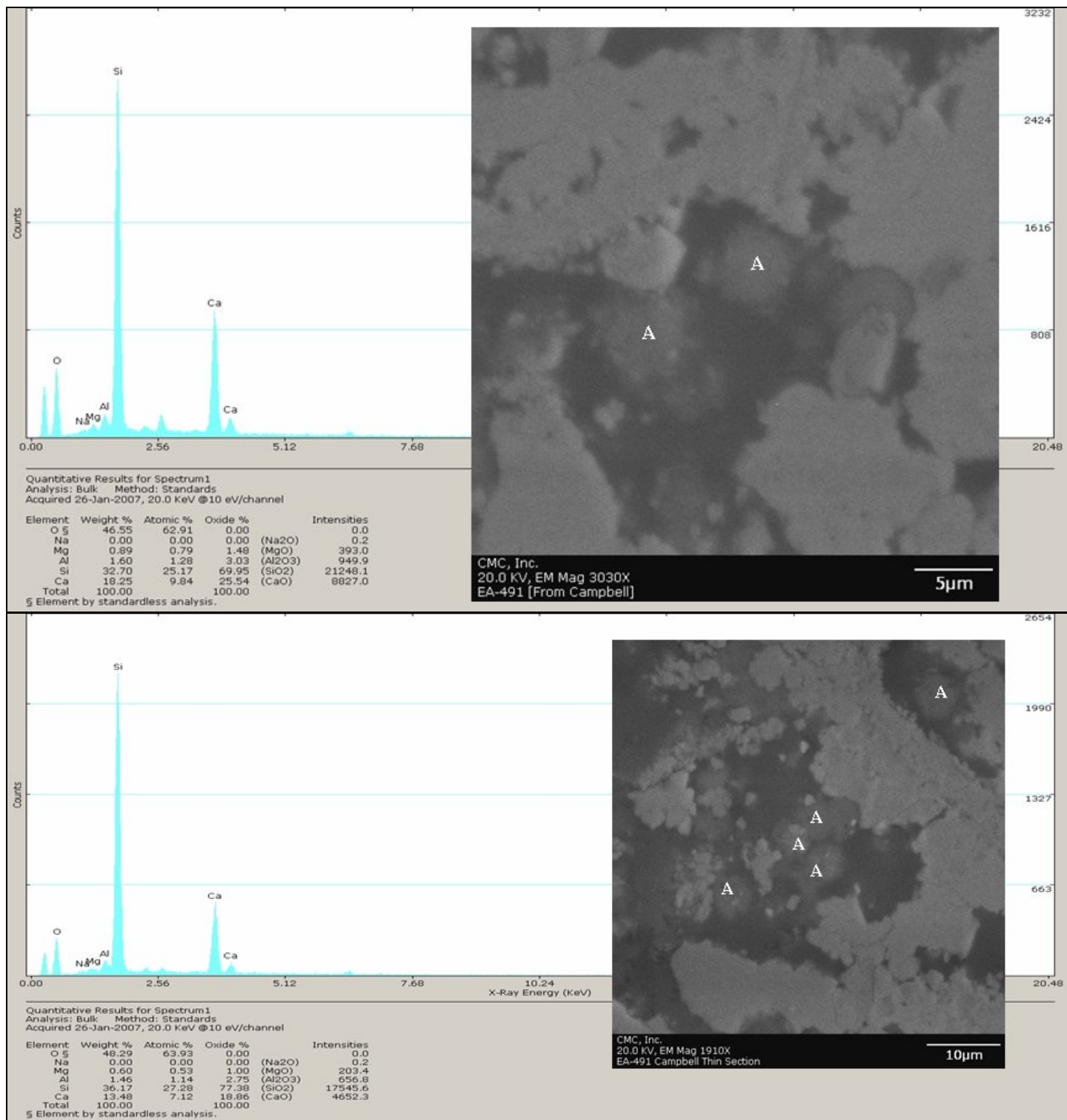
Figure 17: Backscatter electron images and x-ray elemental analyses of near-spherical silica-rich microconstituents (areas marked as “A”) in EA-491 that are described as “lepispheres” in Campbell and Folk (1991) and Bradley and Middleton (1988). All silica-rich areas have more or less similar compositions (Si>>Ca>Mg>Al); two representative ones are shown here. Lepispheres are dark gray spheres in these BSE images located in the interstitial spaces, in between the relatively brighter calcite grains.
