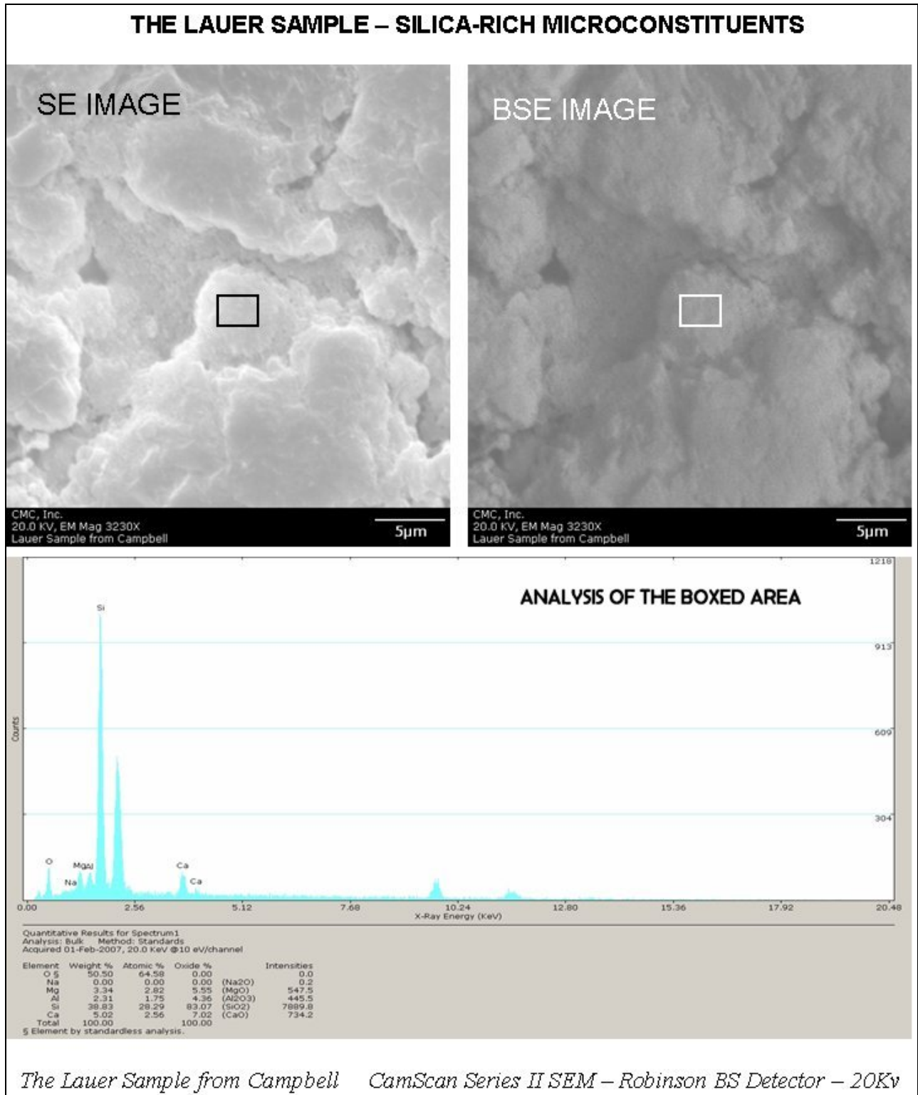
Figure 20: A silica-rich microsphere in the Lauer sample with greater than 80 percent SiO 2 and 4 to 7 percent CaO, Al 2 O 3 , and MgO - a typical example of “impure” lepispheres, a common microconstituent in these limestones. The sphere in this example is approximately 5µm in diameter (lepispheres are 5 to 10µm in size, some are finer than 5µm).
