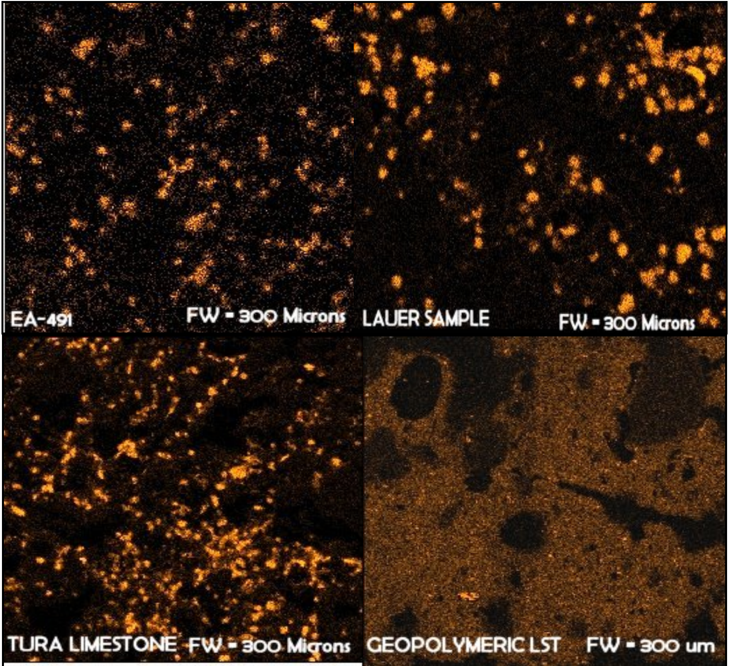
Figure 16: X-ray elemental maps of silicon ( \text{Si-K}\alpha ) in EA-491, Lauer sample, Tura limestone, and geopolymeric limestone. Contrary to the geopolymeric limestone chemistry, where silica occurs uniformly over the entire alkali-aluminosilicate based geopolymeric binder (the bottom-right image), in casing stone and Tura limestone samples, silica occurs as isolated, small (less than 10\mu\text{m} in diameter), spherical, near-spherical, or irregularly shaped, interstitial areas in between the calcite grains that are distinctly highlighted by the Si “spots” in these elemental maps. Notice the near-spherical shapes of these Si-spots in casing stone samples and in many areas in the Tura limestone, which correlate well with spherical silica-rich phases that are detected in SE-BSE images of these samples (see Figures 17-23). An image analysis of these “dot maps” by Image Pro Plus software ( www.mediacybernetics.com ) detected approximately 10 to 15 volumetric percentages of silica rich areas in these samples (taken from 10 to 15 different area scans like these in each sample). Occurrences of these silica-rich phases do not indicate a “man-made” origin of limestone. They are common constituents in many natural limestones, including the ones at Giza and have been described by many as “lepispheres” of opal-CT mineralogy (Bradley and Middleton 1988; Campbell and Folk 1991).
