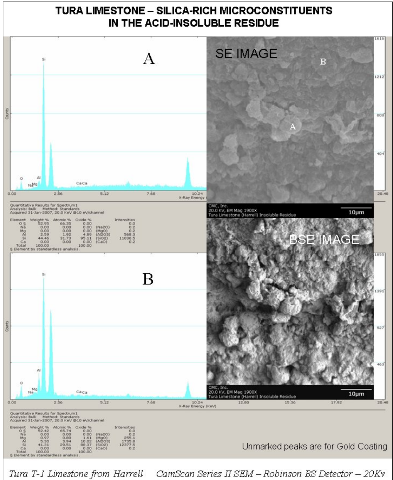
Figure 23: Acid-insoluble residue of Tura limestone showing the silica-rich composition and somewhat distorted microspheres with rougher surfaces (probably due to acid etching) than those detected in the previous photos in the bulk sample All these silica-rich microspheres in a natural limestone also contain noticeable amounts of alumina as impurity and certainly do not indicate an aluminosilicate precipitate from a geopolymeric matrix (Davidovits 2005).
