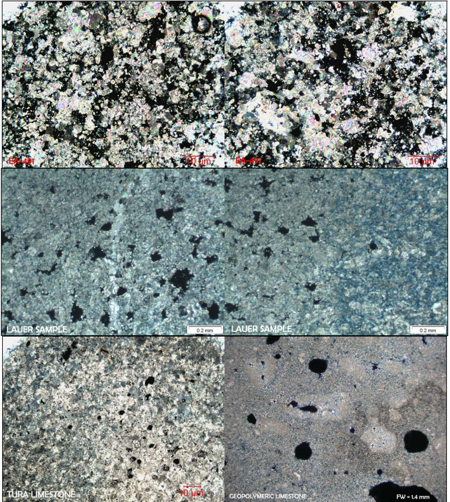
Figure 4: Photomicrographs of thin sections of casing stones (EA-491 and the Lauer sample), Tura limestone, and geopolymeric limestone showing intergranular pore spaces in EA-491, irregularly shaped voids in the Lauer sample, very fine voids and pores in Tura limestone and characteristic near-spherical and spherical voids in geopolymeric limestone. FW (Field Width) is the distance from left to right of a photo.
