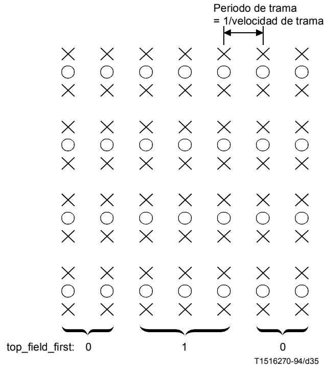
Figura 7-19 – progressive_sequence == 1, repeat_first_field == 1
