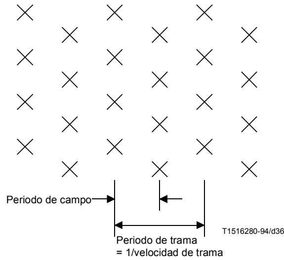
Figura 7-20 – progressive_sequence == 0
