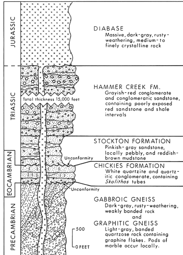
Geologic column.
