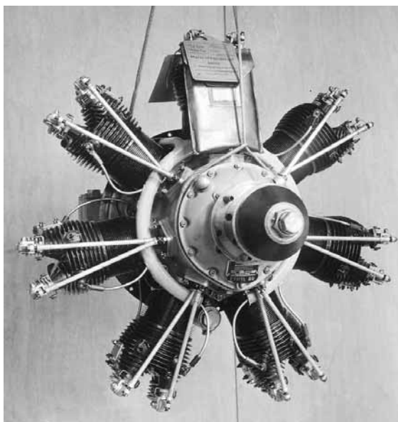
Siemens Sh-14: 160PS. (Bücker Jungmeister)
