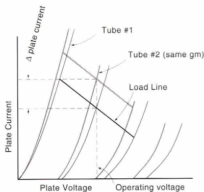
Figure 3 Same gm, different current
