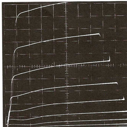
Figure 5 GE 7581A/KT66
