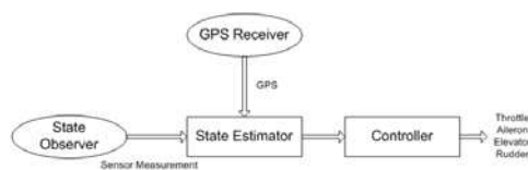
Fig. 2. Functional Structure of the UAV Autopilot.
