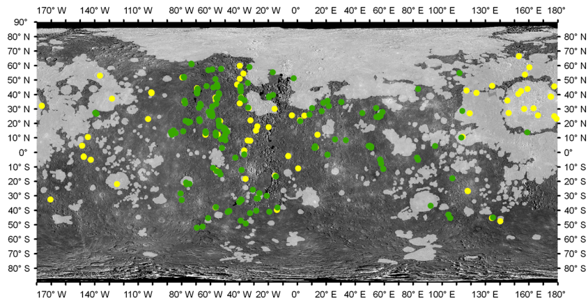
Figure 17. Locations of hollows on Mercury. Yellow dots show the locations of hollows mapped by Blewett et al. [2011]. Green dots are additional hollows identified from MESSANGER orbital images. The shaded light grey areas are smooth plains units mapped by Denevi et al. [2012]. Because of the spacecraft’s highly eccentric orbit, images have better spatial resolution in the northern hemisphere, making identification of hollows easier there. The base image is a global MDIS monochrome mosaic in equirectangular projection.
