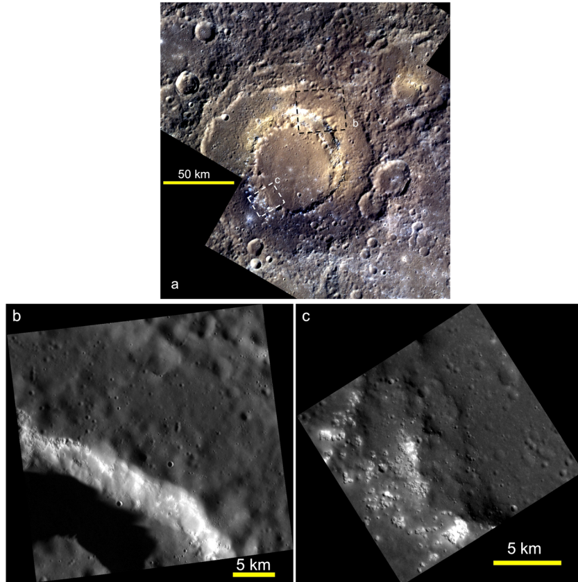
Figure 14. Hollows and pyroclastic material within Scarlatti crater (132 km diameter, 40.8°N, 258.8°E). (a) Color composite mosaic at wavelengths of 996, 749, and 433 nm as RGB. Images EW0242045882I, EW0242004051I, EW0242045874G, EW0242004043G, EW0242045878F, EW0242004047F, 202 m/pixel. Dashed boxes indicate the areas of high-resolution images in Figures 14b and 14c. Reddish pyroclastic material has mantled much of the northern half of the crater. A large, elongated, vent-like depression has replaced the northern portion of the peak ring. Hollows are found within dark, blue material that forms Scarlatti's peak ring and the area between the peak ring and the southern rim. LRM is also found to the north and east of Scarlatti. (b) High-resolution targeted NAC view of a section of the large vent seen in Figure 14a. Image EN0231821310M, 29 m/pixel. Hollows are developed in the rim and walls of the vent. (c) Hollows on the southern peak ring. Targeted NAC image EN0244488176M, 14 m/pixel.
