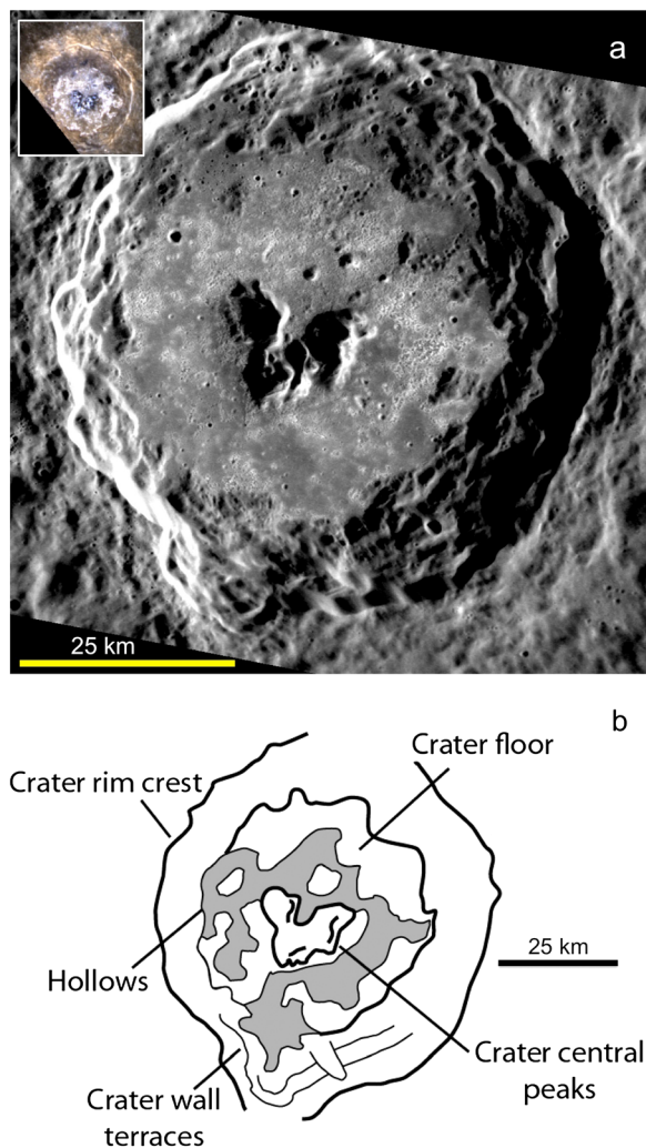
Figure 3. (a) Crater de Graft, exhibiting coalesced hollows (“etched terrain”) on its floor. The crater is 68 km in diameter and centered at 22.1°N, 2.0°E. Targeted monochrome image EN0220761681M, 73 m/pixel. Inset is a red-green-blue composite of images taken through the filters at 996, 749, and 433 nm wavelength (EW0225143097I, EW0225143117G, and EW0225143101F; see also Figure 21). (b) Geologic sketch map of the major features in de Graft.
