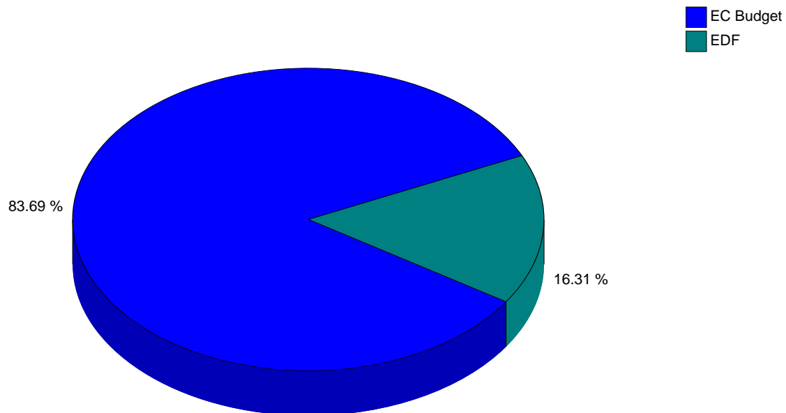
Budget/EDF breakdown - 2005
