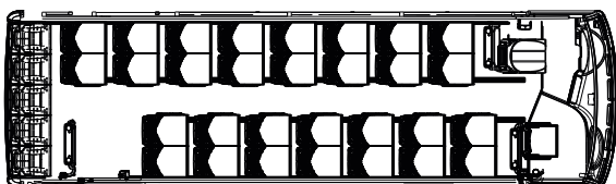
35 SEATED + 1 HOSTESS SEAT
