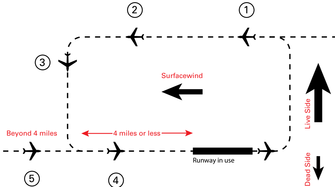
Figure 1 Designated Positions in the Traffic Circuit
