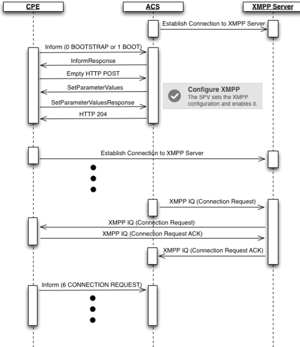
Figure 18 – XMPP Connection Request Message Sequence
