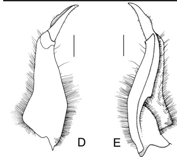
Fig. 5. Eosamon smithianum (Kemp, 1923). Male (53.3 × 42.6 mm) (CUMZ): A, dorsal view; B, frontal view of carapace; C, ventral view of carapace; D, E, left G1. Scale bars: 2.0 mm.
