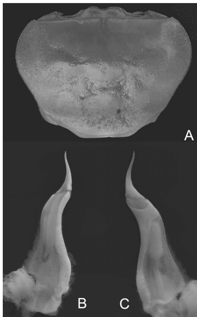
Fig. 18. Villopotamon thaili Dang & Ho, 2003. Holotype, male (54.5 × 40.2 mm) (ZMH): A, dorsal view; B, C, left G1.
