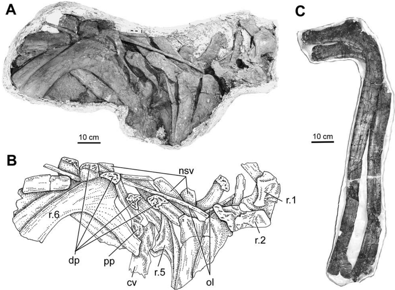
Fig. 13. Some vertebrae and ribs of Eotriceratops xerinsularis . cv, centrum of vertebra; dp, diapophysis of vertebrae; nsv, neural spine of vertebrae; ol, ossified ligament; pp, parapophysis; r.1, r.2, r.5, and r.6, ribs 1, 2, 5, and 6, respectively, reserved in the vertebral series.
