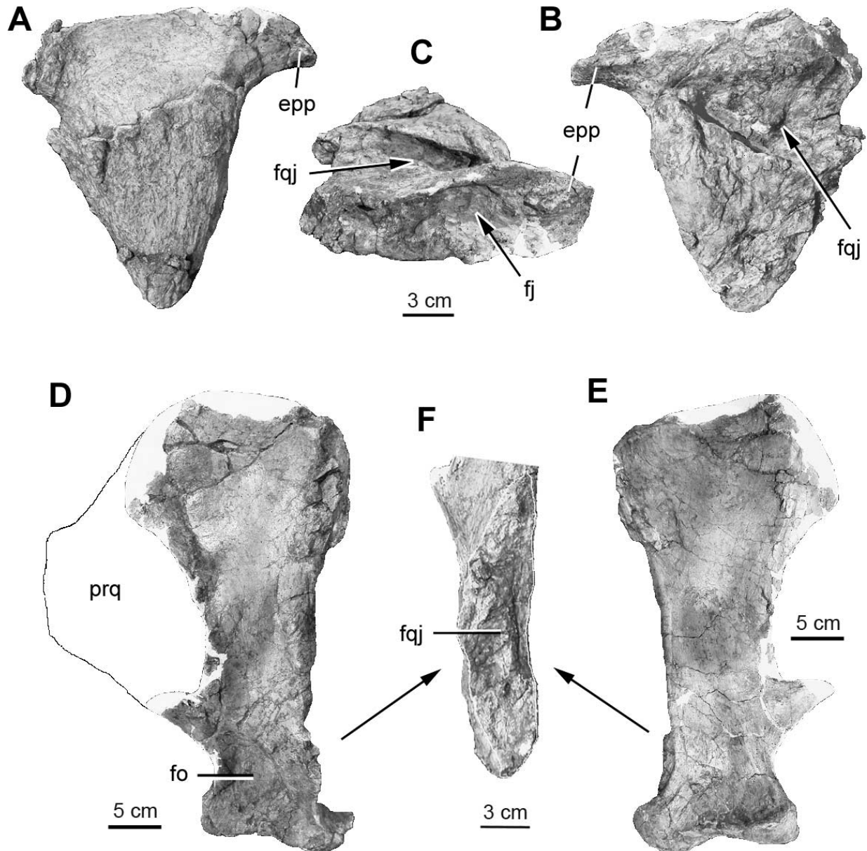
Fig. 9. Left epijugal and left quadrate of Eotriceratops xerinsularis . Left epijugal in lateral (A), medial (B), and dorsomedial (C) views. Left quadrate in posterior (D), anterolateral (F, lower half), and anterior (E) views. epp, proximoposterior process of epijugal; fj, facet for jugal; fo, fossa; fqj, facet for quadratojugal; prq, pterygoid ramus of quadrate.
