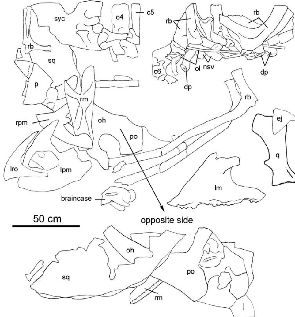
Fig. 2. Spatial arrangement of preserved elements of Eotriceratops xerinsularis showing the distorted preservational state of the specimen. c4, c5, and c6, cervical vertebrae 4, 5, and 6, respectively; dp, diapophysis of vertebrae; ej, epijugal; j, jugal; lm, left maxilla; lpm, left premaxilla; lro, left rostrum; nsv, neural spine of vertebrae; oh, orbital horn core; ol, ossified ligament; p, parietal; po, postorbital; q, quadrate; rb, rib; rm, right maxilla; rpm, right premaxilla; sq, squamosal; syc, syncervical vertebrae.
