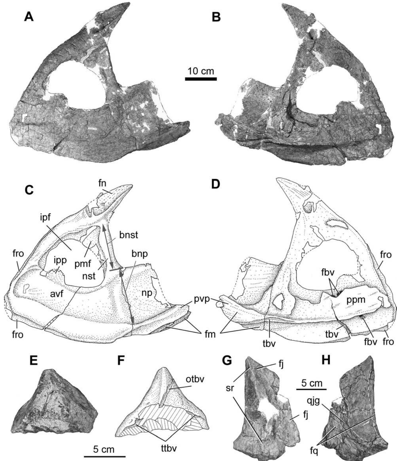
Fig. 6. Some skull elements of Eotriceratops xerinsularis . (A, C) Left premaxilla in lateral views. (B, D) Left premaxilla in medial views. (E, F) Nasal horn core in slightly different anterior views. (G, H) Right quadratojugal in lateral and medial views, respectively. avf, fossa or recess anteroventral to the interpremaxillary fenestra; bnp, dorsoventral breadth of narial process; bnst, dorsoventral breadth of narial strut; fbv, foramen for blood vessels and nerves; fj, facet for jugal; fm, facet for maxilla; fn, facet for nasal; fq, facet for quadrate; fro, facet for rostrum; ipf, interpremaxillary fenestra; ipp, interpremaxillary process; np, narial process; nst, narial strut; otbv, oblique trace for blood vessels; pmf, premaxillary fossa; ppm, palatal portion of maxilla; pvp, posteroventral process; qjg, quadratojugal groove; sr, swollen ridge; tbv, trace for blood vessels and nerves; ttbv, transverse trace for blood vessels.
