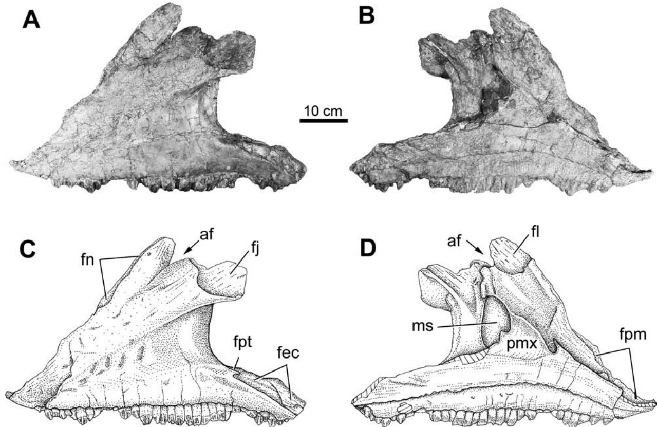
Fig. 7. Left maxilla of Eotriceratops xerinsularis in lateral (A, C) and medial (B, D) views. af, antorbital fenestra; fec, facet for ectopterygoid; fj, facet for jugal; fl, facet for lacrimal; fn, facet for nasal; fpm, facet for premaxilla; fpt; facet for pterygoid; ms, maxillary sinus; pmx, palatal portion of maxilla.
