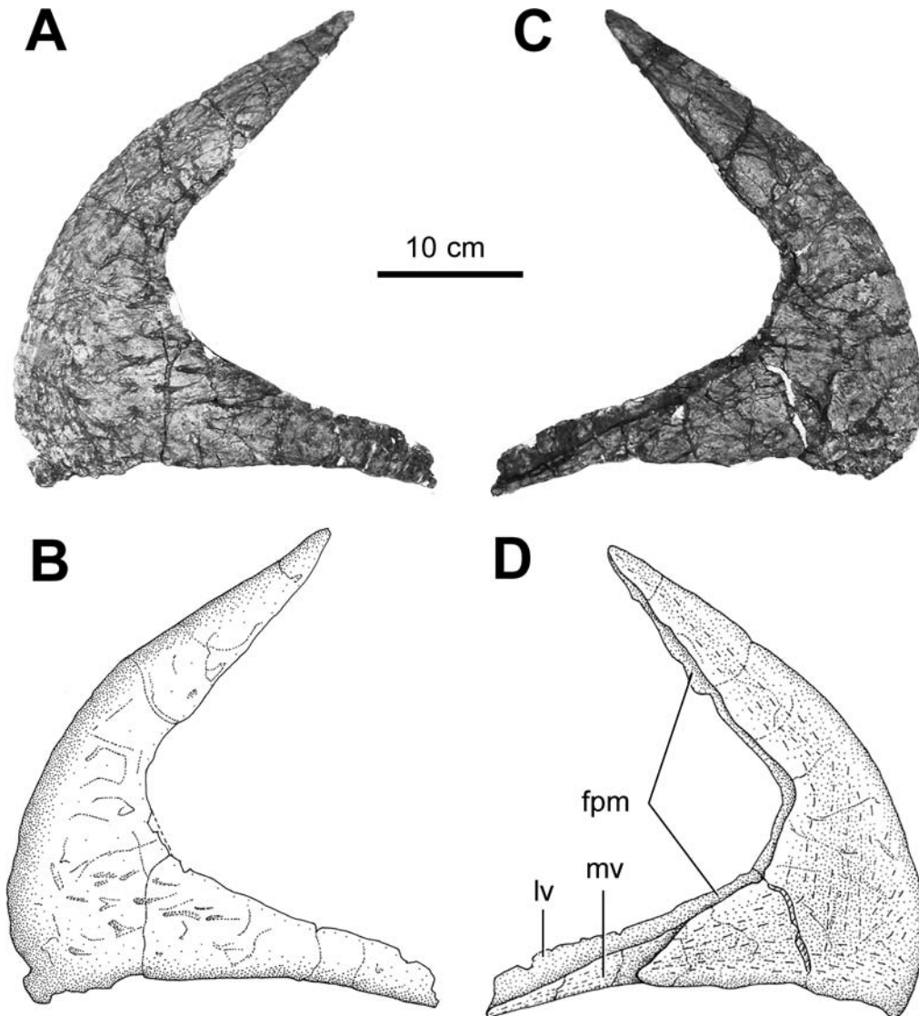
Fig. 5. Left rostrum of Eotriceratops xerinsularis in lateral (A, B) and medial (C, D) views. fpm, facet for premaxilla; lv, lateral portion of ventral ramus; mv, medial portion of ventral ramus.
