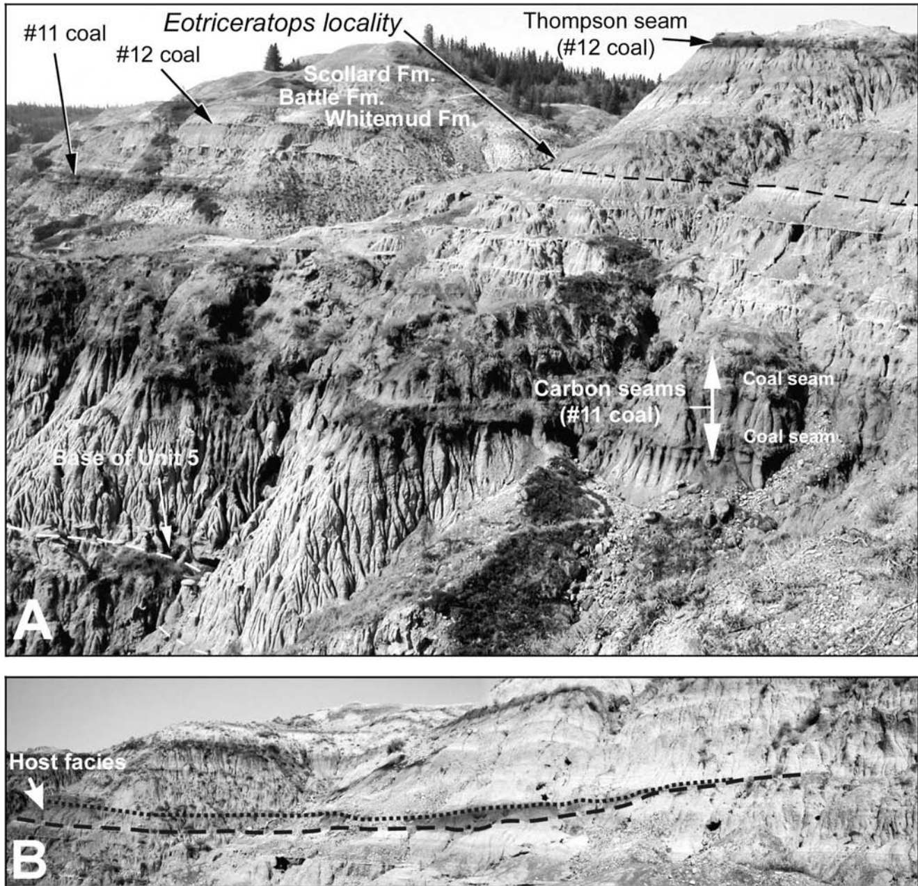
Fig. 4. Location, stratigraphic position, and facies association of Eotriceratops xerinsularis . (A) Specimen occurs between the Carbon and Thompson coal zones, 9 m above the base of the Carbon zone (a double seam) and 13.5 m above the base of unit 5 (here marked by the base of a fine-to-medium grained sandstone body). (B) Specimen occurs near the base of a broadly lenticular (tens of metres wide), dark red-brown, silty, carbonaceous shale that is up to 50 cm thick. Carbonaceous shale is sharp based to erosional, and exhibits patchy, irregular ironstone nodules, and local sulfur staining.
