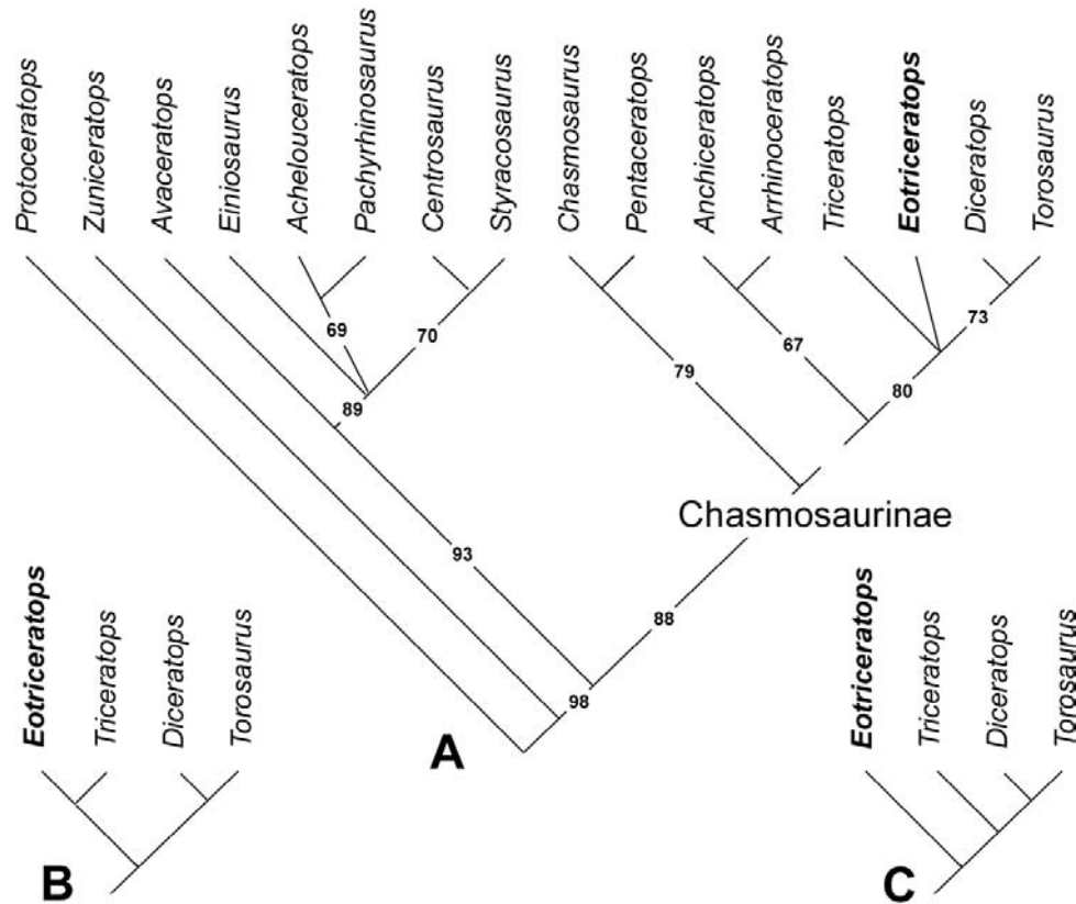
Fig. 14. Cladograms showing phylogenetic relationships of Eotriceratops . (A) Strict consensus tree computed from the six most parsimonious trees (MPTs) recovered by PAUP* analysis of a modified version of the character–taxon matrix by Dodson et al. (2004). (B, C) Alternative relationships of Eotriceratops with crown taxa among the six most parsimonious trees. Nodal numbers indicate bootstrap proportions based on 1 000 replicates using the branch and brand algorithm in PAUP*.
