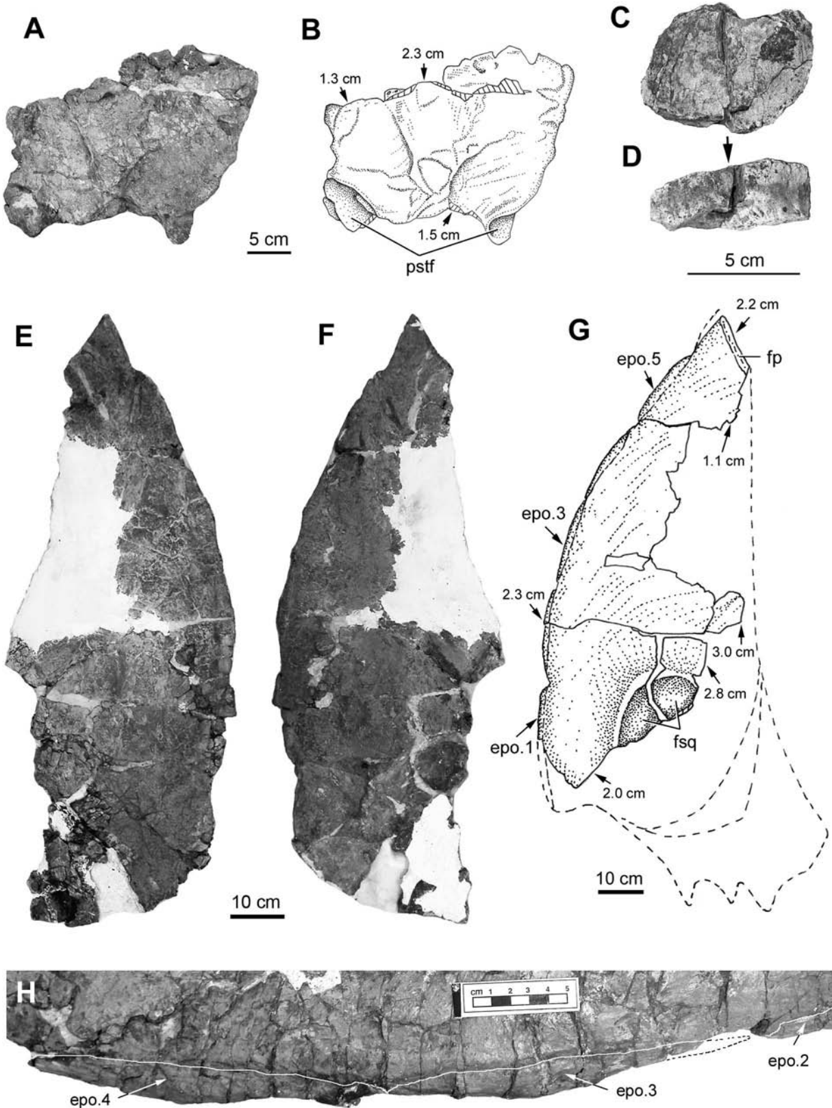
Fig. 10. Frill fragments of Eotriceratops xerinsularis . (A, B) Anterior part of parietal frill in dorsal views. (C, D) A piece of parietal frill in dorsal and cross-section view, respectively. (E–G) Partial squamosal frill in dorsal (E) and ventral (F, G (a reconstruction)) views. (H) lateral edge of squamosal. epo.1–epo.5, epoccipitals 1–5, respectively; fp, sutural facet for parietal frill; fsq, fossa on ventral surface of squamosal frill; pstf, parietal portion of supratemporal fenestra; 1.1 cm, 1.3 cm, 1.5 cm... indicate, respectively, number of centimetre thicknesses of bone in areas shown by arrows.
