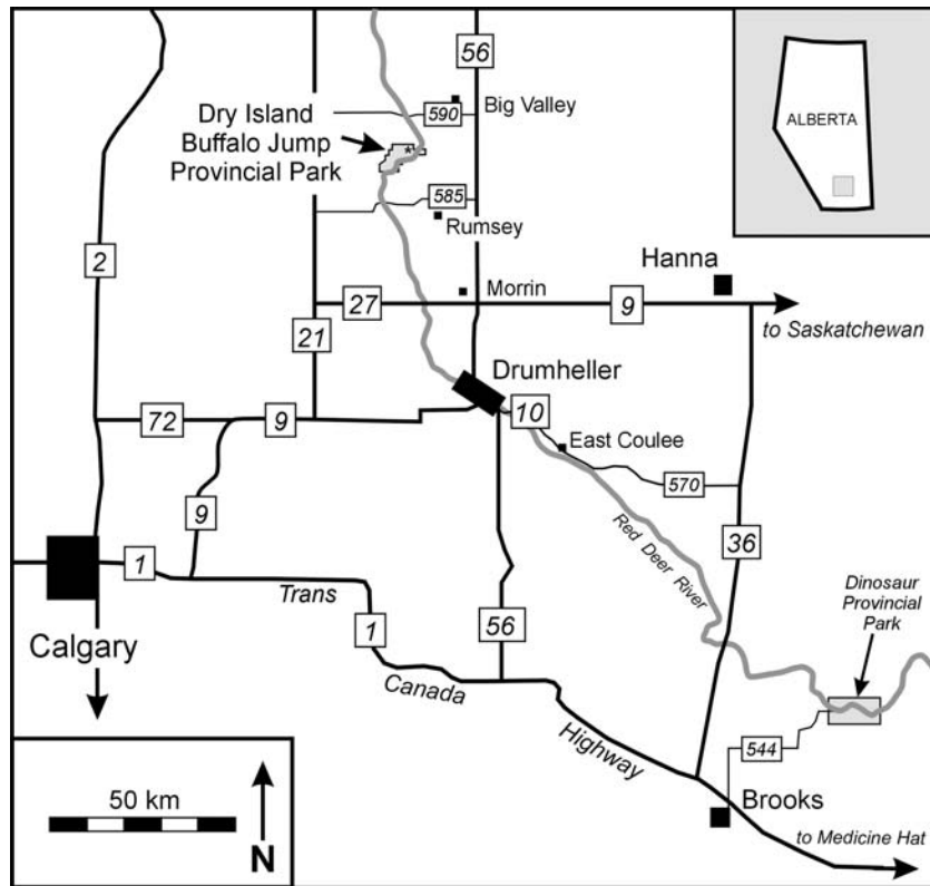
Fig. 1. Locality map for Eotriceratops insularis . The specimen locality is indicated by an asterisk in the northeast portion of Dry Island Buffalo Jump Provincial Park. More detailed locality information is available from the Royal Tyrrell Museum, Collections Section. Upper right inset shows field area in relation to the Province of Alberta.
