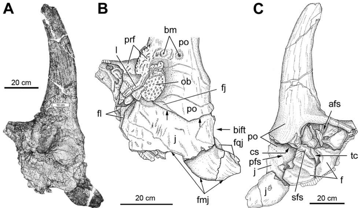
Fig. 8. Supraorbital horn core and bones around orbit of Eotriceratops xerinsularis in lateral (A, B) and medial views. asf, anterior frontal sinus; bift, border of infratemporal fenestra; bm, bite marks; cs, conual sinus; f, frontal; fj, facet for jugal; fl, facet for lacrimal; fmj, free margin of jugal flange; fqj, facet for quadratojugal; j, jugal; l, lacrimal; ob, orbit; pfs, posterior frontal sinus; po, postorbital; prf, prefrontal; sfs, septum of frontal sinus; tc, trace of canal. Two arrows below the postorbital–jugal suture indicate that the jugal was pushed upward underneath the postorbital during preservation.
