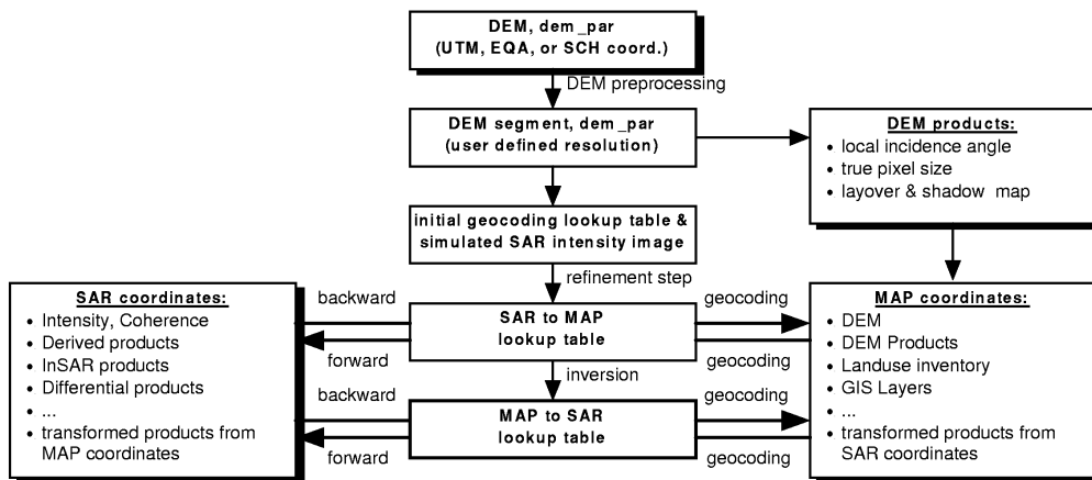
Figure 10. GAMMA DIFF&GEO Software: Geocoding Flow Chart
