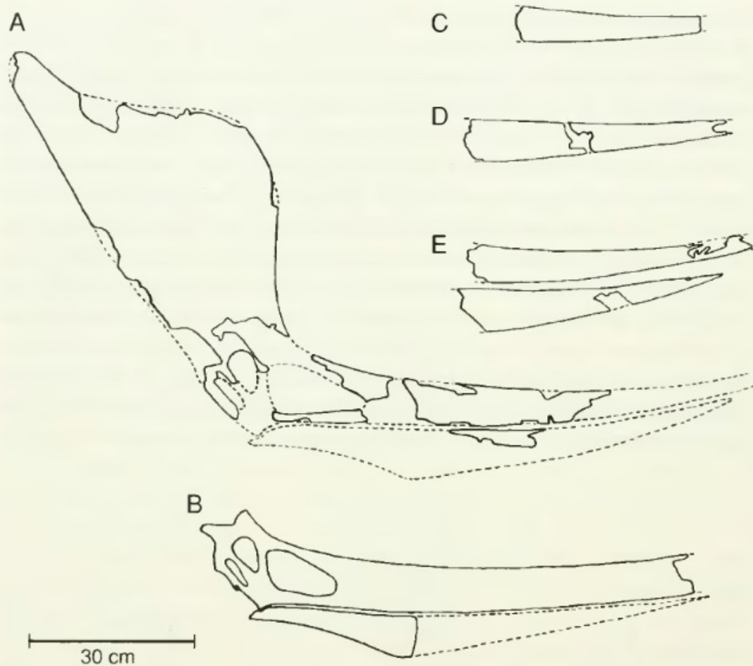
Fig. 2. Cranial crests of Pteranodon sternbergi and jaws of Pteranodon . A , FHSM VP 339 (left lateral view reversed). B , UALVP 24238. C , YPM 2489. D , AMNH 1974 (left lateral view reversed). E , KUV 967. A and B are P. sternbergi ; C and E are P. longiceps ; and D is Pteranodon sp. indet.
