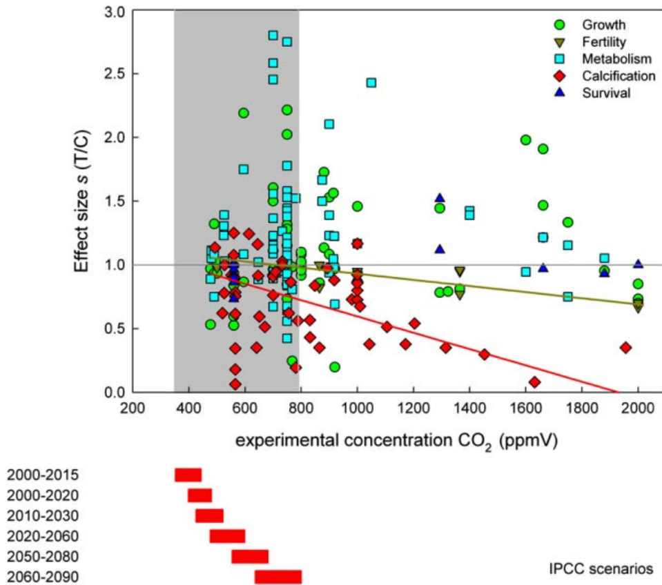
Figure 8: The relationship between the effect size, s (treatment/control), of biological responses, assessed by different processes, to experimental \text{CO}_2 concentration manipulation over the range 477–2000ppm \text{CO}_2 . If s < 1 , then acidification has a negative impact, and if s > 1 then acidification has a positive impact. The shaded area and lower part of the graph shows the future \text{CO}_2 values projected under different IPCC scenarios. Source: Hendriks et al. (2010), p. 162.
