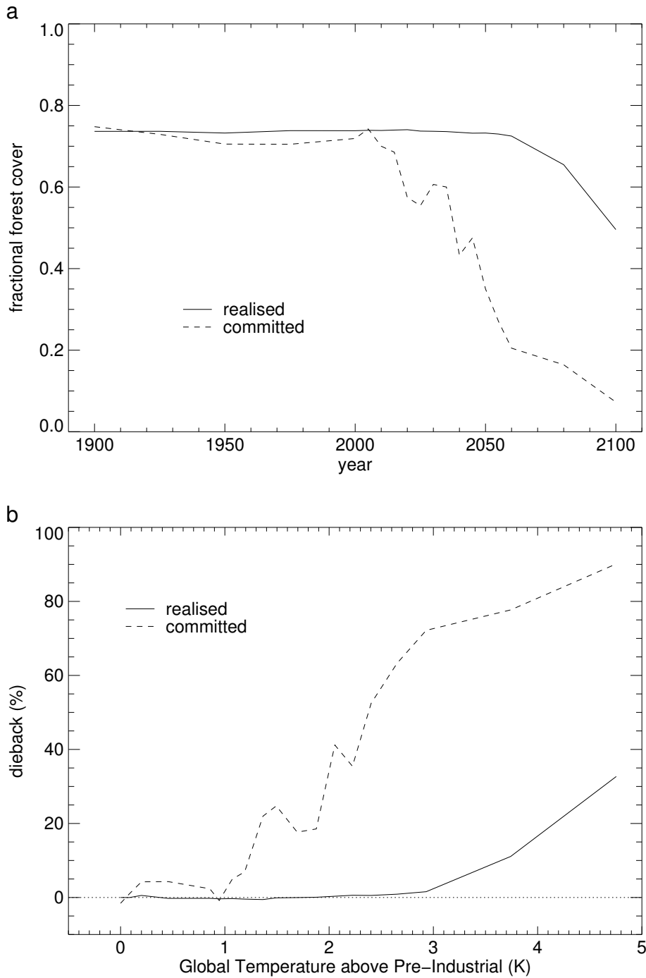
Figure 4: (a) Fractional tree cover (represented as fractional coverage of broadleaf trees in the region 40^{\circ} – 70^{\circ} W, 15^{\circ} S– 5^{\circ} N) as it evolves dynamically through the SRES A2 simulation and the committed state corresponding to each year. (b) The same information plotted as the percentage of complete die-back as a function of global mean temperature rise above pre-industrial (defined as 0 for the original, pre-industrial forest cover, and 100 for complete loss of tree cover in this region). Source: Jones et al. (2009).
