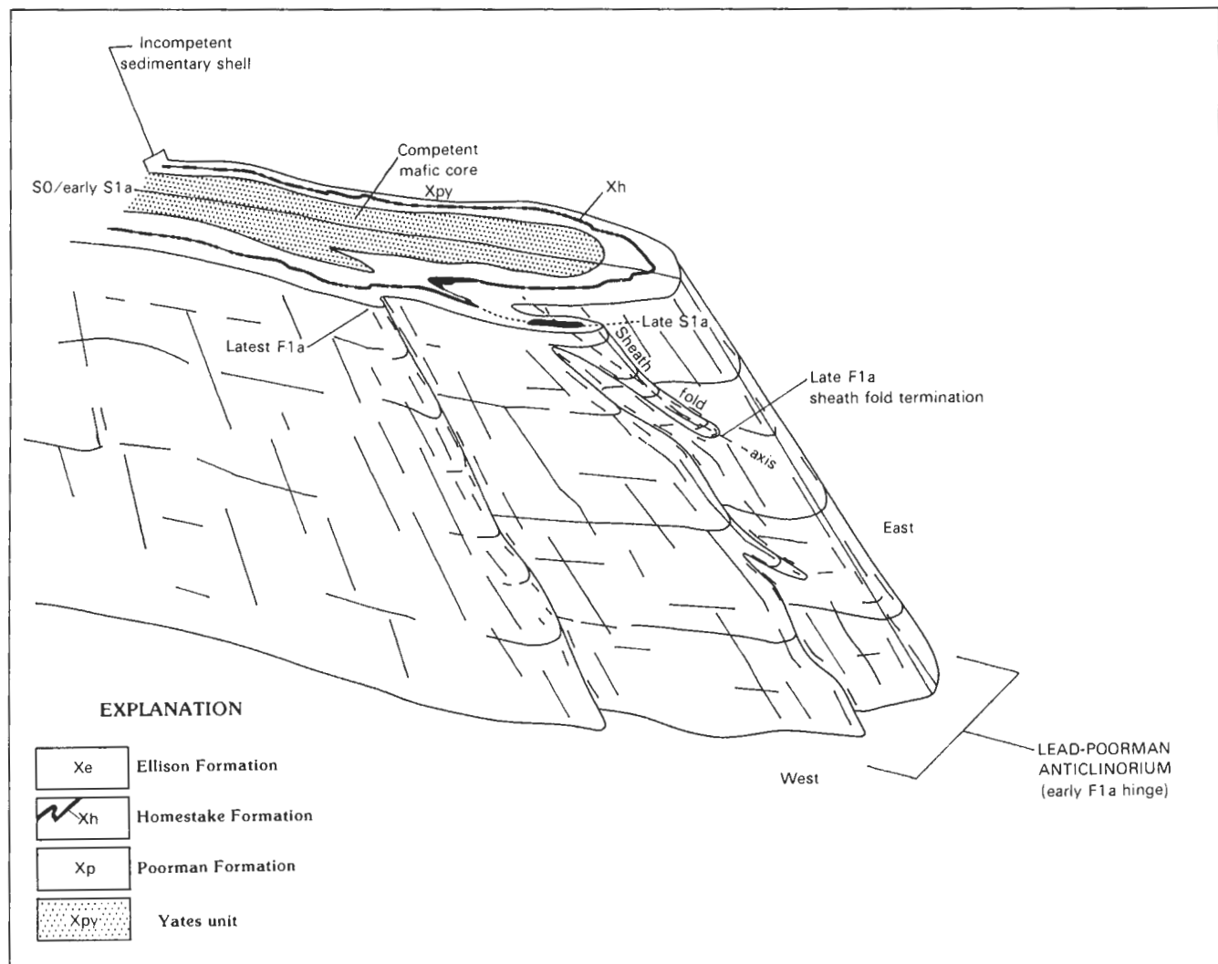
Figure J16. Schematic perspective diagram showing D1a fold events at Homestake mine.
