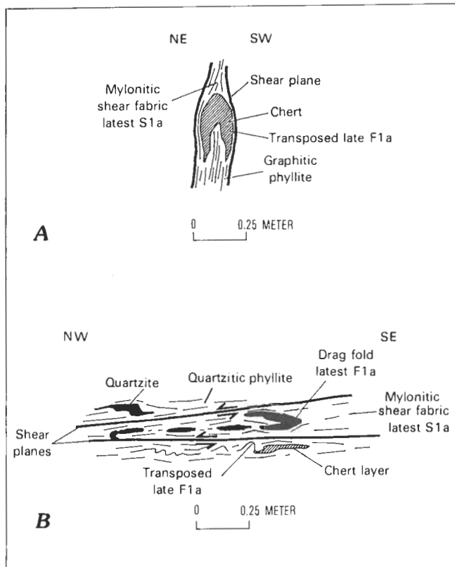
Figure J20. Structural sketches in profile sections of minor folds in latest D1a shear zones, western ledge area on the Poorman anticline, Homestake mine. A , Poorman Formation; floating, detached fold hinge. B , Ellison Formation; disharmonic reclined drag folds. Single-barb arrows show direction of shear.
