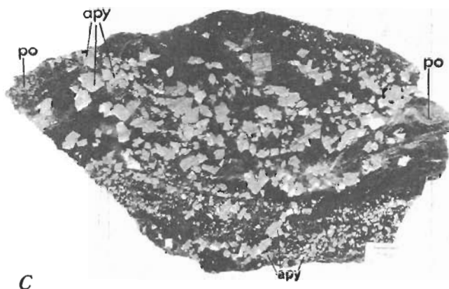
Figure J33. Photographs of typical ore specimens, Homestake mine; po, pyrrhotite; apy, arsenopyrite; v.g., coarse visible gold. A , Pyrrhotite blebs in grunerite- and siderite-rich layers interbedded with thin chert beds from drill core in a 15 Ledge ore body, 8000 level. Minor chlorite is present in the grunerite- and siderite-rich strata. Two small grains of coarse visible gold border irregular pyrrhotite blebs. A 2 m interval assayed 37.3 g Au/t. Modal sulfide contents are 8 percent pyrrhotite, <<1 percent coarse gold, and <<1 percent arsenopyrite. B , Typical layered pyrrhotite (some disseminations and blebs) interlayered with biotite-rich chert and siderite in an ore body in 21 Ledge, 7400 level. Thin layers that enclose thinner pyrrhotite layers contain minor chlorite, and are locally replaced by isolated arsenopyrite porphyroblasts. This layered texture is restricted to ore bodies. Two single grains of coarse visible gold occur within two pyrrhotite layers. Modal sulfide contents are 12–14 percent pyrrhotite, <1 percent arsenopyrite, and <<1 percent coarse visible gold. C , Coarse-grained arsenopyrite within a chlorite-rich siderite matrix from an ore body in 7 Ledge, 1550 level. Specimen came from a 2.0-m-wide Stage II quartz-vein selvage within which coarse visible gold is present locally. The gold borders and is within arsenopyrite porphyroblasts, and is enclosed as isolated platy grains in chlorite. This ore is typically of exceptional grade and averages >16.0 g Au/t. Modal sulfide contents are 15–20 percent arsenopyrite and <1 percent pyrrhotite.
