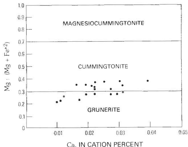
Figure J7. Plot of Mg:(Mg+Fe^{+2}) versus Ca (cation percent) for selected grunerite-cummingtonite-series amphiboles from the Homestake mine. Petrographic studies of amphiboles in iron-formation across the mine show that grunerite composition is most abundant. Diagram modified from Leake (1978); data from T.J. Campbell (unpublished Homestake report).
