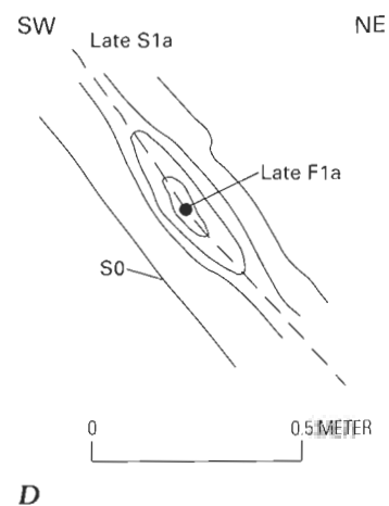
Figure J19. Sketches of late F1a (sheath) and early F1b minor folds in Poorman and Ellison Formations in the eastern ledge area of the Lead anticline, Homestake mine. A , typical late F1a fold in profile section; B , meso-scale late F1a-early F1b refolded combination in profile section; C , late F1a-early F1b refolded combination in plan view—this style of fold interference is seen at all scales; D , meso-scale late F1a sheath fold termination in profile section. Profile sections viewed up plunge along the fold-axis direction.
