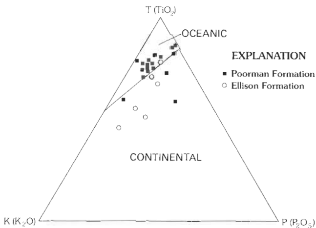
Figure J10. KTP diagram for metabasalt samples from the Poorman Formation (Yates unit) and Ellison Formation, Homestake mine. Field boundary from Pearce and others (1975).
