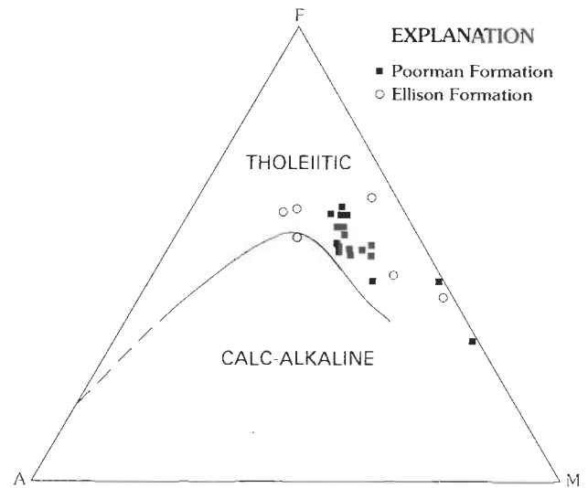
Figure J9. AFM diagram for metabasalt samples from the Poorman Formation (Yates unit) and Ellison Formation, Homestake mine. Field boundaries from Irvine and Baragar (1971).
