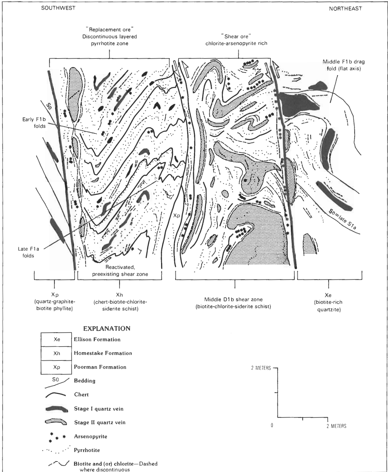
Figure J29. Face sketch, 7 Ledge, 1550 level, 58-61 stope, Homestake mine. Near-vertical line, shear; heavy line, major shear; bars show relative movement.
