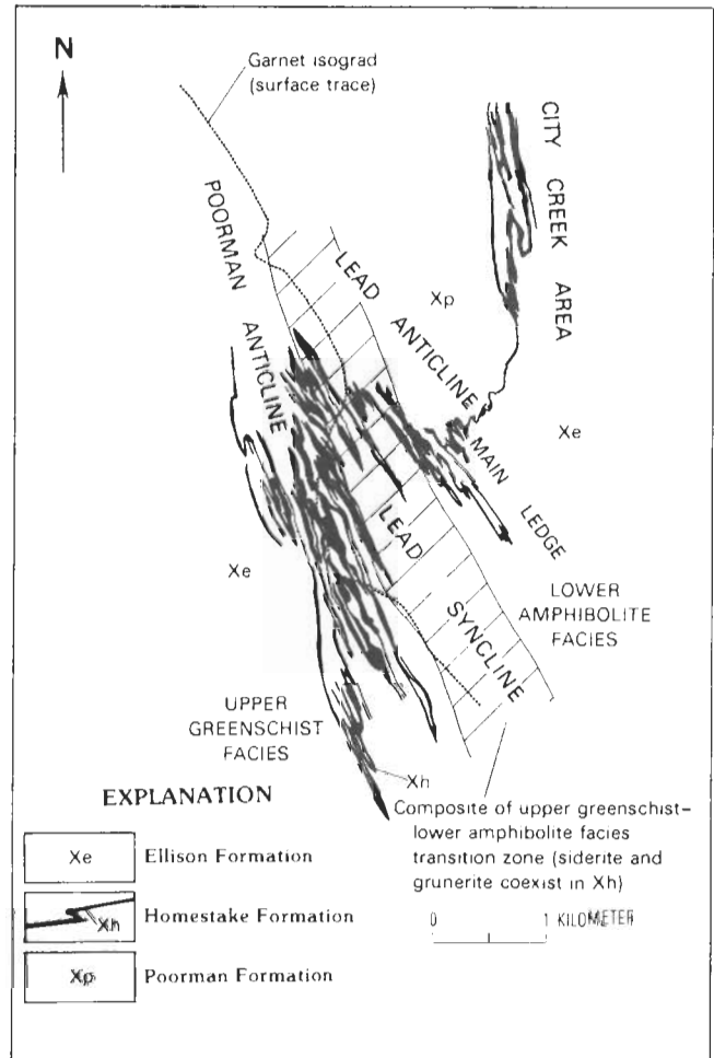
Figure J11. Geology of 2600 level, Homestake mine, showing upper greenschist–lower amphibolite facies and ground surface trace of garnet isograd.
