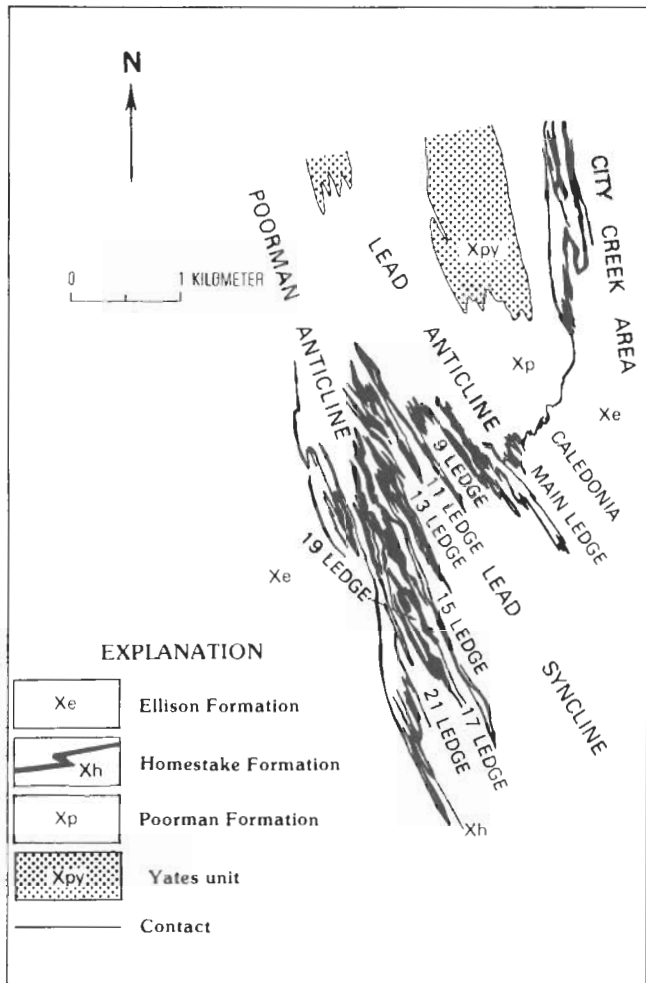
Figure J6. Geology of 2600 level of the Homestake mine, showing significant fold structures and ore ledges.
