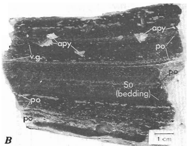
Figure J33. Photographs of typical ore specimens, Homestake mine; po, pyrrhotite; apy, arsenopyrite; v.g., coarse visible gold. A , Pyrrhotite blebs in grunerite- and siderite-rich layers interbedded with thin chert beds from drill core in a 15 Ledge ore body, 8000 level. Minor chlorite is present in the grunerite- and siderite-rich strata. Two small grains of coarse visible gold border irregular pyrrhotite blebs. A 2 m interval assayed 37.3 g Au/t. Modal sulfide contents are 8 percent pyrrhotite, <<1 percent coarse gold, and <<1 percent arsenopyrite. B , Typical layered pyrrhotite (some disseminations and blebs) interlayered with biotite-rich chert and siderite in an ore body in 21 Ledge, 7400 level. Thin layers that enclose thinner pyrrhotite layers contain minor chlorite, and are locally replaced by isolated arsenopyrite porphyroblasts. This layered texture is restricted to ore bodies. Two single grains of coarse visible gold occur within two pyrrhotite layers. Modal sulfide contents are 12–14 percent pyrrhotite, <1 percent arsenopyrite, and <<1 percent coarse visible gold. C , Coarse-grained arsenopyrite within a chlorite-rich siderite matrix from an ore body in 7 Ledge, 1550 level. Specimen came from a 2.0-m-wide Stage II quartz-vein selvage within which coarse visible gold is present locally. The gold borders and is within arsenopyrite porphyroblasts, and is enclosed as isolated platy grains in chlorite. This ore is typically of exceptional grade and averages >16.0 g Au/t. Modal sulfide contents are 15–20 percent arsenopyrite and <1 percent pyrrhotite.
