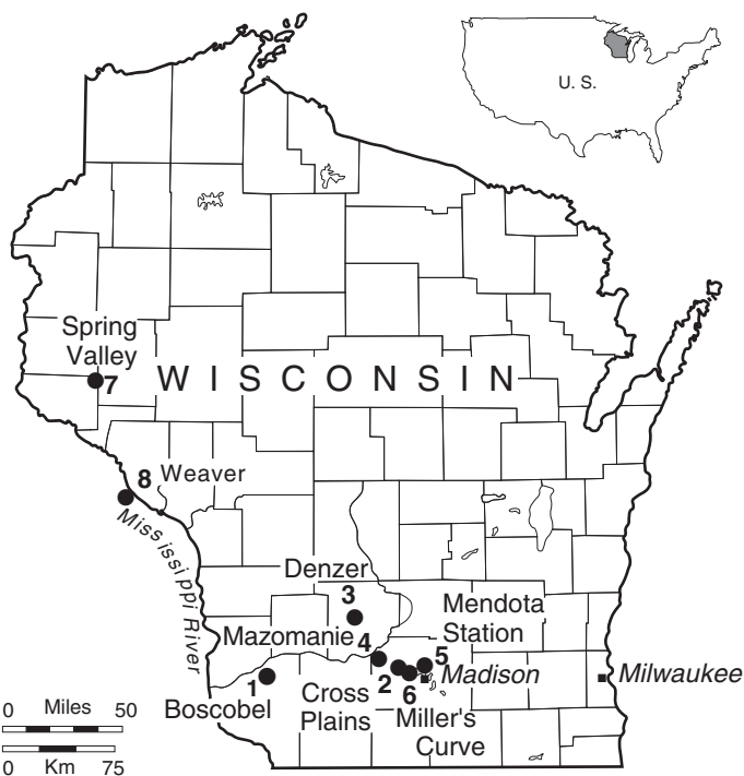
Figure 2. Jordan–Oneota boundary sections studied. 1. Boscobel, SW \frac{1}{2} , NW \frac{1}{2} , section 21, T8N, R3W, Grant County, Wisconsin; 2. Cross Plains East, NW \frac{1}{2} , SW \frac{1}{2} , sec. 11, T7N, R7E, Dane County, Wisconsin; 3. Denzer, quarry approximately 0.5 mi SE of Denzer, north side of Highway C, NW \frac{1}{2} , SE \frac{1}{2} , sec. 14, T10N, R5E, Sauk County, Wisconsin; 4. Mazomanie, approximately 3 mi SW of Mazomanie, south side of Highway K, NW \frac{1}{2} , NE \frac{1}{2} , sec. 31, T8N, R6E, Dane County, Wisconsin; 5. Mendota Station, railroad cut in center sec. 26, T8N, R9E, Dane County, Wisconsin; 6. Miller’s Curve, roadcut approximately 2.5 mi SE of Cross Plains, north side of Highway 14, SW \frac{1}{2} , SE \frac{1}{2} , section 7, T7N, R8E, Dane County, Wisconsin; 7. Spring Valley, approximately 0.25 mi north of Spring Valley, NW \frac{1}{2} , NW \frac{1}{2} , sec. 5, T27N, R15E, Pierce County, Wisconsin; 8. Weaver, SW \frac{1}{2} , SW \frac{1}{2} , sec. 30, T109N, R9W, Wabasha County, Minnesota.
