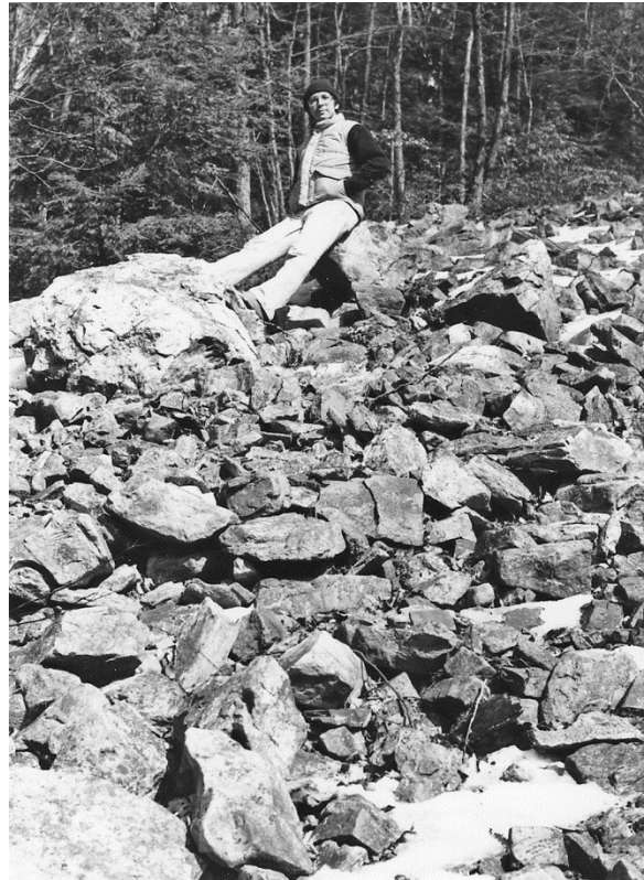
Scree in Rapid Run gap (Angular boulders are hard, quartzitic sandstone of Tuscarora Formation.)
