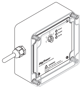
Figure 22: Ambient-sensing thermostats
