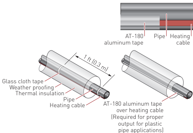
Figure 8: Attaching the heating cable
