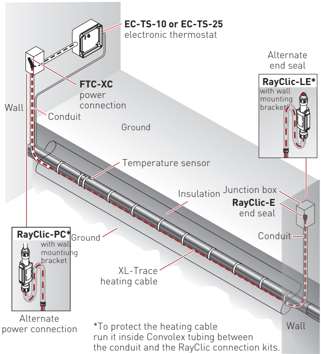
Figure 18: Buried pipe XL-Trace System
