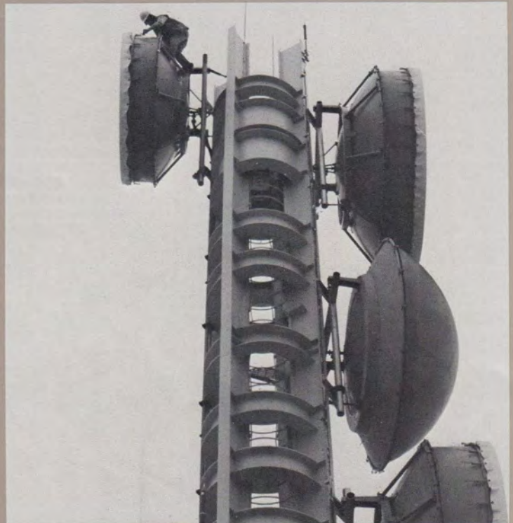
Below—Digital transmission systems were an increasingly important part of the network in the 70s. This unusual tower in Eugene, Oregon, was part of the first DR-6 digital system.
