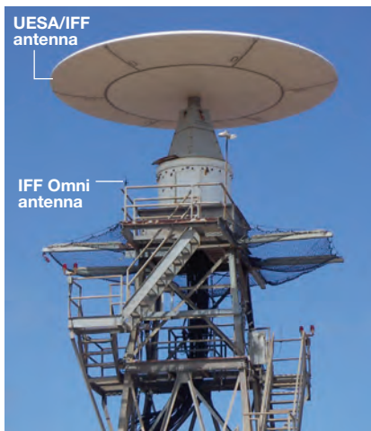
Figure 13-16 UESA/IFF circular array.
