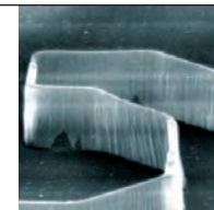
Silylation resist with 0.1 \mu\text{m} features
