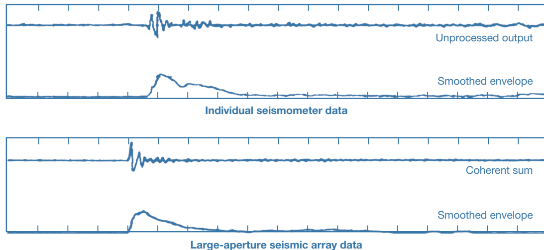
Figure 21-5 Presumed explosion in Kazakhstan, USSR.
