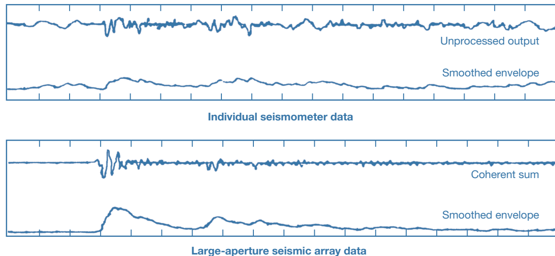
Figure 21-4 Earthquake near the Aleutian Rat Islands, November 11, 1965.
