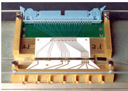
Figure 24-27 Lithium niobate ( \text{LiNbO}_3 ) 1-to-8 optical time-division demultiplexer used in the 10-bit 505 MS/s optically sampled A/D converter. One input fiber can be seen to the left of the \text{LiNbO}_3 , and eight output fibers are on the right side. The top face of the \text{LiNbO}_3 crystal is 7 cm \times 0.5 cm.
