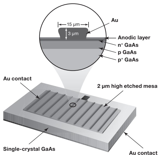
Figure 20-4 Schematic diagram of 20% efficient, 1.0 \times 0.5 cm GaAs shallow-homojunction solar cell with antireflection coating formed by anodic oxidation.
