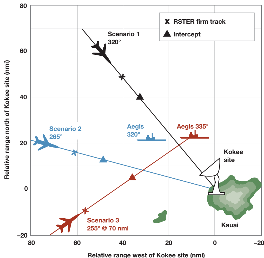
Figure 13-14 Cruise Missile Defense Advanced Concept live-fire demonstration.
