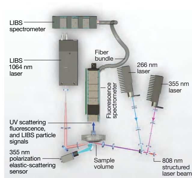
Figure 17-8 RAAD optics breadboard showing all laser sources and sensors.
