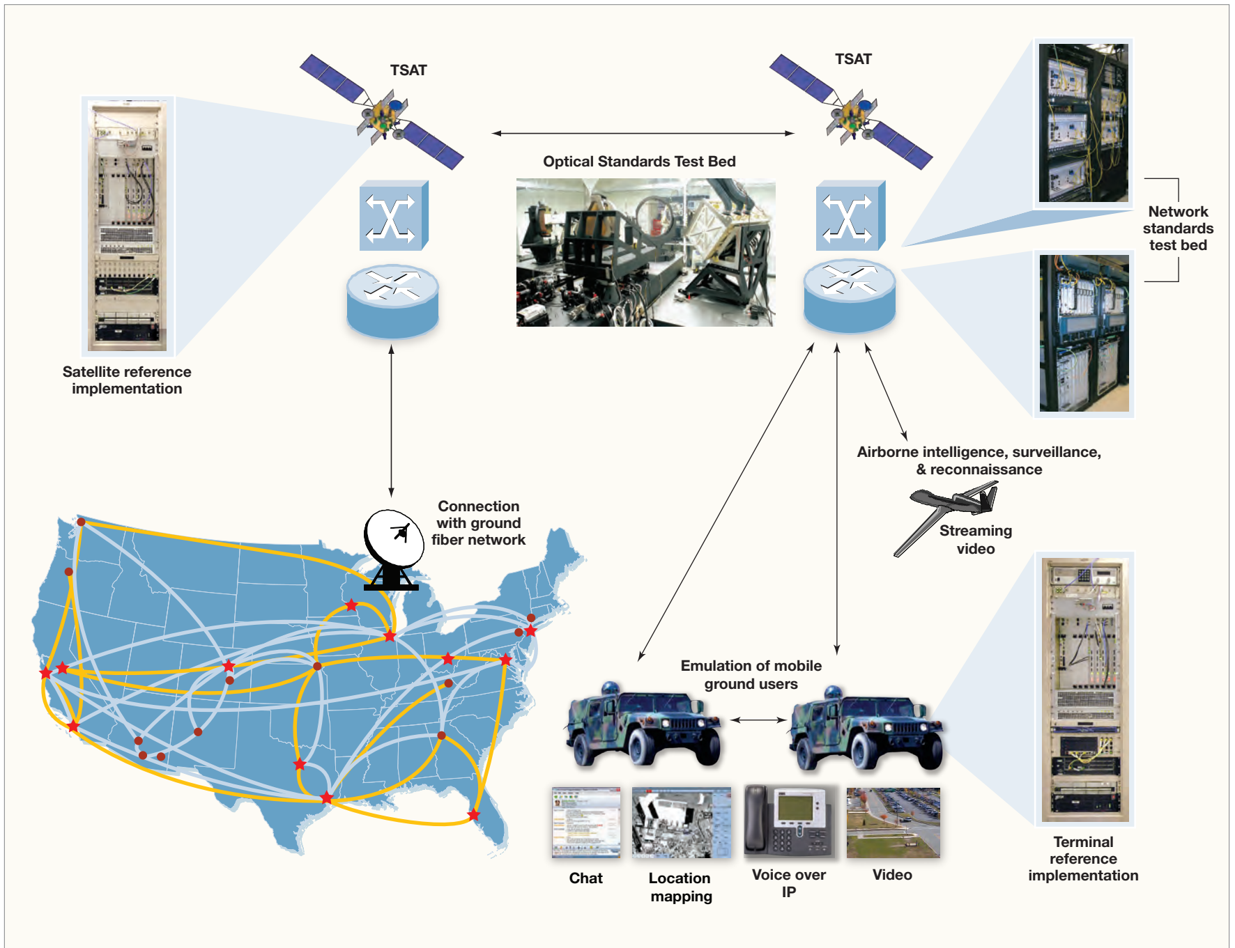
Figure 6-2 TSAT test bed concept.
