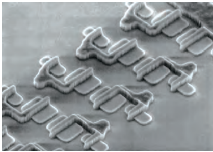
Figure 24-14 Scanning electron micrograph of the first functional electrical devices (ring oscillators) fabricated with the 193 nm system. The pitch of the inverter chain is 3.65 \mu\text{m} .
