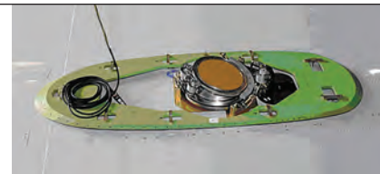
Advanced Multiband Communications Antenna used on Paul Revere for 2009 test flight
