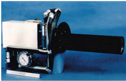
Figure 10-10 The 31-inch telescope camera and cold-shield assembly adapted for medium-wavelength infrared (1 to 5 \mu\text{m} ) satellite-tracking experiments.
