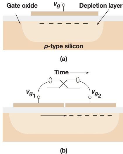
Figure 26-3 Illustration of CCD operation.
