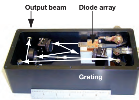
Figure 25-12 Compact, high-brightness 100-diode laser array implemented using wavelength beam combining.
