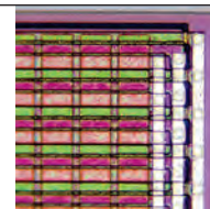
Corner of a CCD imager showing three (horizontal) gate levels per pixel and (vertical) aluminum clock busses
