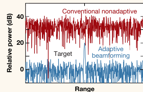
Figure 29-5 Radar receive beam output.
