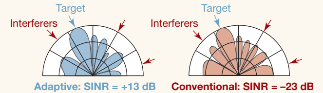
Figure 29-4 Receive beam responses as a function of signal arrival angle.
