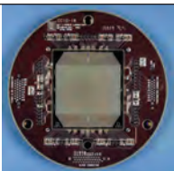
Full-wafer GEODSS 2560 × 1960-pixel imager on printed circuit board
