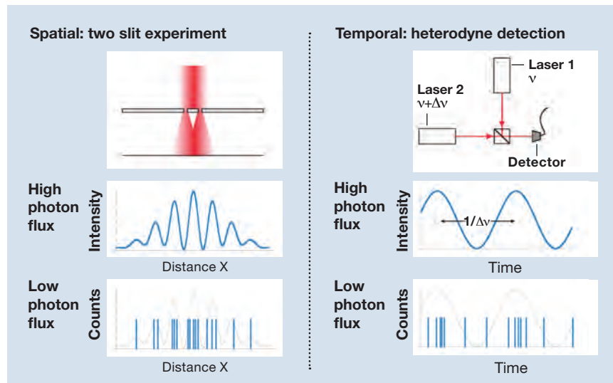
Figure 27-9 Photon-counting coherent detection.
