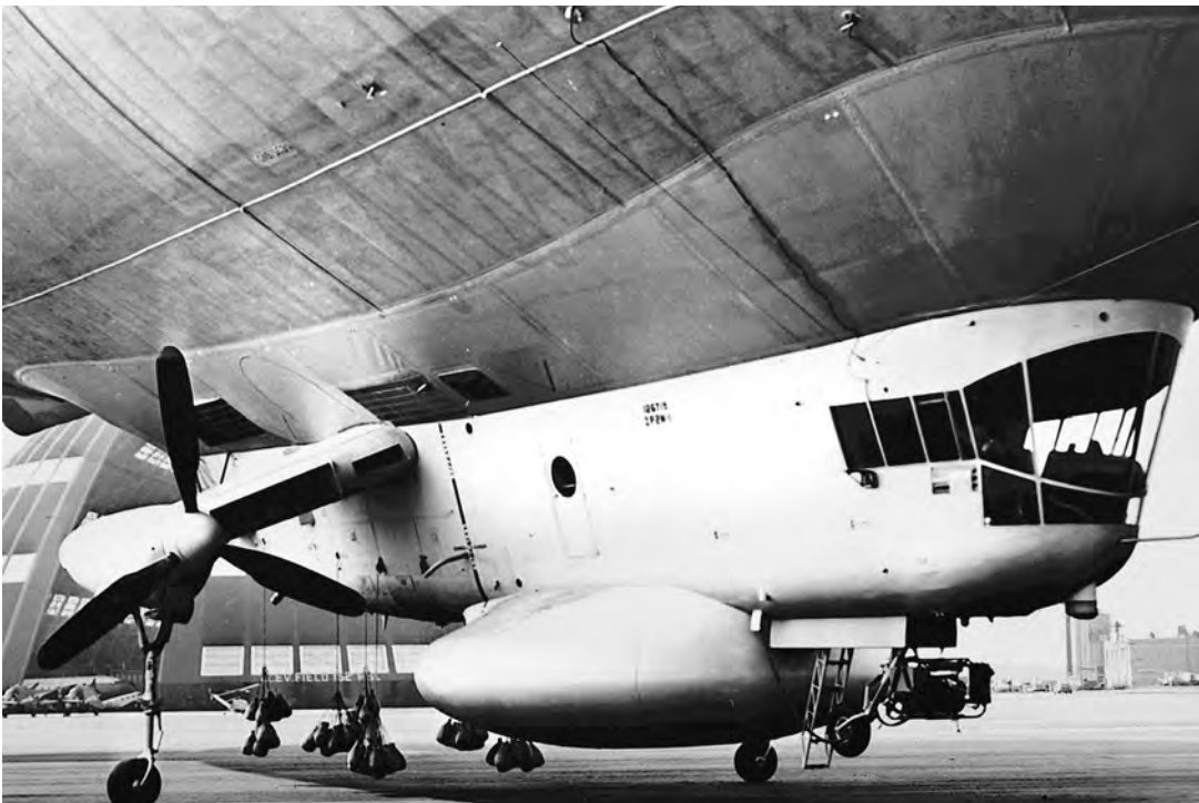
Figure 3-2 Navy blimp installation of the UHF AEW radar.
