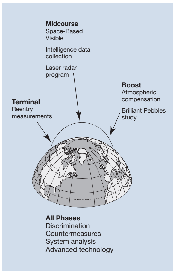
Figure 9-11 The three phases of ballistic missile flight.
