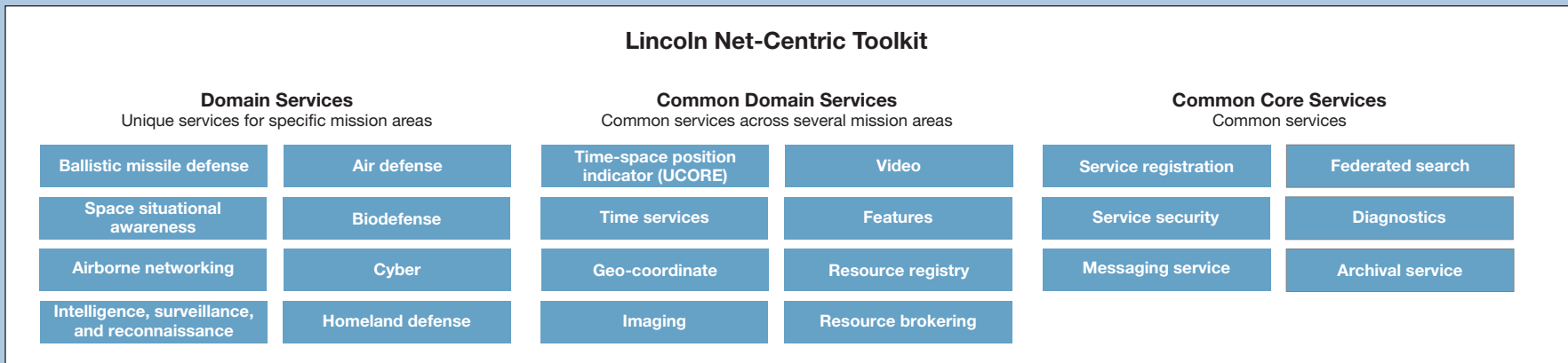
Figure 6-8 Lincoln Net-Centric Toolkit.
