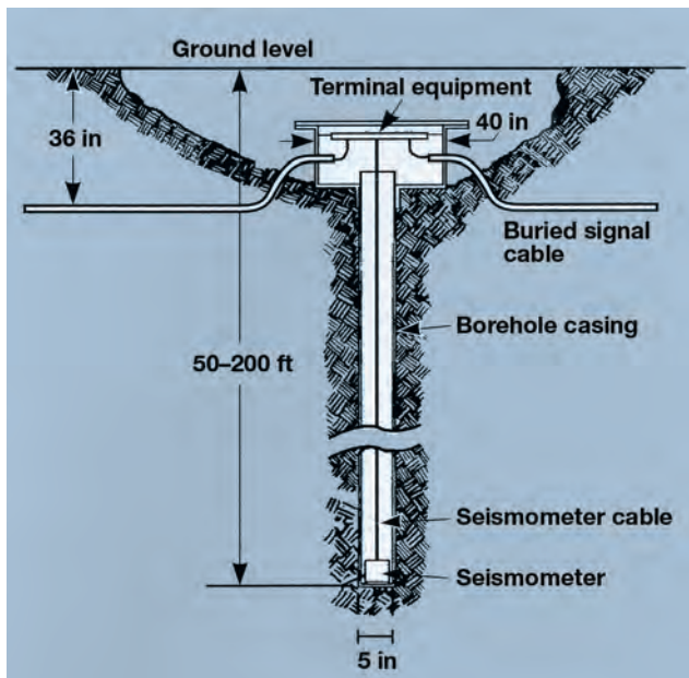
Figure 21-1 LASA seismometer installation.
