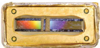
Figure 9-10 SAW filter. Note the faint white curves (left) that visibly indicate the finite-impulse-response filter coefficients. These coefficients implement a very narrow bandpass filter.
