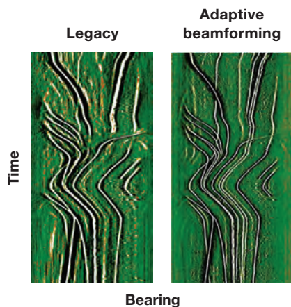
Figure 29-14 Sphere-array performance comparison.
