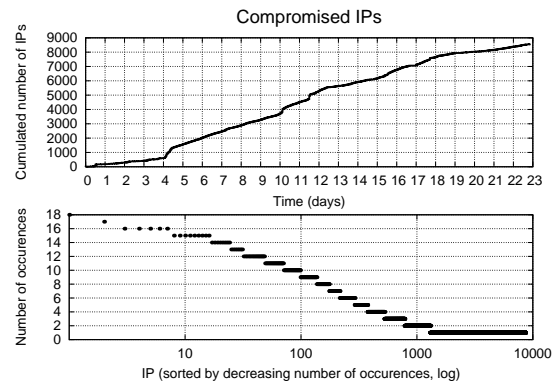
Figure 5: Number of unique IPs that we de-anonymized in time (top) and number of occurrences of a de-anonymized IP with at least one day of interval (bottom). We compromised IPs uniformly in time. Whereas we de-anonymized most IPs once, a few IPs were de-anonymized many times.
