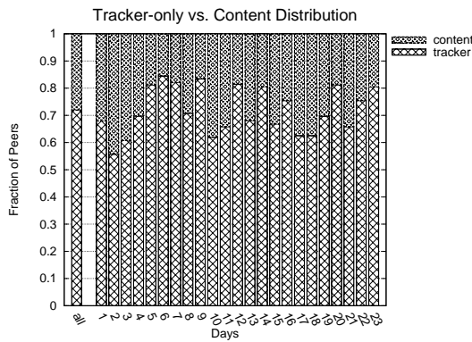
Figure 4: For each day, this histogram shows the proportion of peers who use Tor for content distribution (content) or only to connect to the tracker (tracker). all is the average over all days. 72% of peers use Tor only to connect to the tracker.
