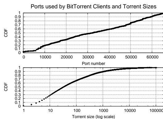
Figure 2: Distribution of the listening ports used by the BitTorrent clients that we have de-anonymized on 6 monitored exit nodes during 23 days (top). Distribution of the torrent sizes in which peers using those exit nodes were participating in during the same period (bottom). Because the port numbers are uniformly distributed and most torrents are small, the port number is a good peer identifier.
