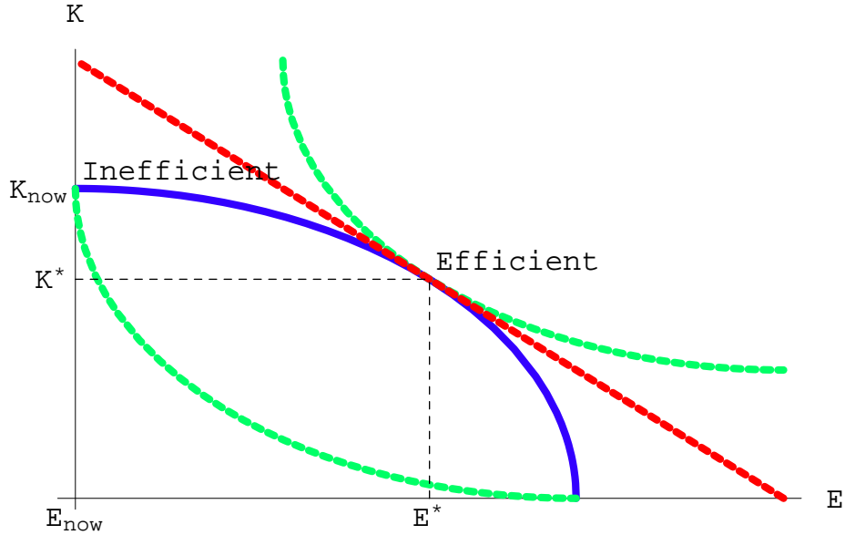
Figure 1: The heavy (blue) line represents combinations of E and K compatible with the present level of consumption of the current generation. Without mitigation of global warming the current generation will bequeath effectively zero climatological capital to future generations represented by the point (E_{now}, K_{now}) . The lower dotted (green) curve shows the combinations of E and K that would allow future generations to achieve the same level of consumption. Because the marginal cost of mitigation at the original point is zero, but the marginal benefit of mitigation for future generations is positive, the current allocation is inefficient. It would be possible without reducing the consumption of the current generation to move to (or closer to) the efficient allocation of investment, (E^*, K^*) , at which future generations could enjoy a higher level of consumption, represented by the upper dotted (green) curve showing the combinations of E and K that would allow future generations to achieve a higher level of consumption. At the efficient point the marginal cost and benefit of mitigation in terms of conventional investment are equal. The straight dotted (red) line represents the price of mitigation in terms of conventional capital at the efficient allocation.
