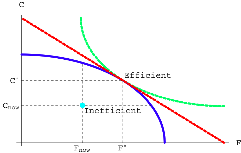
Figure 2: The heavy (blue) line represents combinations of F and C compatible with the technological tradeoffs between consumption of current and future generations, taking account of both conventional and environmental investments. Without mitigation of global warming the point representing the consumption of future and current generations is inside this frontier, (F_{now}, C_{now}) . Correction of the global-warming externality would move the world to (or closer to) the efficiency frontier. One possible efficient allocation is shown as (F^*, C^*) , where the efficiency frontier is tangent to the particular social indifference curve between consumption of current and future generations represented by the dotted (green) curve. The exact division of the benefit of correcting the externality between future and current generations will depend on the marginal valuation current generations put on the consumption of future generations, represented by the slope of the dotted (red) line tangent to the efficiency frontier.
