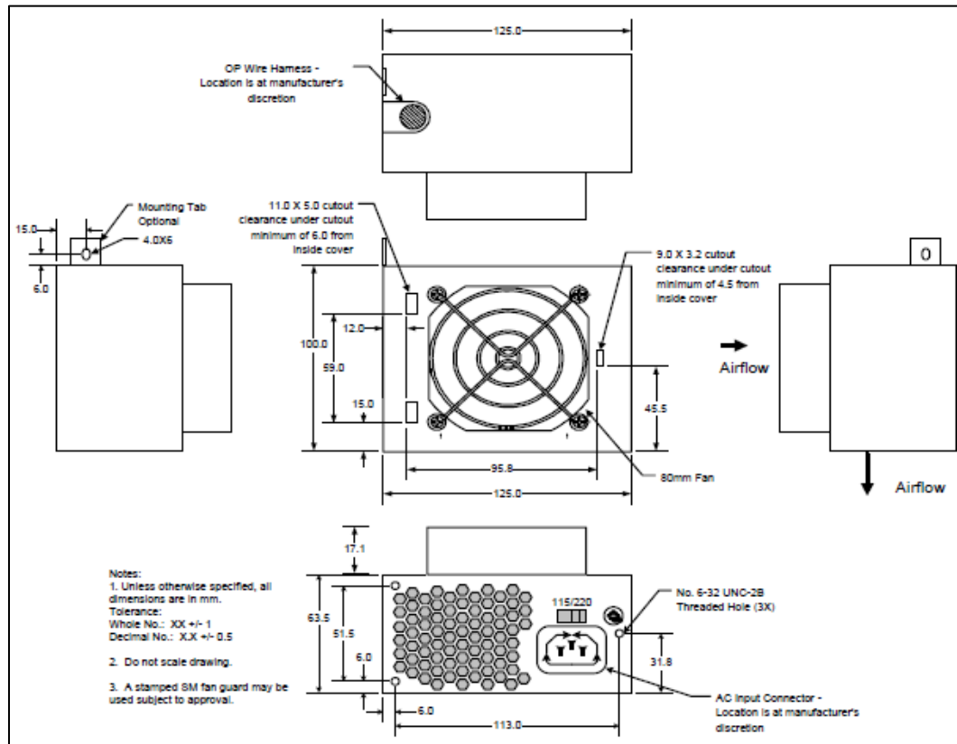
Figure 20 Chassis Cutout
