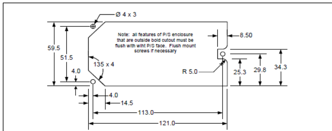
Figure 20 Chassis Cutout
