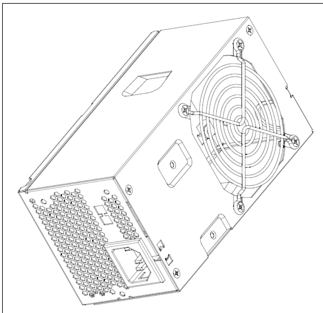
Figure 24 Mechanical Outline
