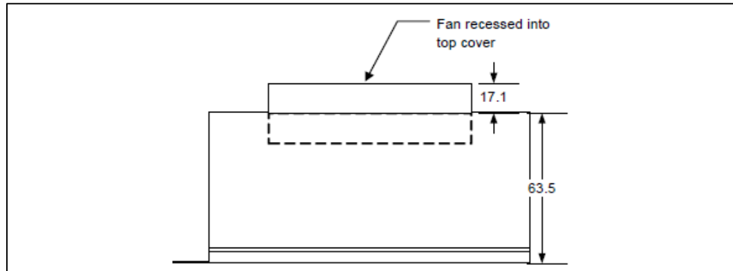
Figure 18 Recessed Fan Mounting
