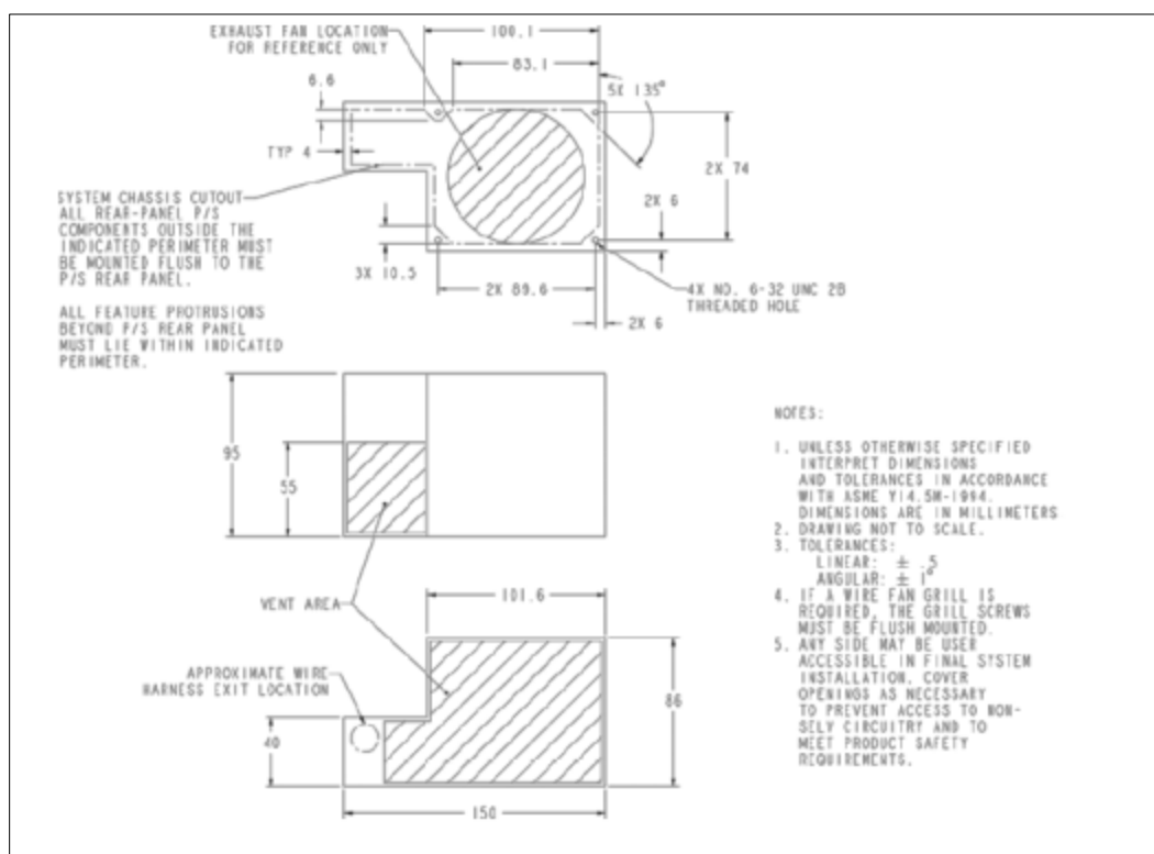
Figure 7 CFX12V Mechanical Outline
