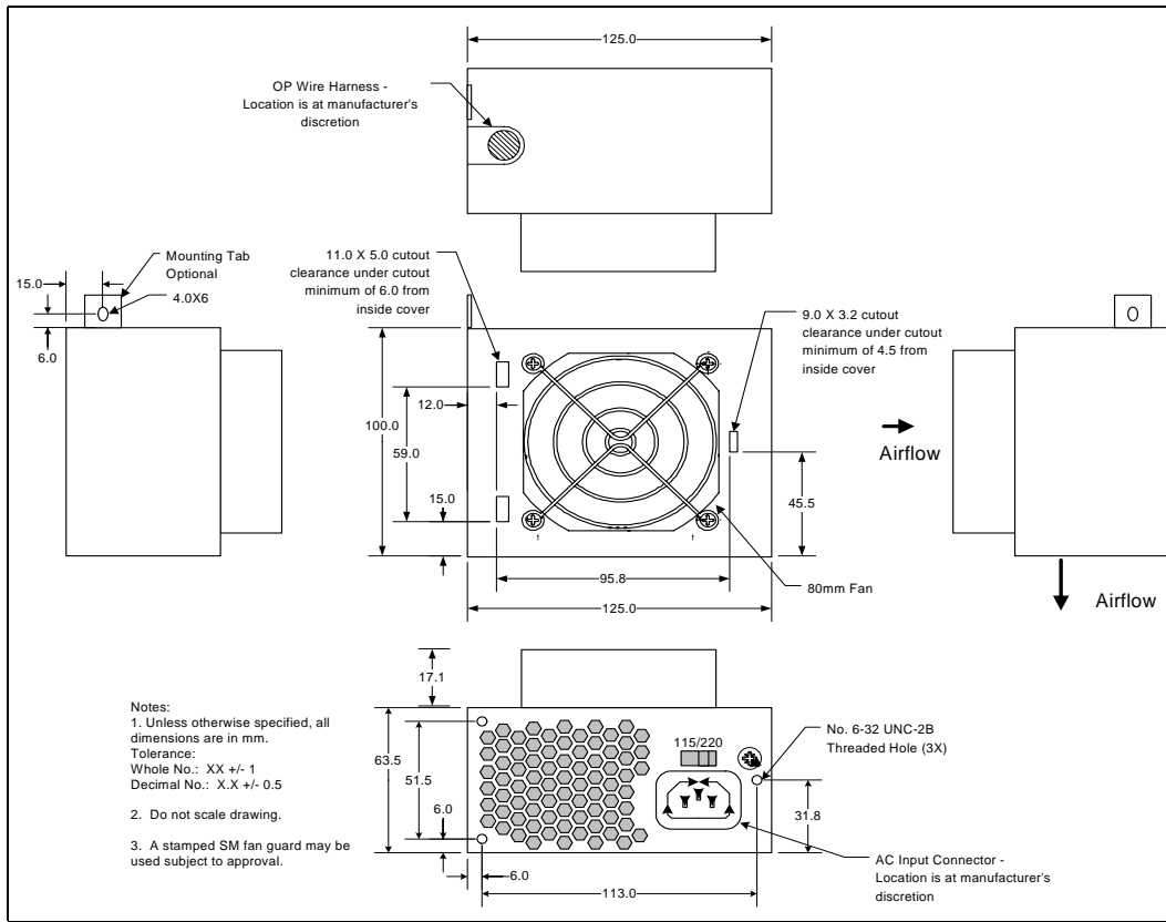
Figure 40. Chassis Cutout
