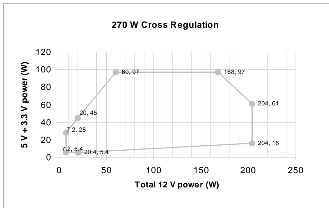
Figure 11. Cross Loading Graph for 270 W Configurations
