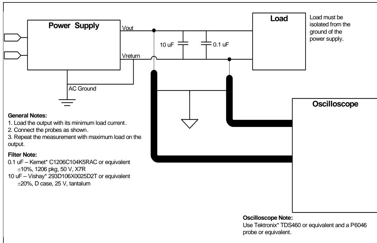
Figure 1. Differential Noise Test Setup
