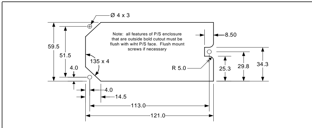
Figure 40. Chassis Cutout
