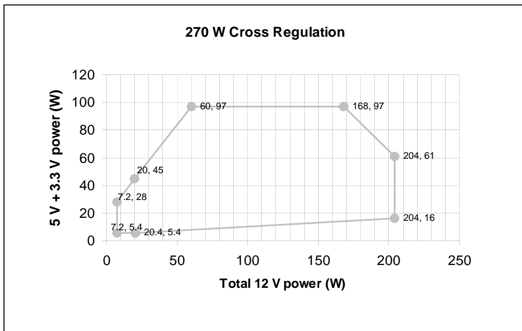
Figure 16. Cross Loading Graph for 270 W Configurations
