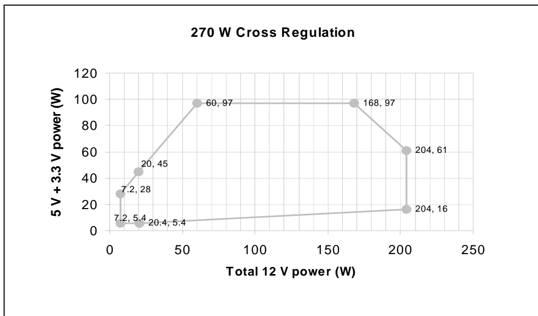
Figure 32. Cross Loading Graph for 270 W Configuration
