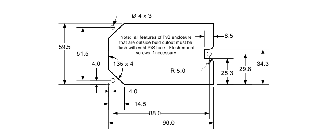
Figure 42. Chassis Cutout
