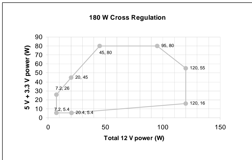
Figure 14. Cross Loading Graph for 180 W Configurations
