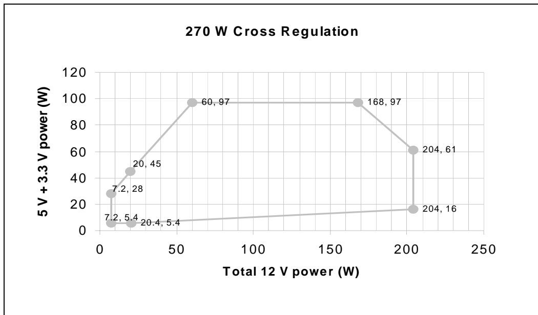
Figure 23. Cross Loading Graph for 270 W Configurations
