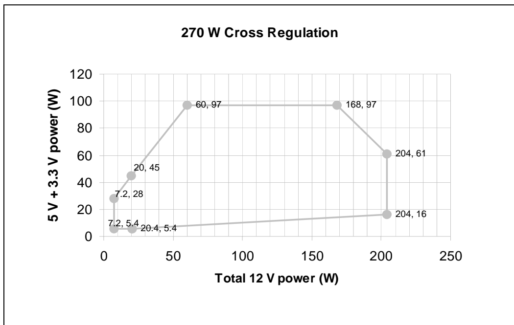
Figure 56. Cross Loading Graph for 270 W Configuration
