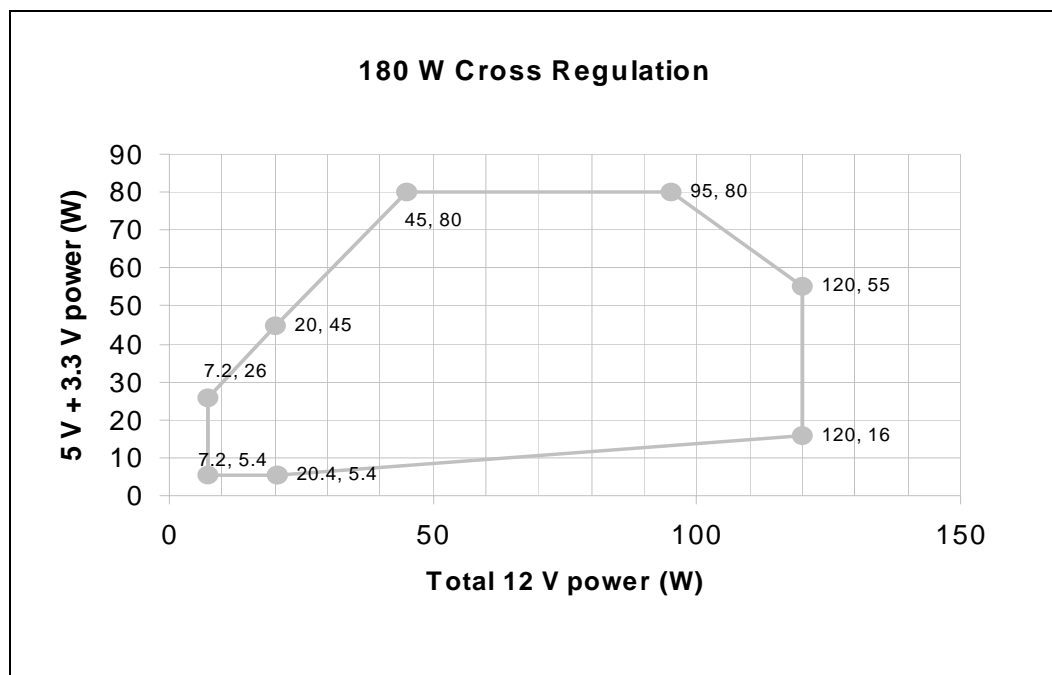
Figure 30. Cross Loading Graph for 180 W Configurations
