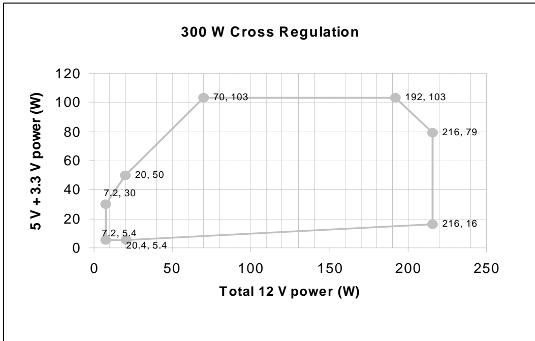
Figure 12. Cross Loading Graph for 300 W Configurations
