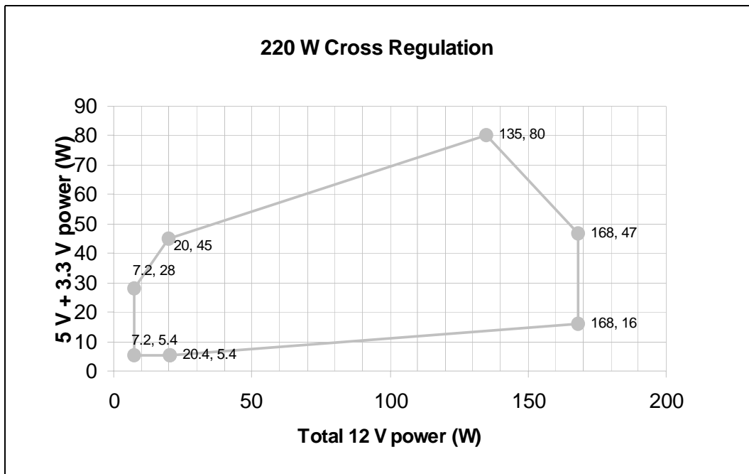
Figure 10. Cross Loading Graph for 220 W Configurations
