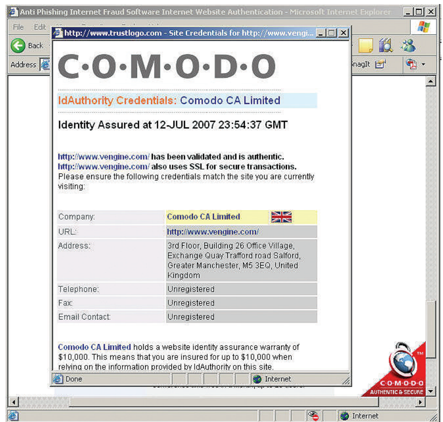
Figure 5: Comodo's IdAuthority™ JavaScript-based website validation response.
