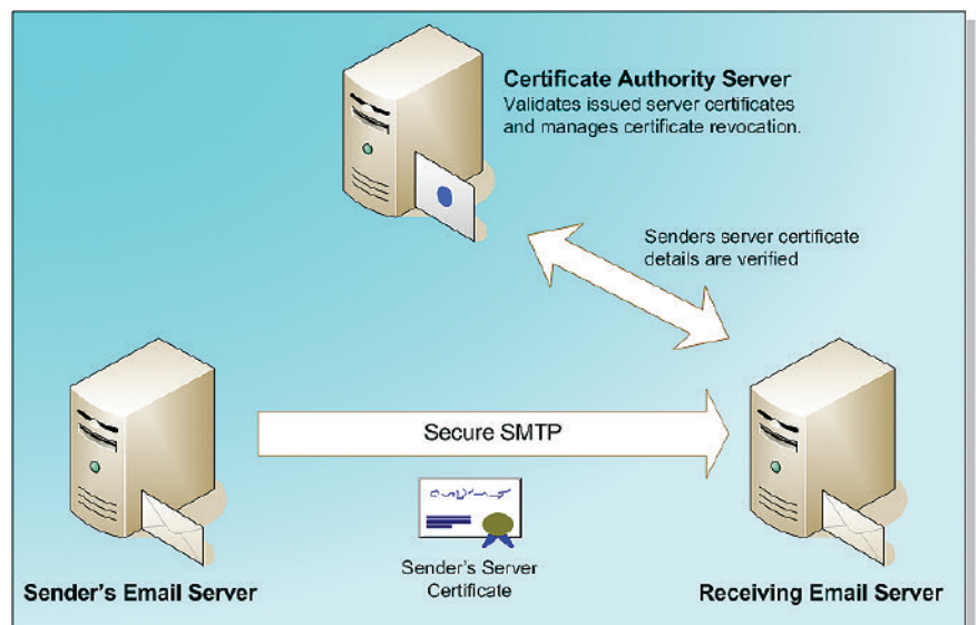
Figure 20: Mail server authentication – server certificates
