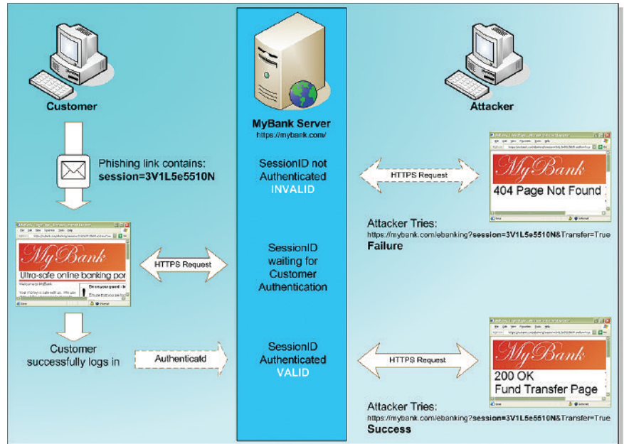
Figure 12: Preset session attacks
