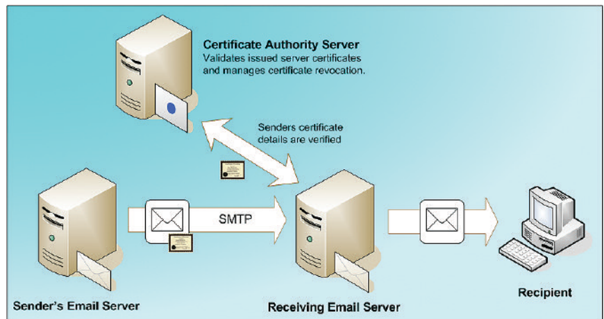
Figure 21: Digitally signed e-mail – receiving mail server validation of authenticity
