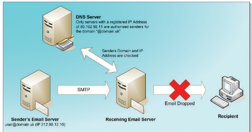
Figure 19: Mail server authentication – DNS querying of MX records
