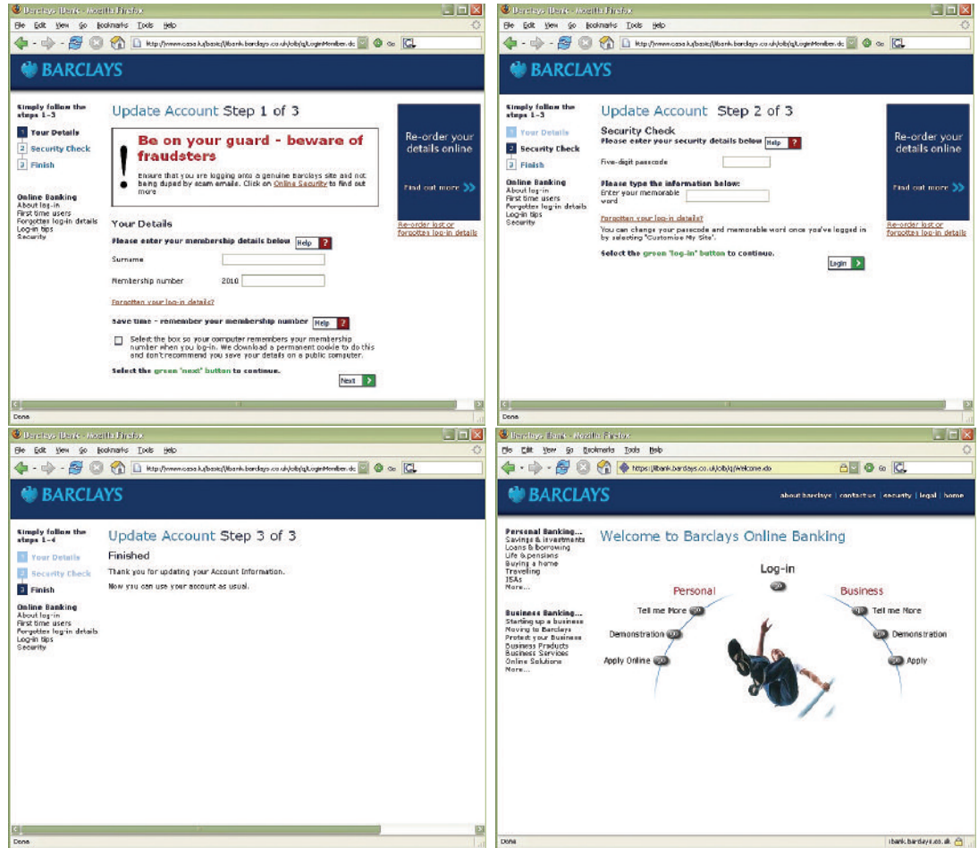
Figure 7: The website used by the phisher to steal authentication credentials from the victims
