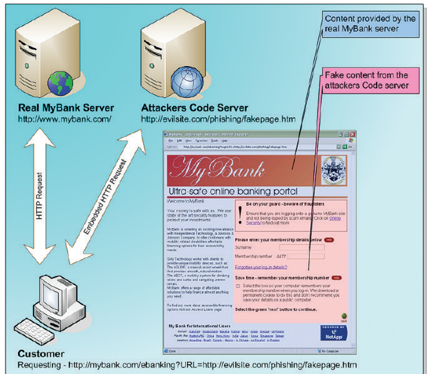
Figure 11: Cross-site scripting attacks
