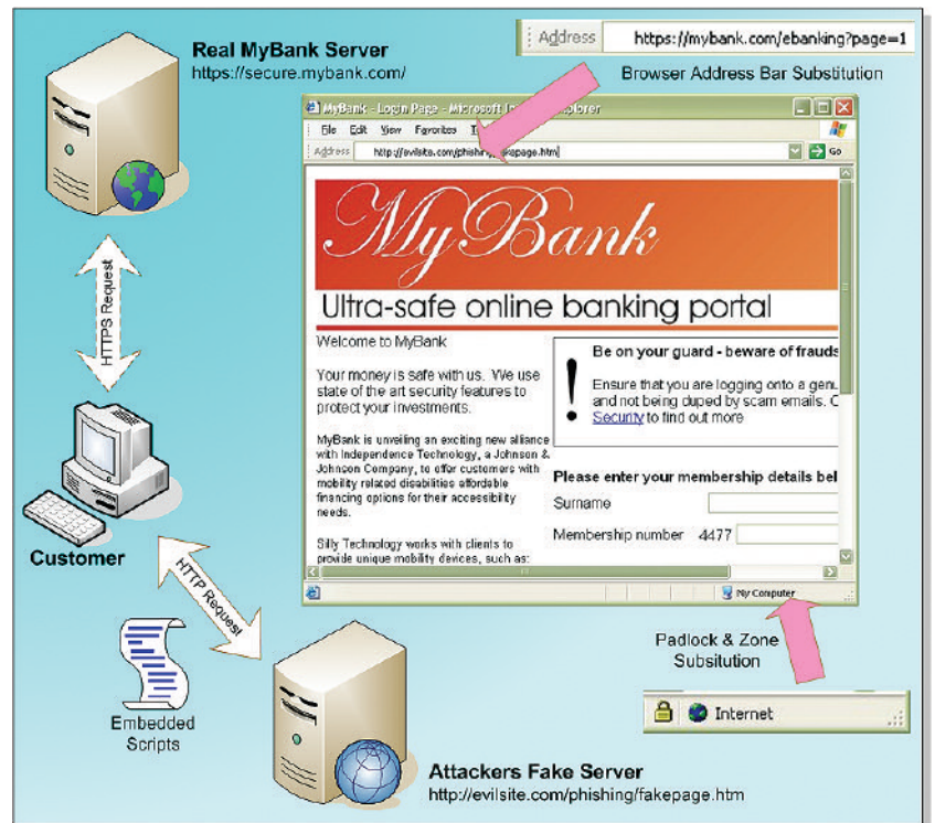
Figure 13: Site impersonation with browser address bar, secure padlock and zone substitution
