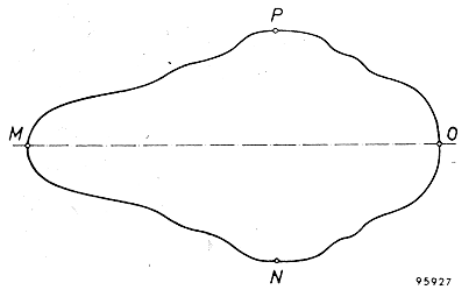
4. The resistivity measurement is simplified if the sample has a line of symmetry. If two of the contacts are situated on the line of symmetry and the two others are symmetrically disposed with respect to this line, one measurement is sufficient to give the required resistivity.
