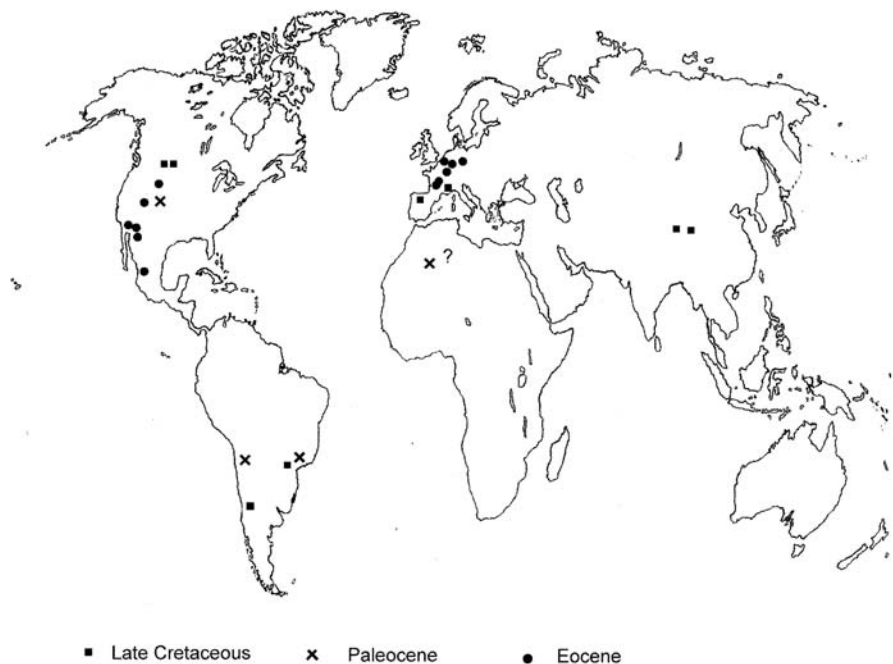
Fig.8- Distribution of fossil iguanid lizards.
